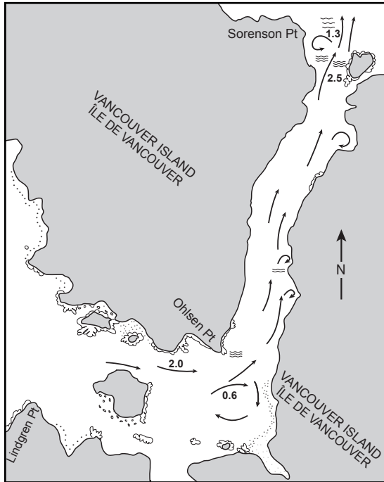
Figure 7.1 Quatsino Narrows Currents
