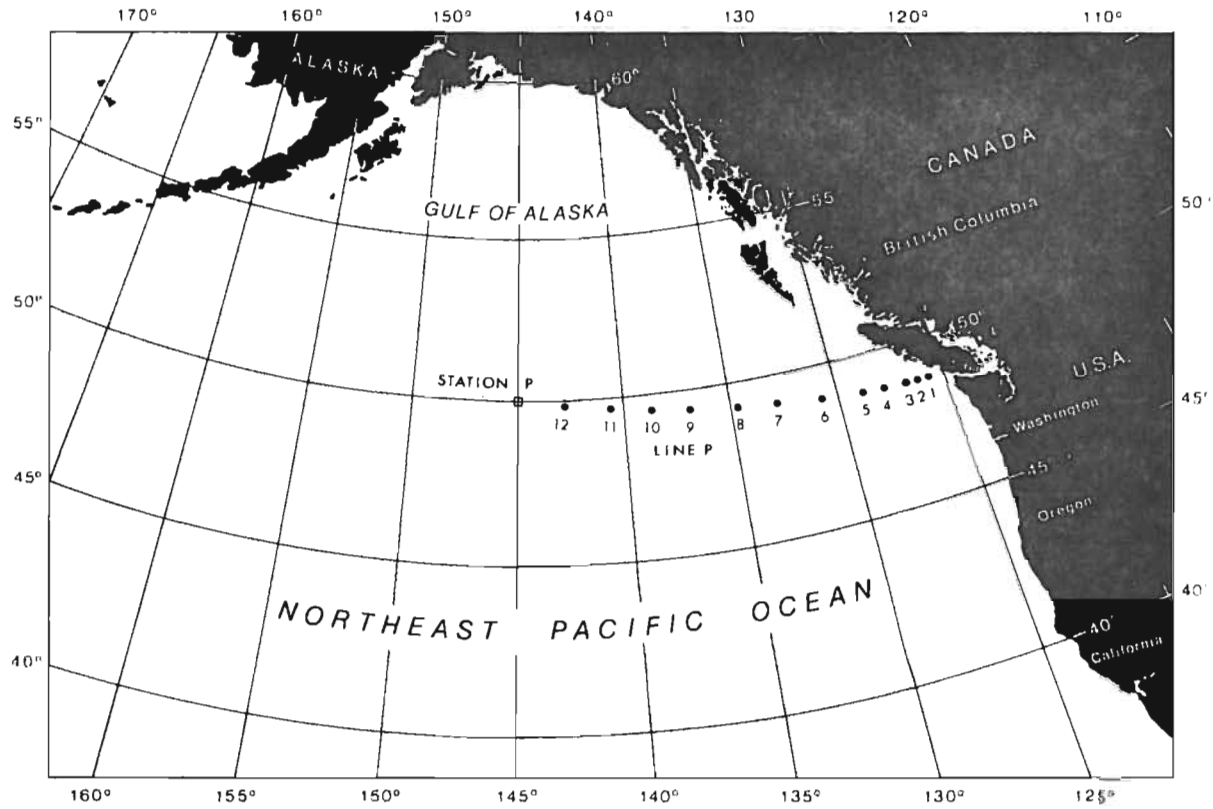
Figure 1. Location of Ocean Station P and Line P in the northeast Pacific Ocean.
