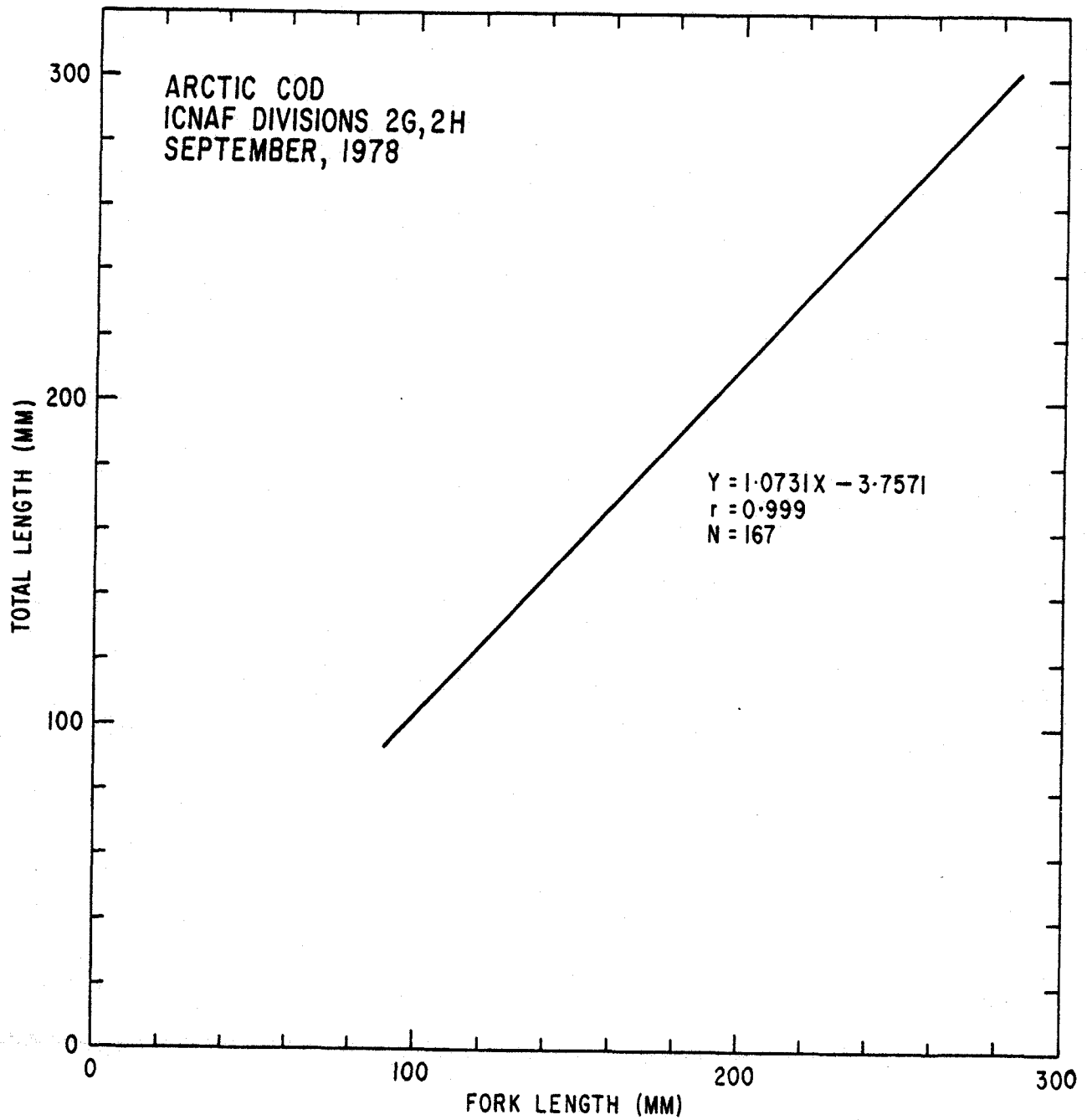
Figure 1. Weighted least squares regression of total length (mm) versus fork length (mm) for Arctic Cod.
