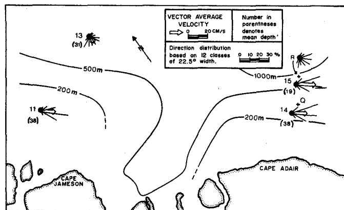
FIG. 30. The directional distribution of currents at nominal depths of 35 m off the east coast of Baffin Island. Stations 11, 13, 14 and 15 were operated in August and September 1978. Stations R and Q were operated in August and September 1979. (No distribution is shown for station Q because no 35 m record was recovered there).
