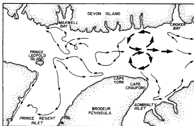
FIG. 25. A schematic presentation of drifter motion during summer 1979 in western and central Lancaster Sound. Representative individual tracks are indicated by thin arrows and patterns suggested by two or more drifters are shown as heavy arrows.
