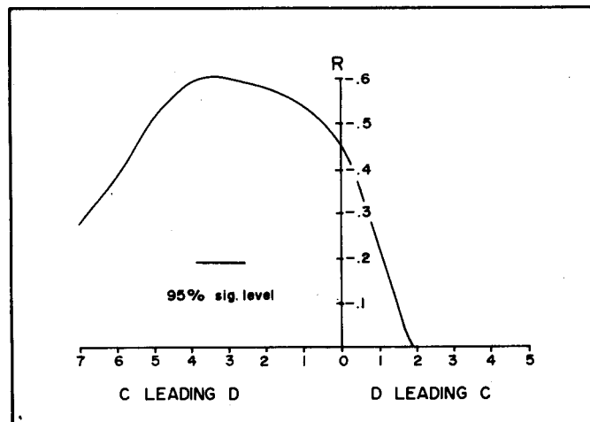
FIG. 12. Cross-correlation coefficient ( R ) versus time lag in days for northerly velocity components measured at stations C and D, 35 m depth. (Locations shown in Figure 10.)
