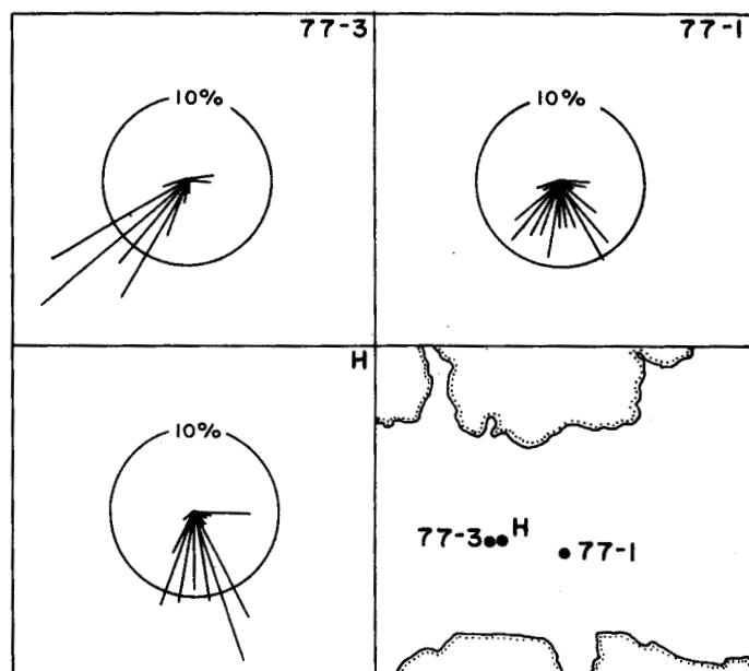
FIG. 18. Direction distributions of currents at 35 m which exceeded 48 cm/s at stations 77-1, 77-3 and H, in eastern Lancaster Sound.
