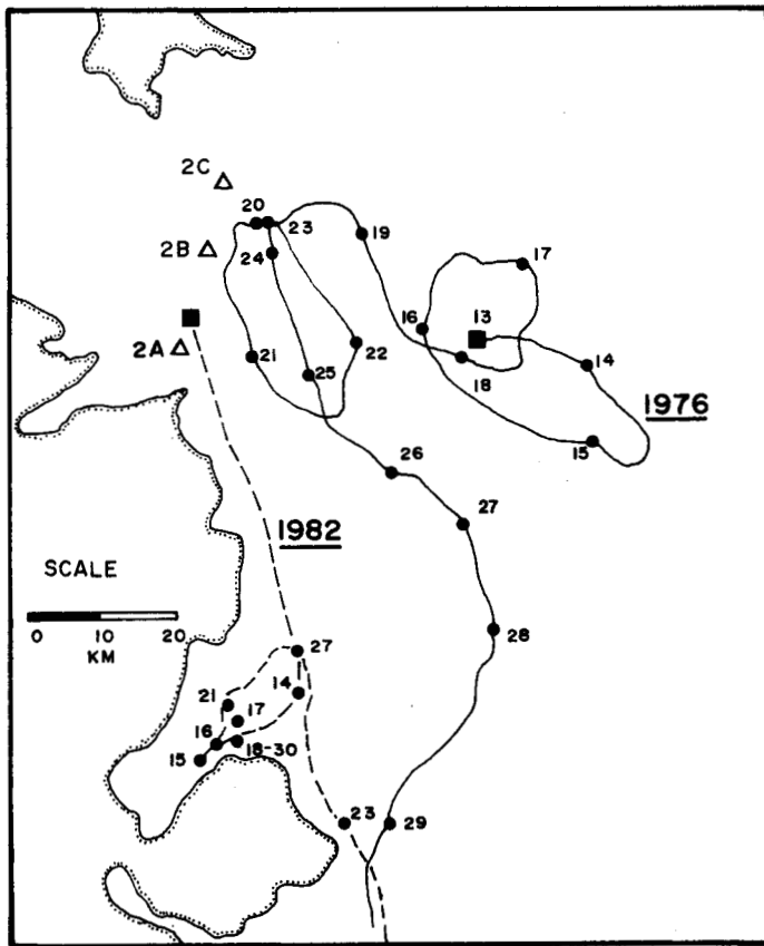
FIG. 8. Tracks of two drifters, 1976 and 1982, moving in the approaches to Lady Ann Strait east of Devon Island during August 1979. The triangles mark the locations of CTD stations in Lady Ann Strait. The squares indicate the release points of the drifters, and the dots show the first reported position on the day whose date appears beside it. One of the tracks is shown as a dashed line for clarity.
