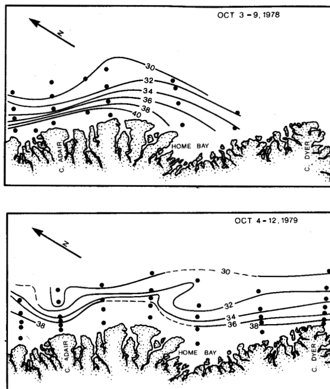
FIG. 29. Dynamic topography (in dynamic cm) of the surface relative to 300 dbar from CTD data collected in 1978 and 1979 off the east coast of Baffin Island. The dots mark the station locations. The indicated surface flow is parallel to the contour lines, with greater dynamic heights to the right of the flow. Current speed is inversely proportional to the spacing between the contours.
