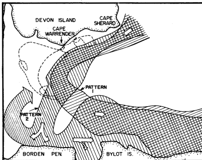
FIG. 13. Envelopes containing drifter tracks obtained in 1979 in eastern Lancaster Sound, divided according to two patterns. Shown separately as dashed lines are the tracks of four drifters which departed from the major flow patterns.
