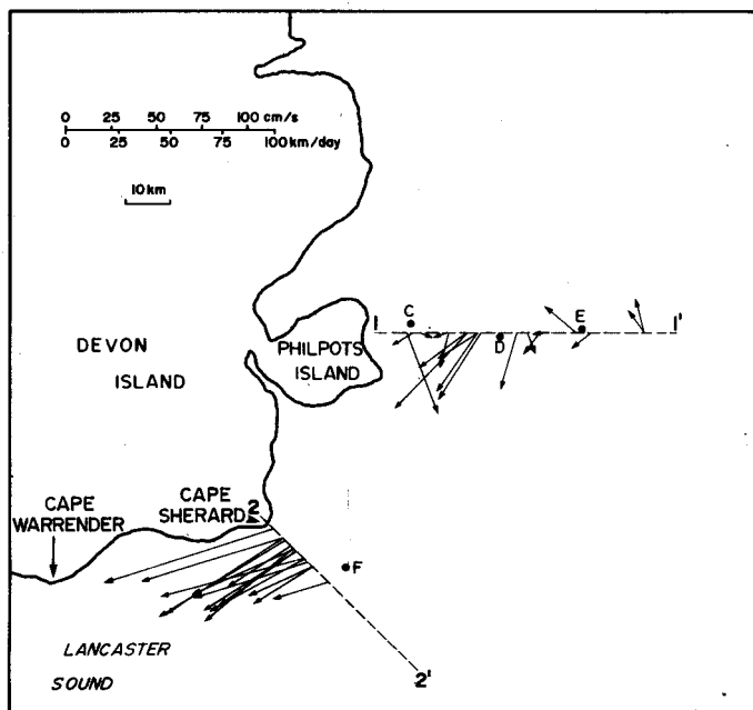
FIG. 10. Velocities of near-surface currents measured by satellite-tracked drifters crossing two sections off Devon Island in 1979. Letters indicate current meter mooring locations.
