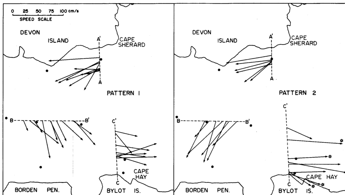
FIG. 15. Near-surface current velocities measured by satellite-tracked drifters through three cross-sections of the intrusive current. The velocities are presented separately for each pattern of the current. The symbol (*) represents velocities of drifters deployed in western and central Lancaster Sound. The dots mark the locations of current meter moorings.
