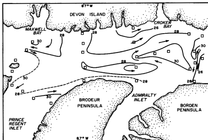
FIG. 24. Dynamic topography (in dynamic cm) of the surface relative to 175 dbar for the period 24 Aug. - 6 Sept. 1979 in western Lancaster Sound. The squares mark the station locations and the numbers give the dynamic height anomaly associated with each contour line. The arrows indicate the direction of surface baroclinic flow. Current speed is inversely proportional to the spacing between the contours.
