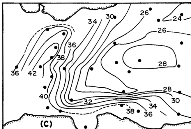
FIG. 14. Surface dynamic height anomalies (in dynamic cm) relative to 300 dbar level for four periods of CTD observations in 1979: (A) July 18-19 (B) July 29-Aug. 3 (C) Sept. 2-4 and (D) Sept. 14-23 in eastern Lancaster Sound. (The dots mark the station locations). The indicated surface flow is parallel to the contour lines, with greater dynamic heights to the right of the flow. Current speed is inversely proportional to the spacing between the contours.
