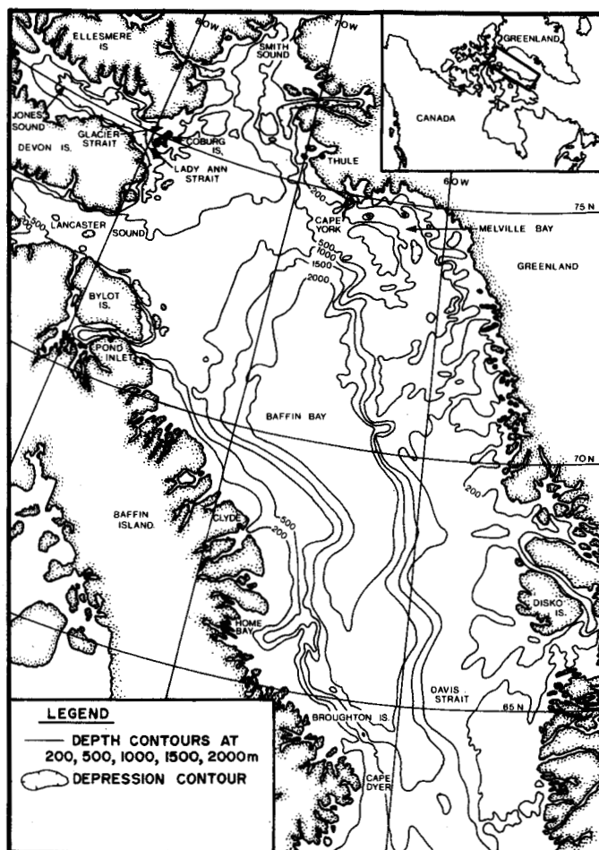
FIG. 1. Bathymetry of Baffin Bay and adjacent water bodies.
