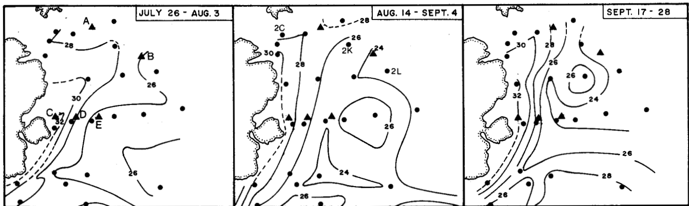
FIG. 9. The surface dynamic height anomaly east of Devon Island (in dynamic cm) relative to 300 dbar for three periods of CTD observations in the summer of 1979. The dots mark the CTD stations used to compile the chart. The triangles mark the locations of current meter moorings in the area. (Numbers and letters [e.g. 2L] beside dots, and letters beside triangles are station names). The indicated baroclinic surface flow is parallel to the contour lines, with greater dynamic heights to the right of the flow. The current speed is inversely proportional to the spacing between the contours.
