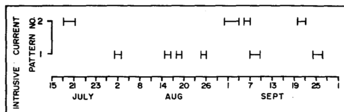
FIG. 20. Patterns of the intrusive current observed in 1979. The bars denote periods during which the current was observed unambiguously to follow pattern 1 or pattern 2. During the periods between the bars, there were insufficient data to determine the configuration of the flow.
