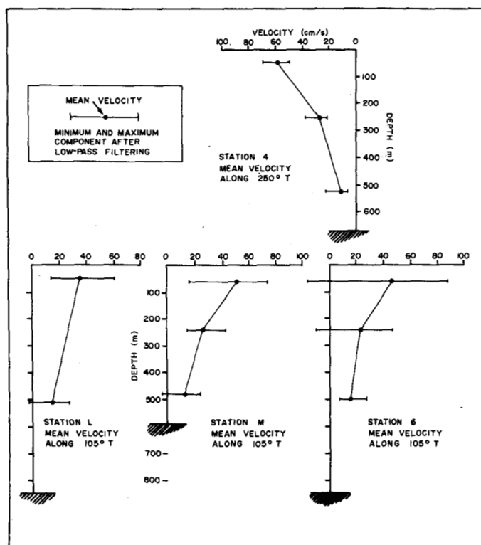
FIG. 21. Average vertical profiles of the intrusive current as measured at mooring stations 4, 6, L and M. The horizontal bars represent the extremes of the current after a low pass filter has been applied to remove daily and higher frequency variations.
