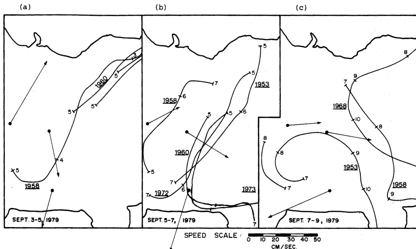
FIG. 19. Case studies in Lancaster Sound of simultaneous drifter and current meter velocities from 3-9 Sept. 1979, illustrating transition from pattern (2) to pattern (1) of intrusive current (see Fig. 13). The underlined numbers (e.g. 1958) are the drifter identity numbers. Each small bar across the drifter tracks denotes the first recorded position on the day whose date appears beside it. The arrows depict the direction and magnitude (measured according to the scale shown) of the daily vector-averaged 35 m current at each mooring in the area.
