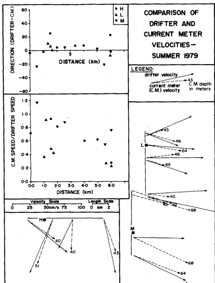
FIG. 16. A comparison of drifter and simultaneous uppermost current meter velocities for separations of 6 km or less at mooring stations H, L and M, located in eastern Lancaster Sound.
