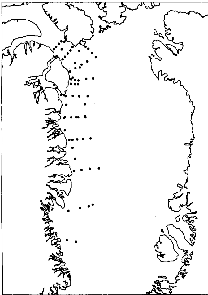
FIG. 4. Locations of CTD stations in 1978. The majority of the stations were occupied three times during the period from July to October, with the stations south of Bylot Island being occupied only once for the two most southerly lines and twice for the remainder.
