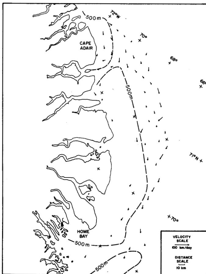
FIG. 28. Average velocities from drifter data obtained in 1979 off the east coast of Baffin Island. Each arrow represents the vector-averaged velocity of all the drifters which passed through the grid square, centered at the base of the arrow. The grid elements have dimensions of 0.5^\circ longitude and 0.167^\circ latitude. Only arrows representing three or more averages are included.
