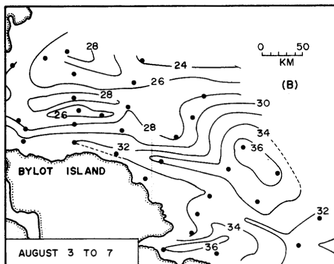
FIG. 26. Dynamic topography (in dynamic cm) of the surface relative to 300 dbar, for 4 periods in 1979. The dots mark station locations. The indicated surface flow is parallel to the contour lines, with greater dynamic heights to the right of the flow. Current speed is inversely proportional to the spacing between the contours.
