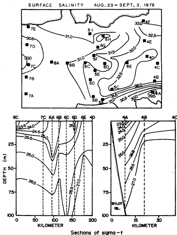
FIG. 22. Evidence of frontal structures in the intrusive current from CTD data from 23 Aug. - 3 Sept. 1979. The contour interval for surface salinities is 0.5‰. The squares mark the station locations.
