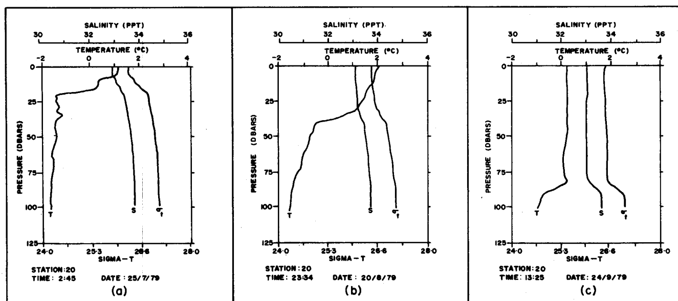
FIG. 7. Successive temperature, salinity and sigma-t profiles at offshore station 20 (30 km east of Devon Island), in 1979. (Pressure in dbars is approximately equal to depth in metres.)
