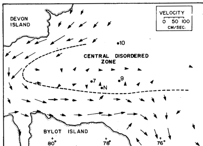
FIG. 23. The vector-averaged velocities for grid areas in the Central Disordered Zone from drifter data obtained in 1979. Each arrow represents the vector-averaged velocity of all the drifters which passed through a grid element with dimensions 0.5^\circ in longitude by 0.167^\circ in latitude, centered at the base of the arrow. N, 7, 9 and 10 are the locations of current meter moorings.
