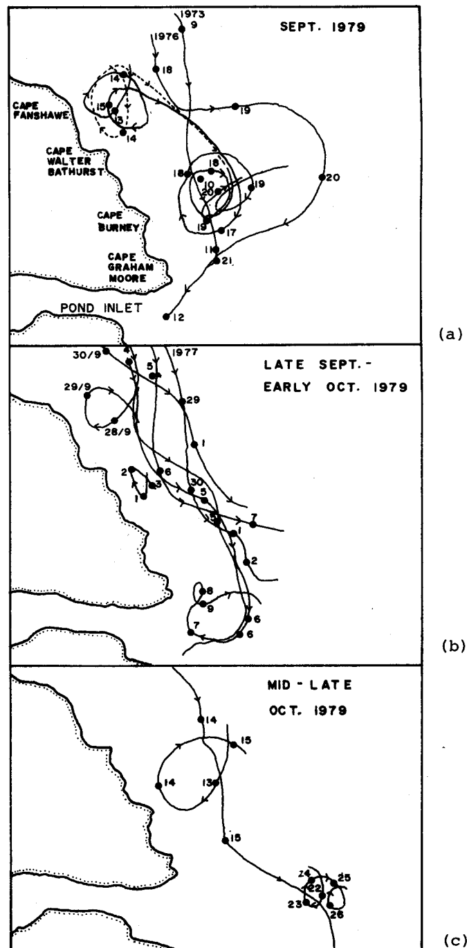
FIG. 27. Eddies detected in 1979 by drifter tracks east of Bylot Island: (a) Sept. 9-21 (b) Sept. 27-Oct. 9 and (c) Oct. 13-26. (One track in part (a) has been shown dashed for clarity). Each dot on the tracks denotes the first recorded position on the day whose date appears beside it.
