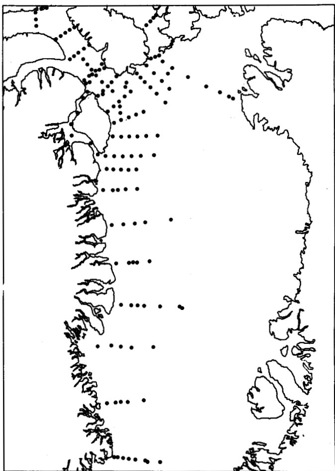
FIG. 5. Locations of CTD stations in 1979. Stations were occupied from July to October, with most of the stations in Lancaster Sound and its approaches being occupied four times. The remainder of the stations were taken either once or twice.
