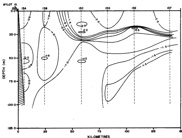
FIG. 6. Cross-section of temperature in the upper 100 m, for a line of stations running east of Bylot Island, 25-26 August 1979.
