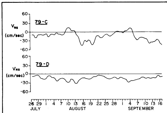
FIG. 11. Low pass filtered northerly component of velocity at 35 m depth, stations C and D. (Locations shown in Figure 10.)
