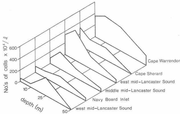
Figure 7.3 Phytoplankton Standing Crop (expressed as total cell counts) varied with depth and location in Lancaster Sound, July 22 to September 13, 1976 (from Sekerak et al, 1976b) 7.4 .
