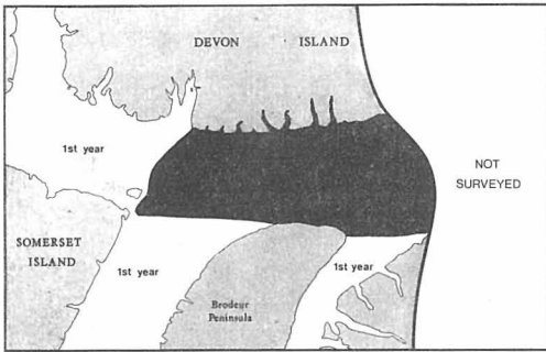
Figure 4.3 Springtime Ice Concentrations 1967 & 1968
