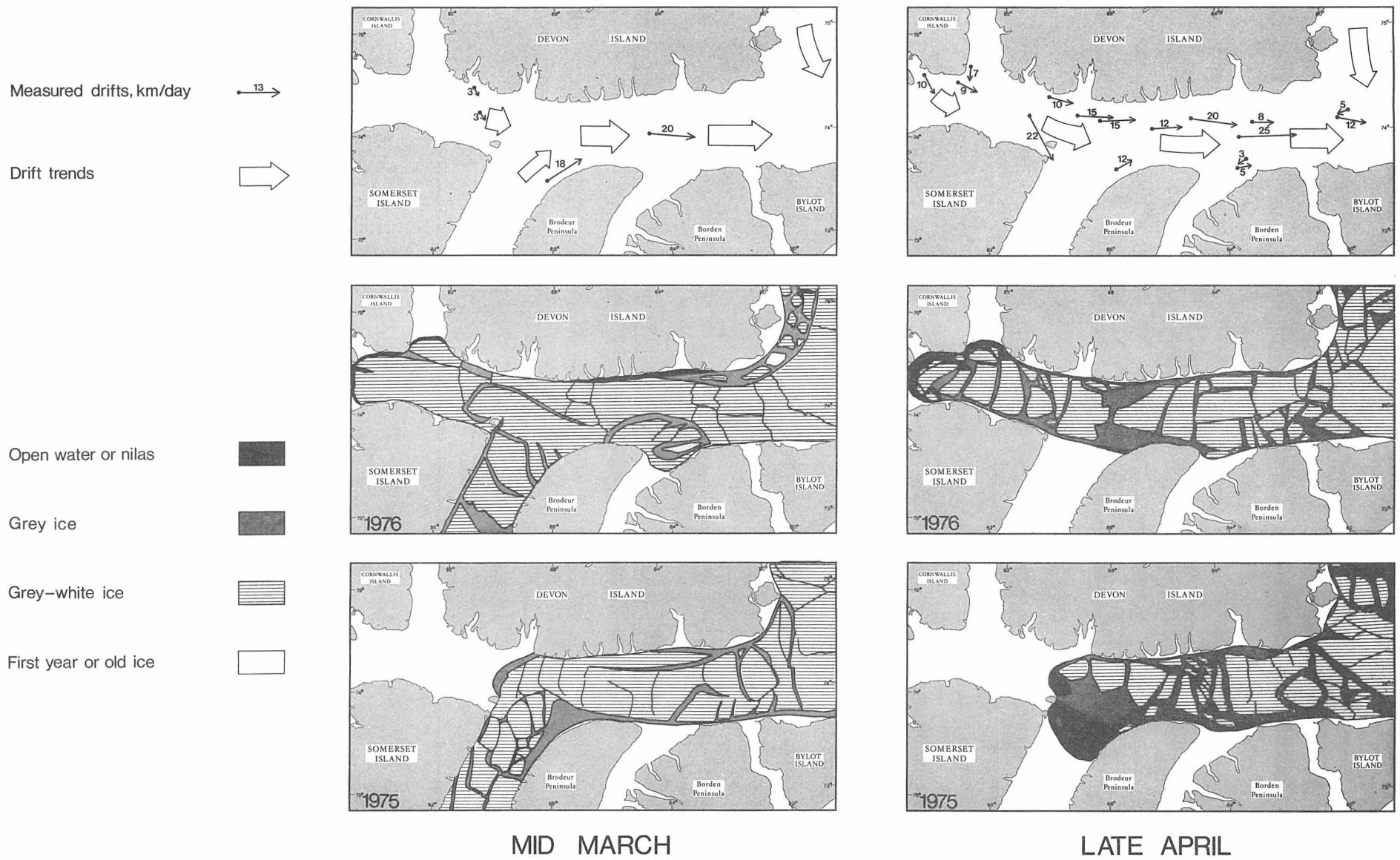
Figure 4.2 (cont'd) Ice freeze-up and breakup patterns, 1975 and 1976.
