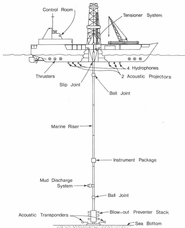
Figure 3.1 Deep-water Drilling System
