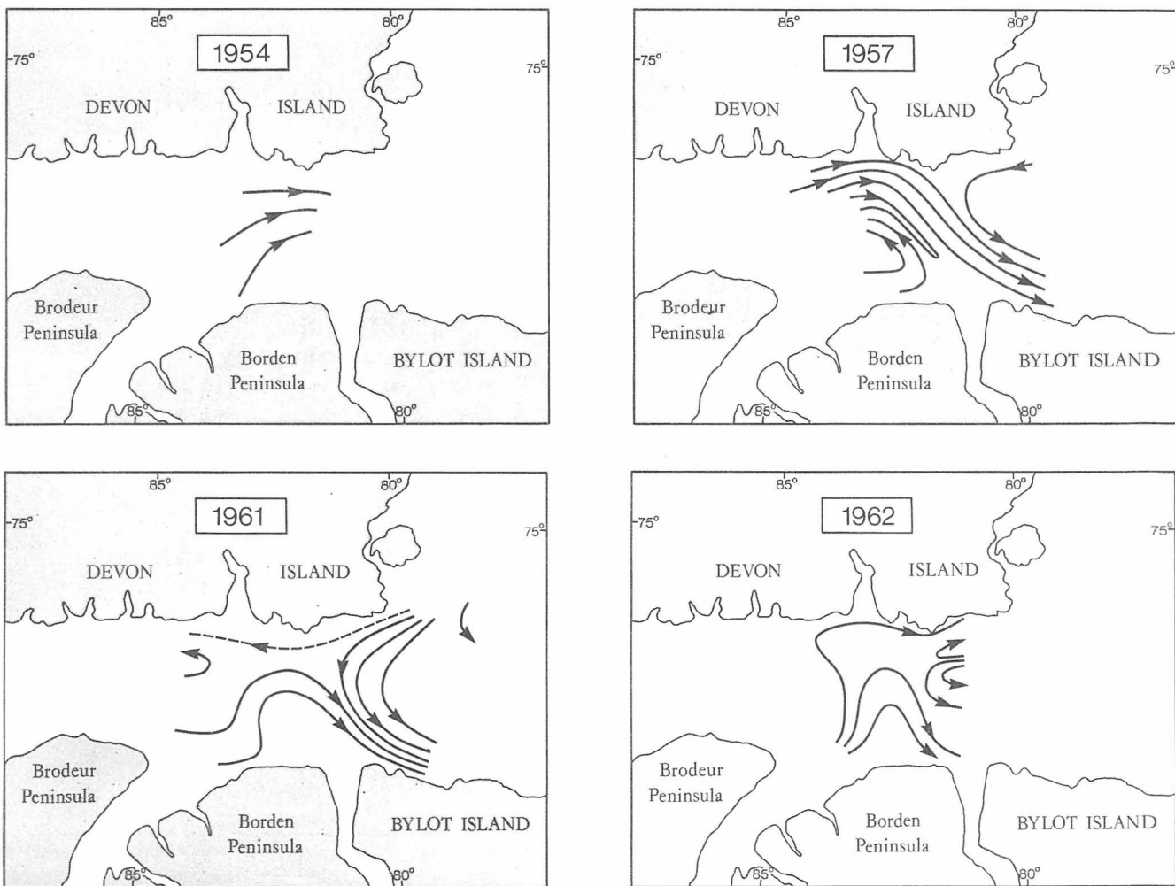
Figure 4.14 Surface current patterns calculated by Muench 4.16 for July - August 1954; September 1957, September 1961 and September 1962.
