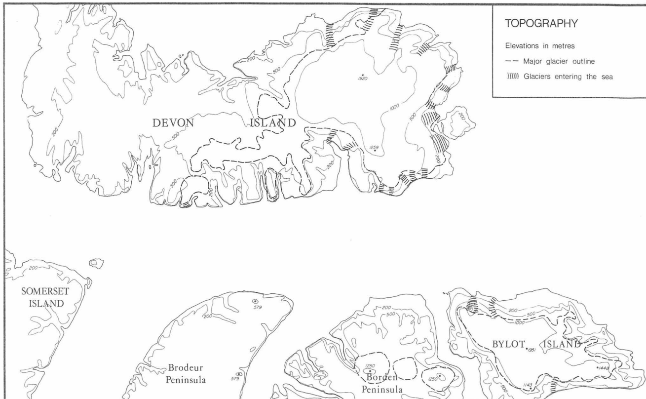
Figure 4.9 Land Topography, Lancaster Sound Region
