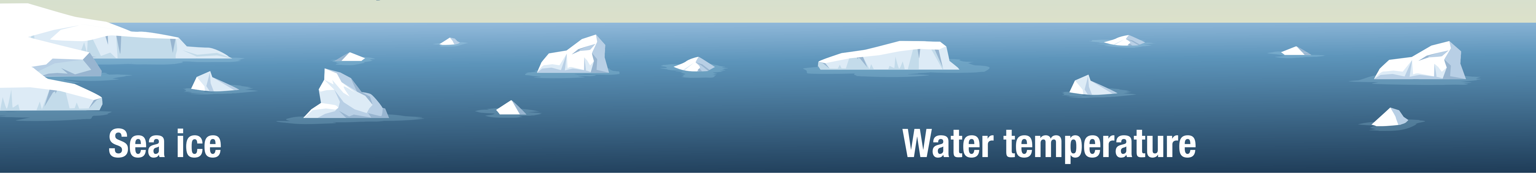
Newfoundland and Labrador Shelves sea ice index
