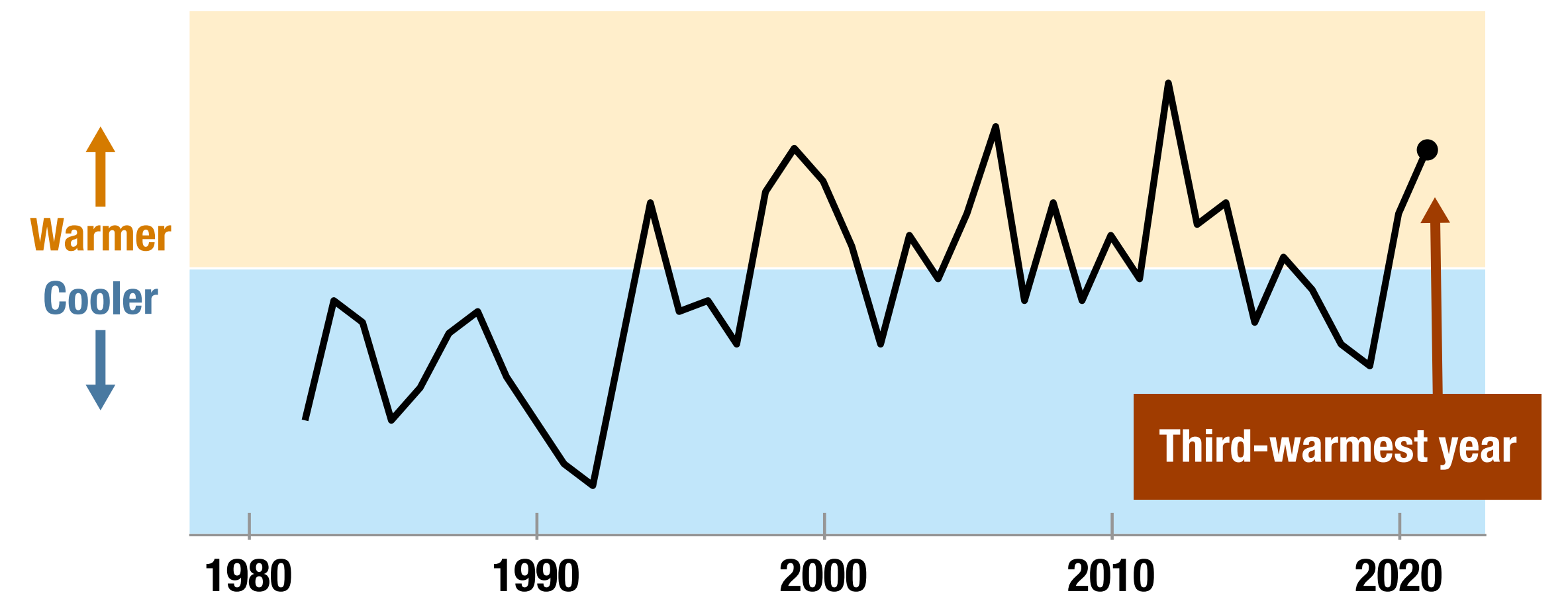
Sea-surface temperature index (Atlantic-wide)
