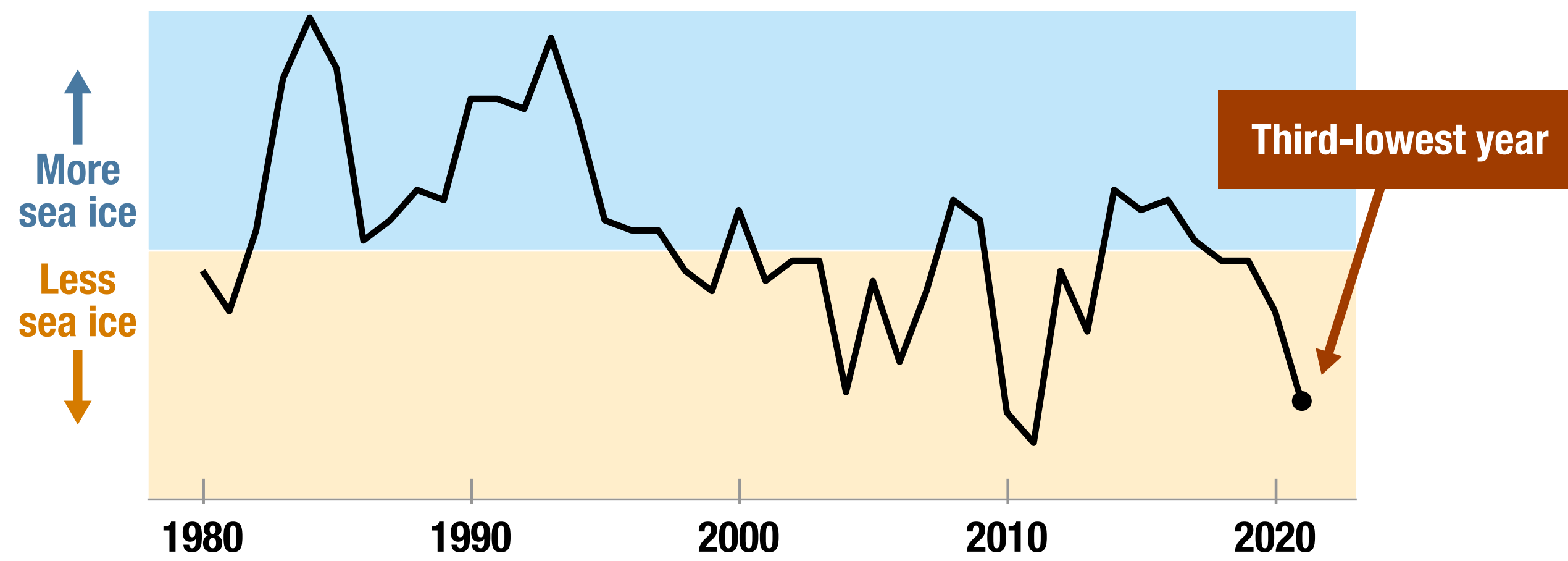
Newfoundland and Labrador Shelves sea ice index
