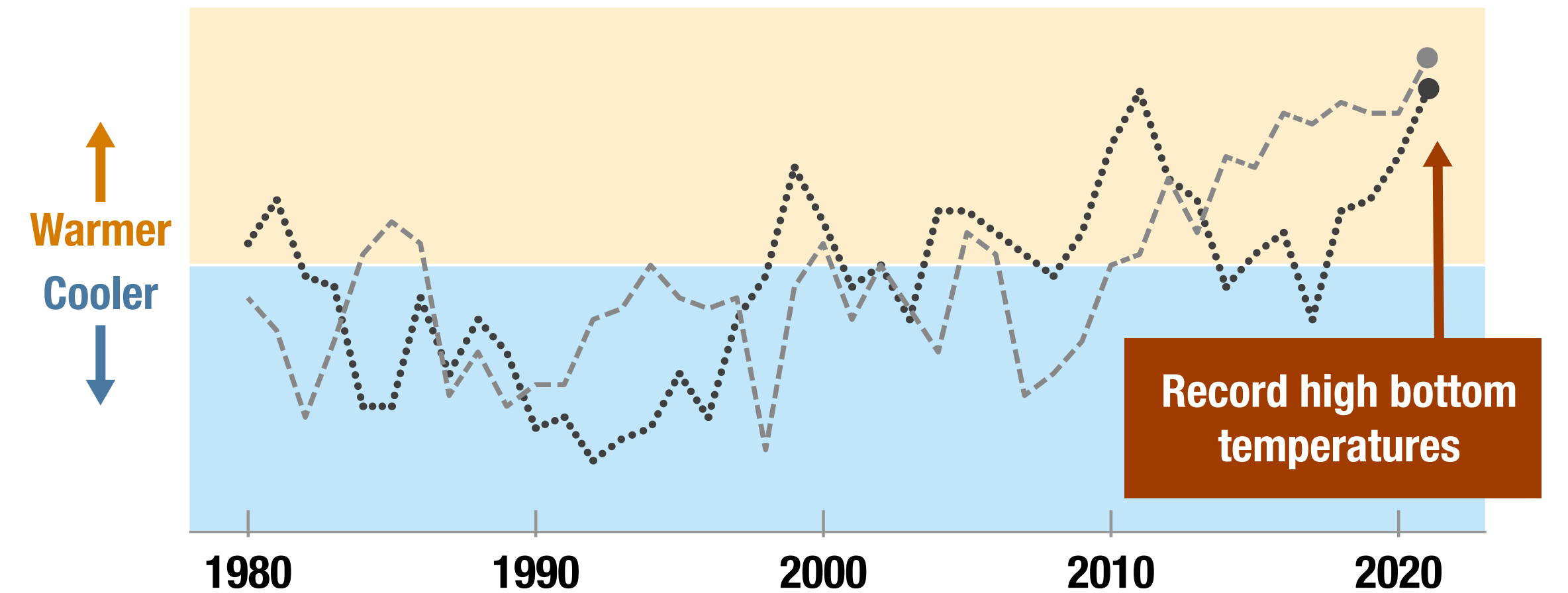
Bottom water temperature index (Atlantic-wide)
