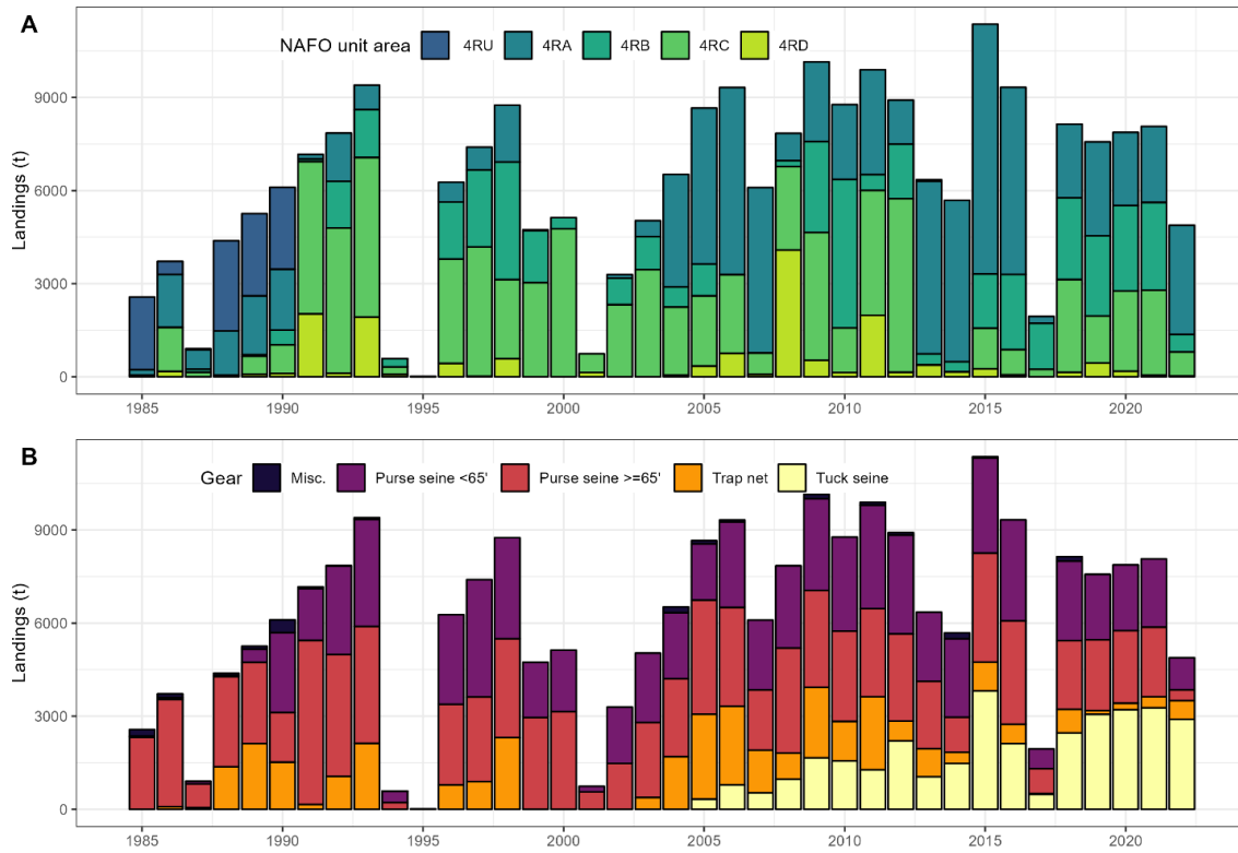
Figure 3. Annual commercial landings (t) of capelin in NAFO Div. 4R for the 1985–2022 period, by A) NAFO unit area (4RU = unknown 4R unit area) and B) main fishing gear type. Landings for 2020, 2021 and 2022 are preliminary.
