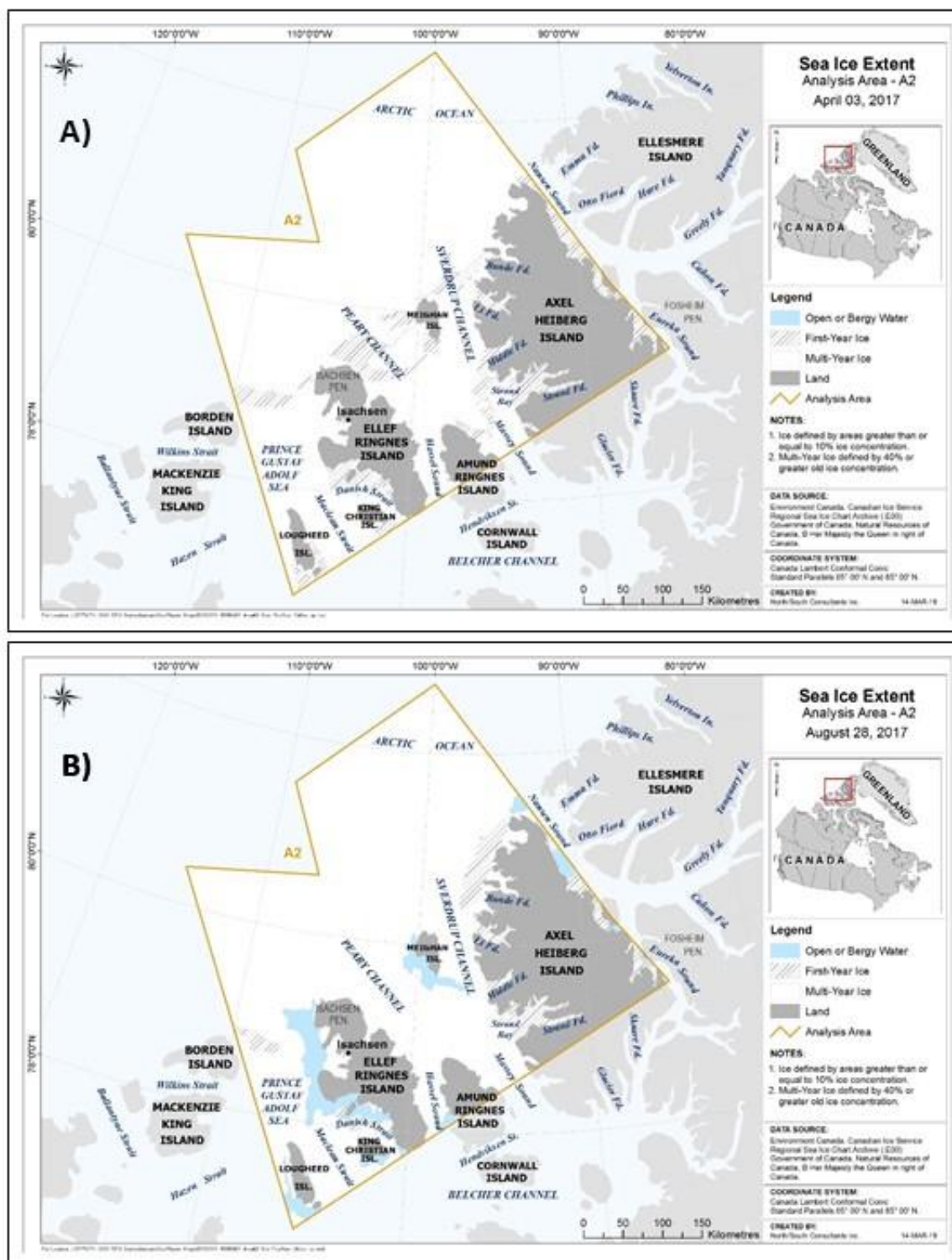
Figure 42. Extent of MYI, FYI and open water on maximum sea ice extent date (A) and minimum sea ice extent date (B) in 2017 within region A2.
