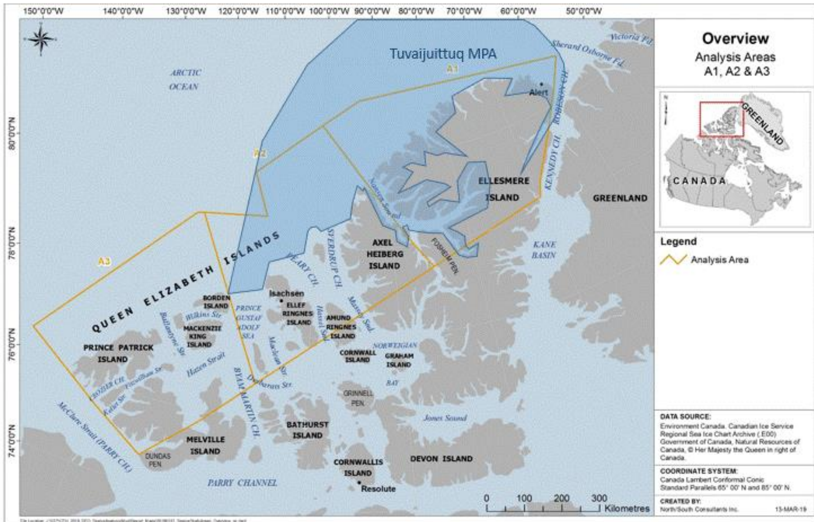
Figure 1. Geographic boundaries of analysis regions A1, A2, and A3, along with the portion of Tuvaivittuq MPA boundary located within the study region.
