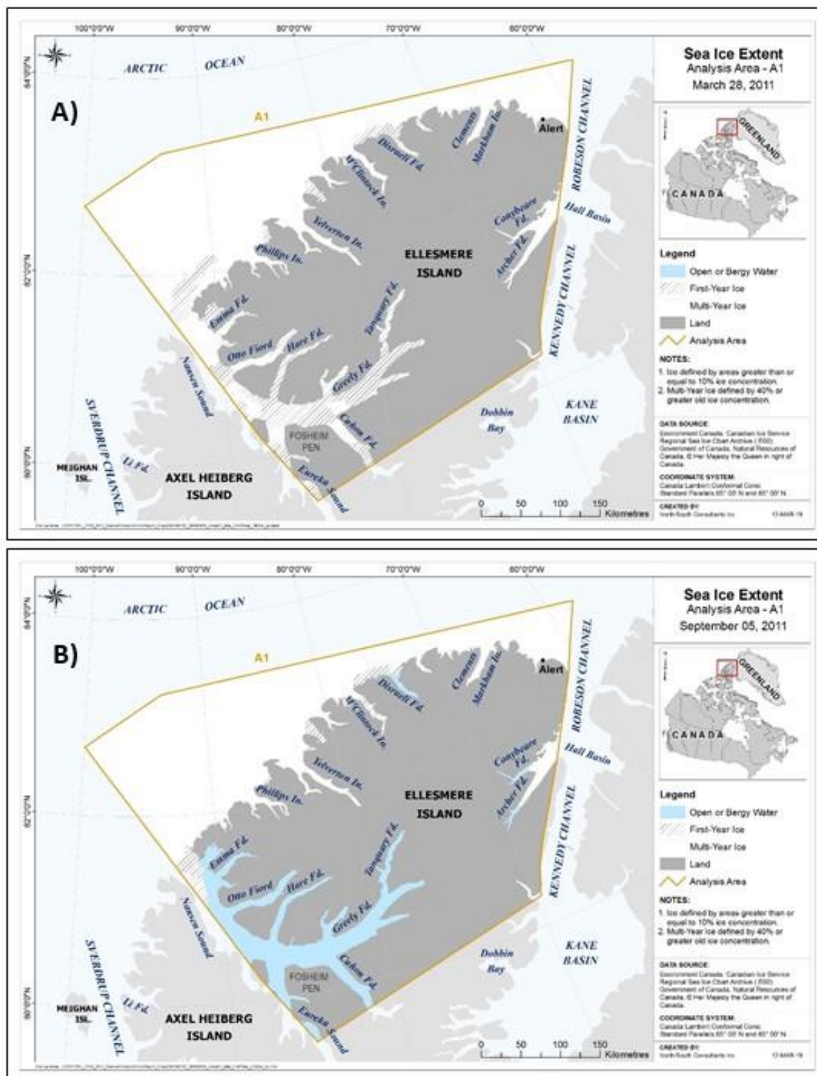
Figure 16. Extent of MYI, FYI and open water on maximum sea ice extent date (A) and minimum sea ice extent date (B) in 2011 within region A1.
