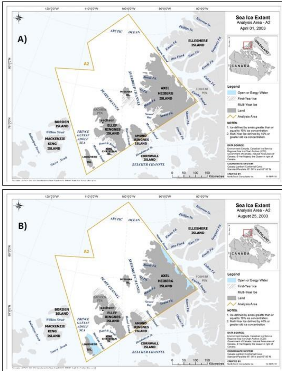
Figure 28. Extent of MYI, FYI and open water on maximum sea ice extent date (A) and minimum sea ice extent date (B) in 2003 within region A2.
