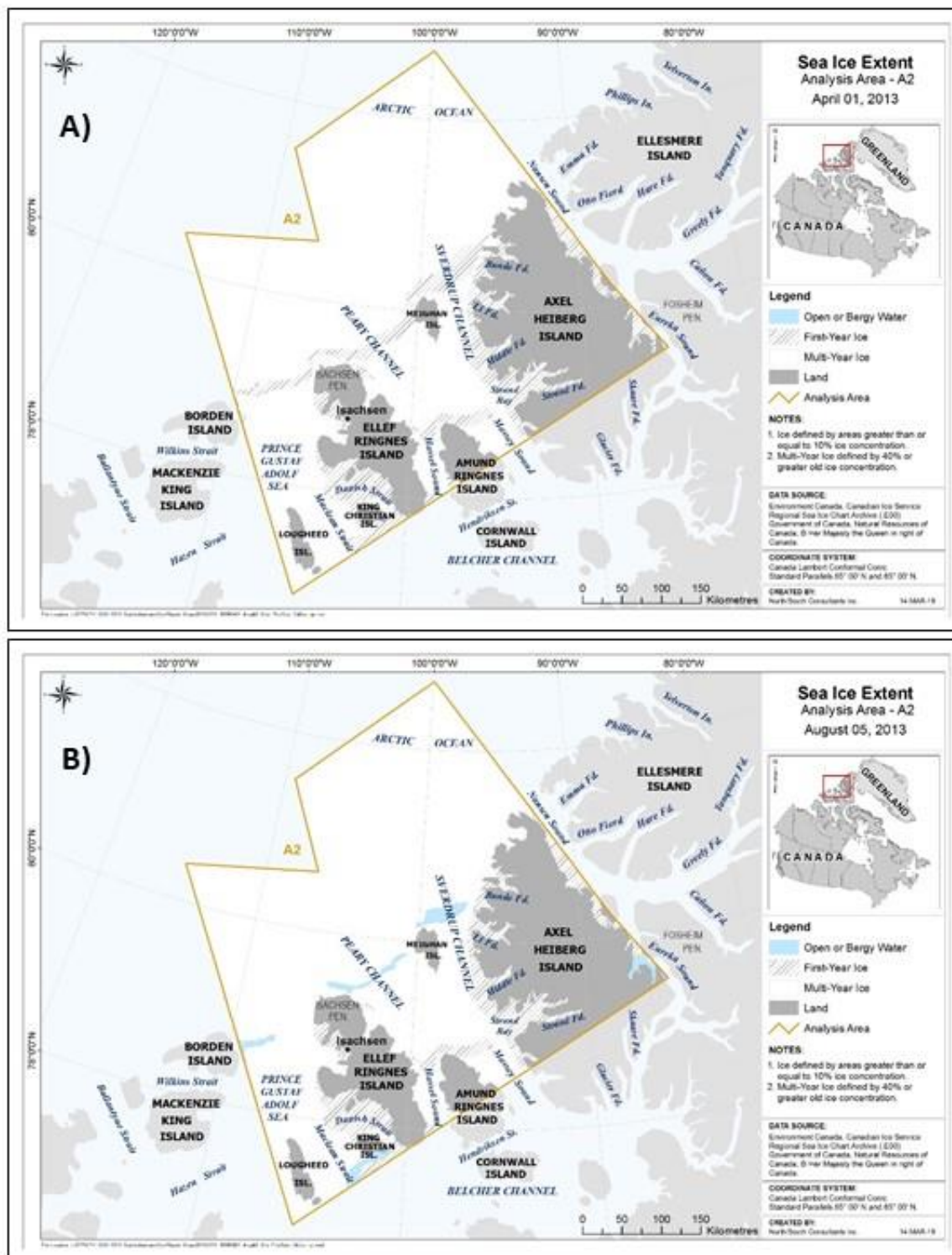
Figure 38. Extent of MYI, FYI and open water on maximum sea ice extent date (A) and minimum sea ice extent date (B) in 2013 within region A2.
