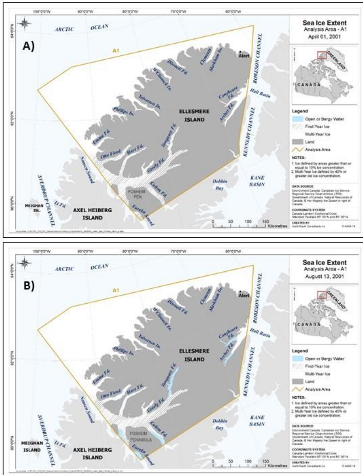
Figure 6. Extent of MYI, FYI and open water on maximum sea ice extent date (A) and minimum sea ice extent date (B) in 2001 within region A1.
