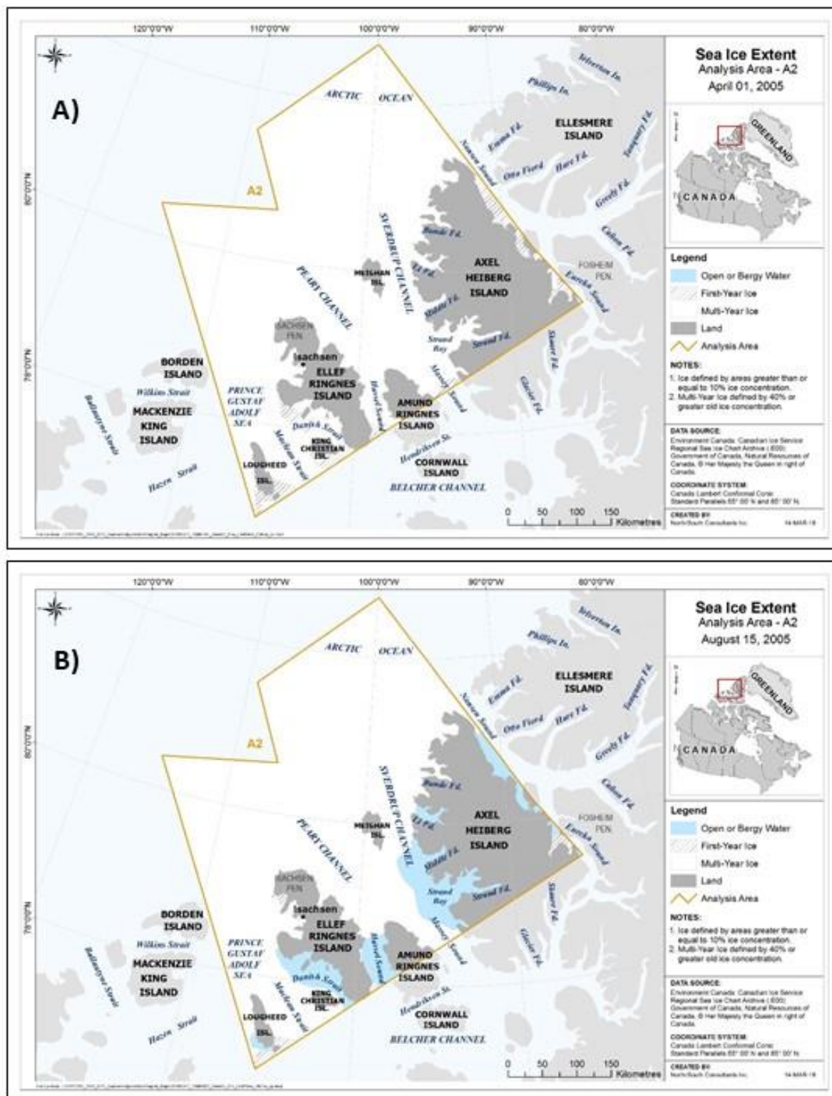
Figure 30. Extent of MYI, FYI and open water on maximum sea ice extent date (A) and minimum sea ice extent date (B) in 2005 within region A2.
