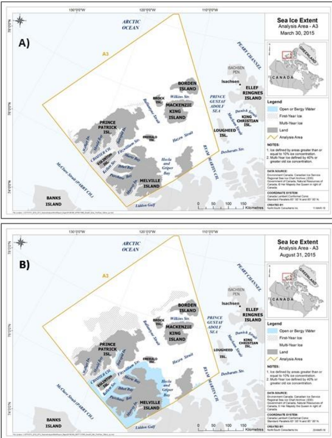
Figure 60. Extent of MYI, FYI and open water on maximum sea ice extent date (A) and minimum sea ice extent date (B) in 2015 within region A3.
