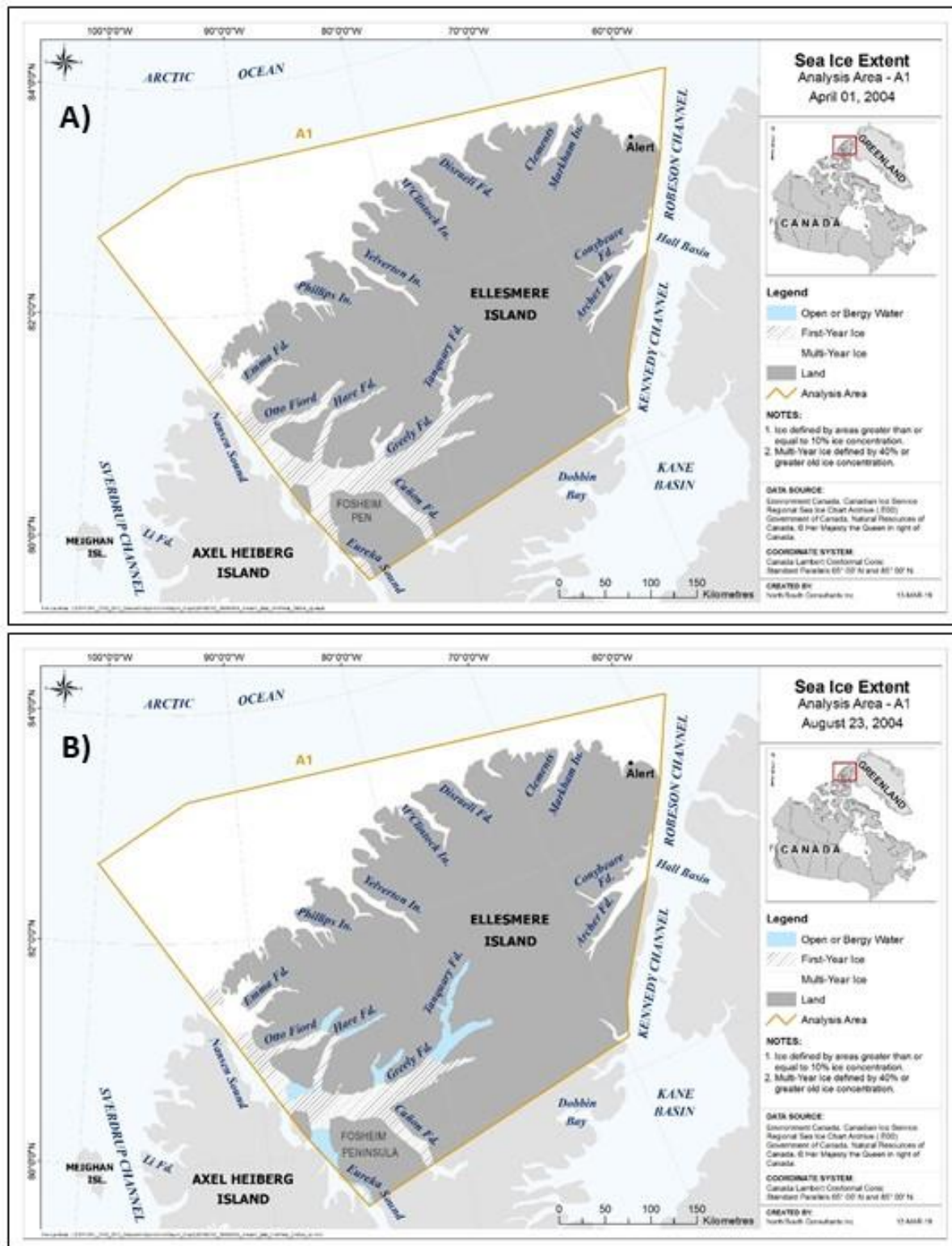
Figure 9. Extent of MYI, FYI and open water on maximum sea ice extent date (A) and minimum sea ice extent date (B) in 2004 within region A1.
