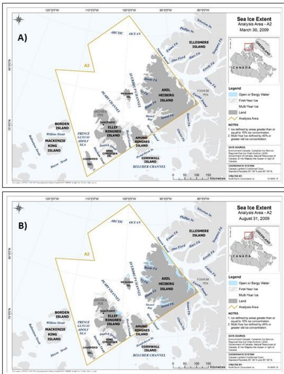
Figure 34. Extent of MYI, FYI and open water on maximum sea ice extent date (A) and minimum sea ice extent date (B) in 2009 within region A2.
