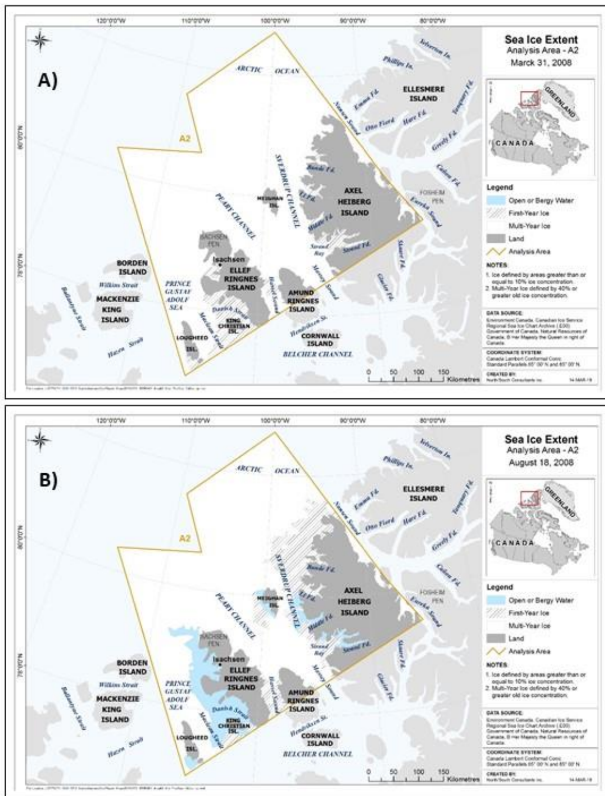
Figure 33. Extent of MYI, FYI and open water on maximum sea ice extent date (A) and minimum sea ice extent date (B) in 2008 within region A2.
