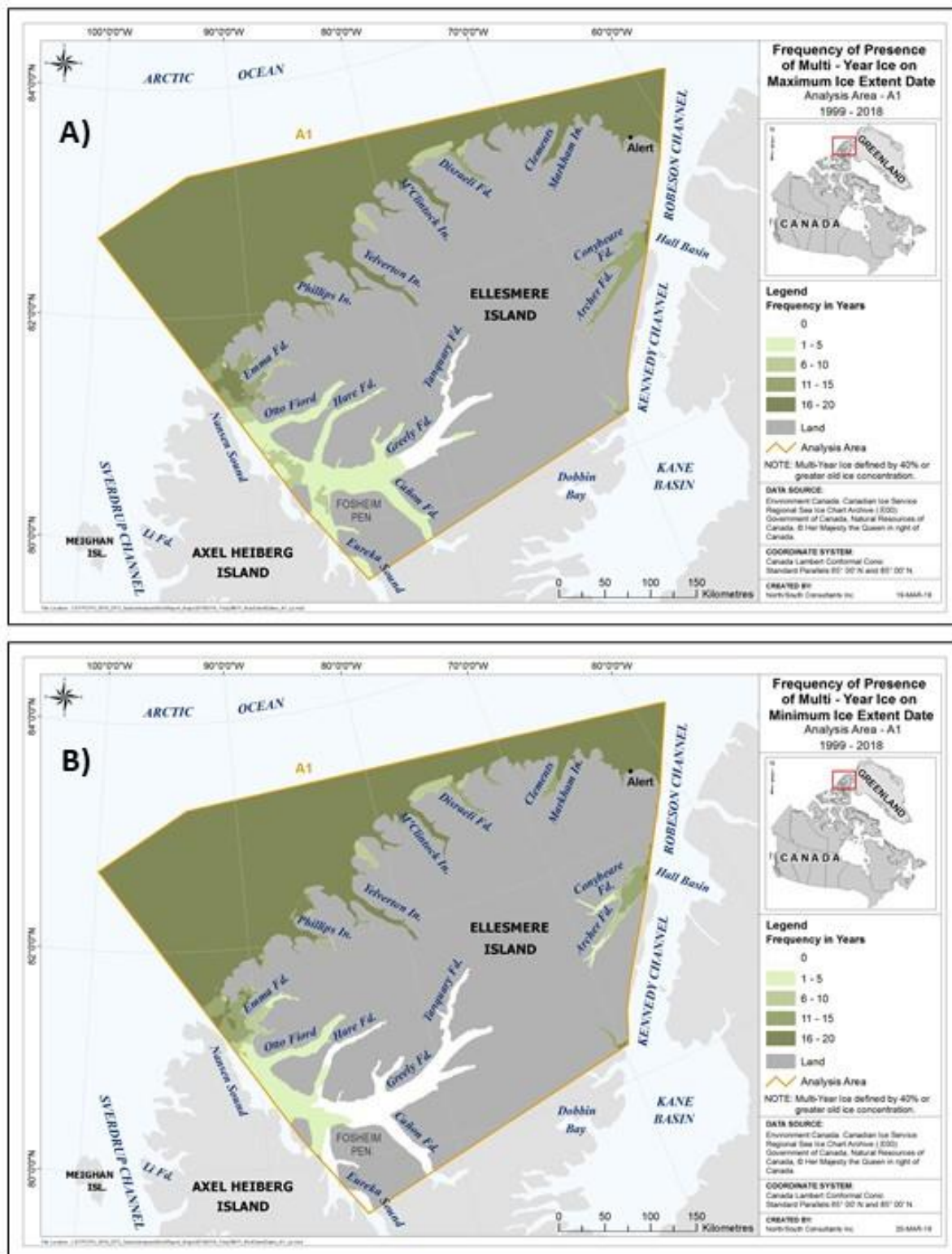
Figure 64. Frequency of occurrence of MYI on maximum sea ice extent date (A) and minimum sea ice extent date (B) between 1999 and 2018 within region A1.
