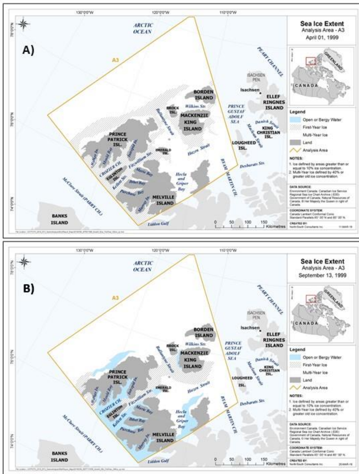
Figure 44. Extent of MYI, FYI and open water on maximum sea ice extent date (A) and minimum sea ice extent date (B) in 1999 within region A3.
