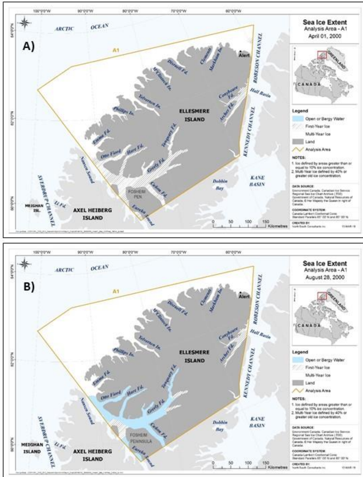
Figure 5. Extent of MYI, FYI and open water on maximum sea ice extent date (A) and minimum sea ice extent date (B) in 2000 within region A1.
