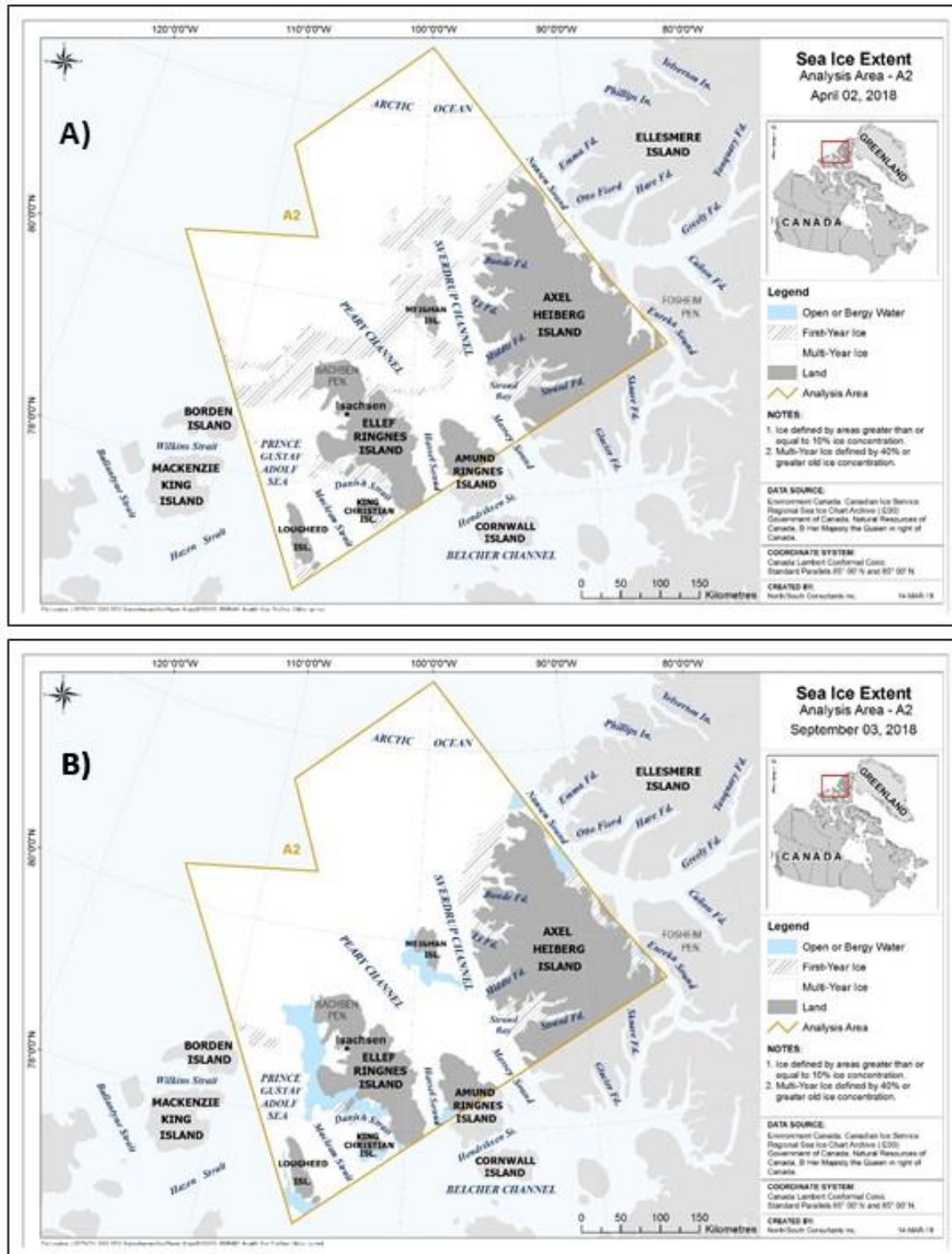
Figure 43. Extent of MYI, FYI and open water on maximum sea ice extent date (A) and minimum sea ice extent date (B) in 2018 within region A2.
