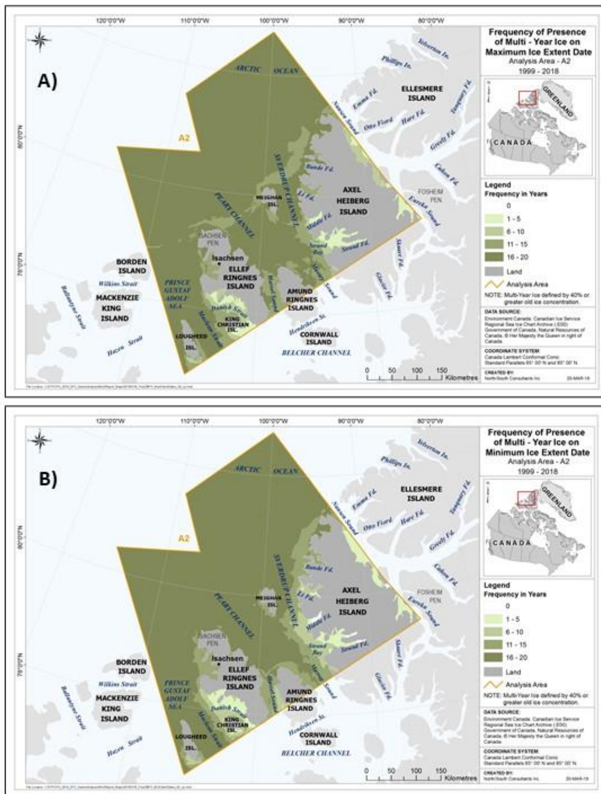
Figure 66. Frequency of occurrence of MYI on maximum sea ice extent date (A) and minimum sea ice extent date (B) between 1999 and 2018 within region A2.
