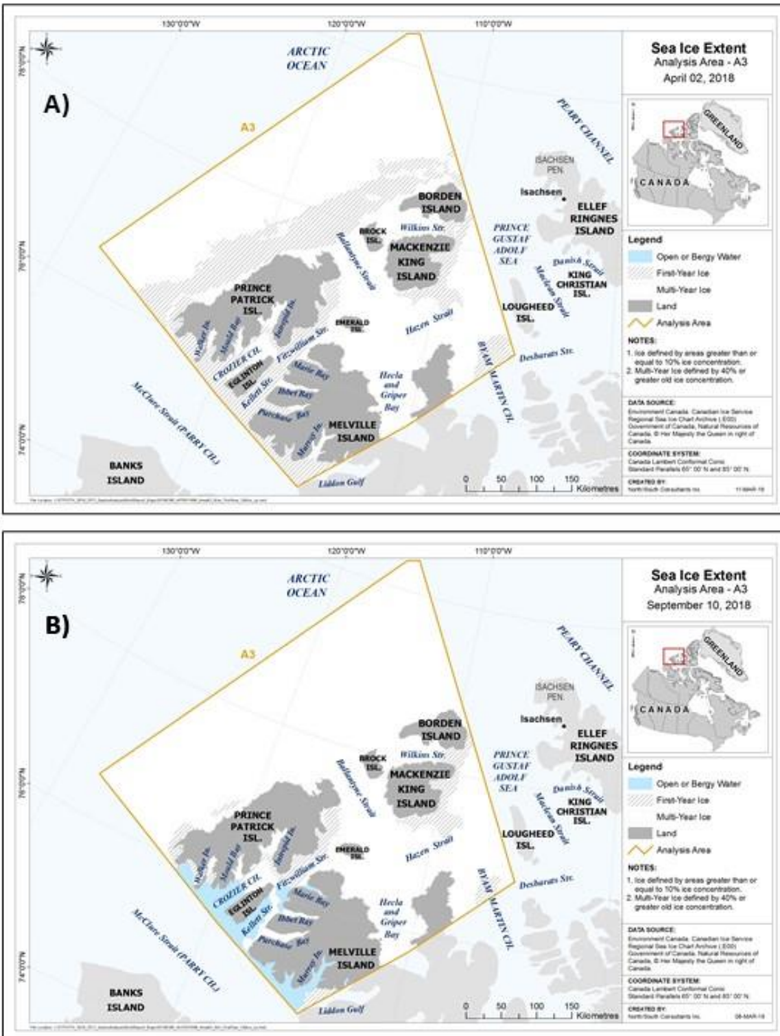
Figure 63. Extent of MYI, FYI and open water on maximum sea ice extent date (A) and minimum sea ice extent date (B) in 2018 within region A3.
