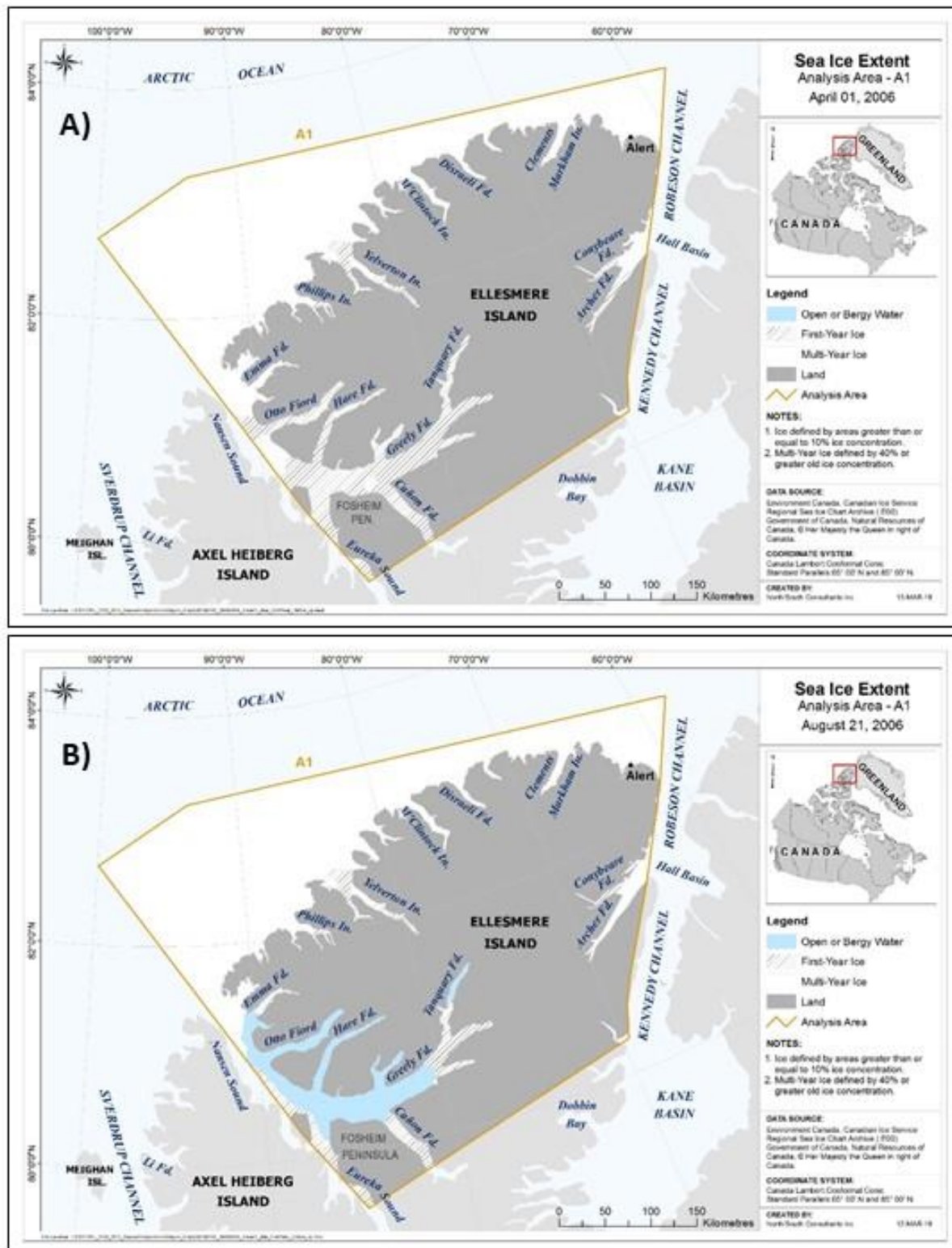
Figure 11. Extent of MYI, FYI and open water on maximum sea ice extent date (A) and minimum sea ice extent date (B) in 2006 within region A1.
