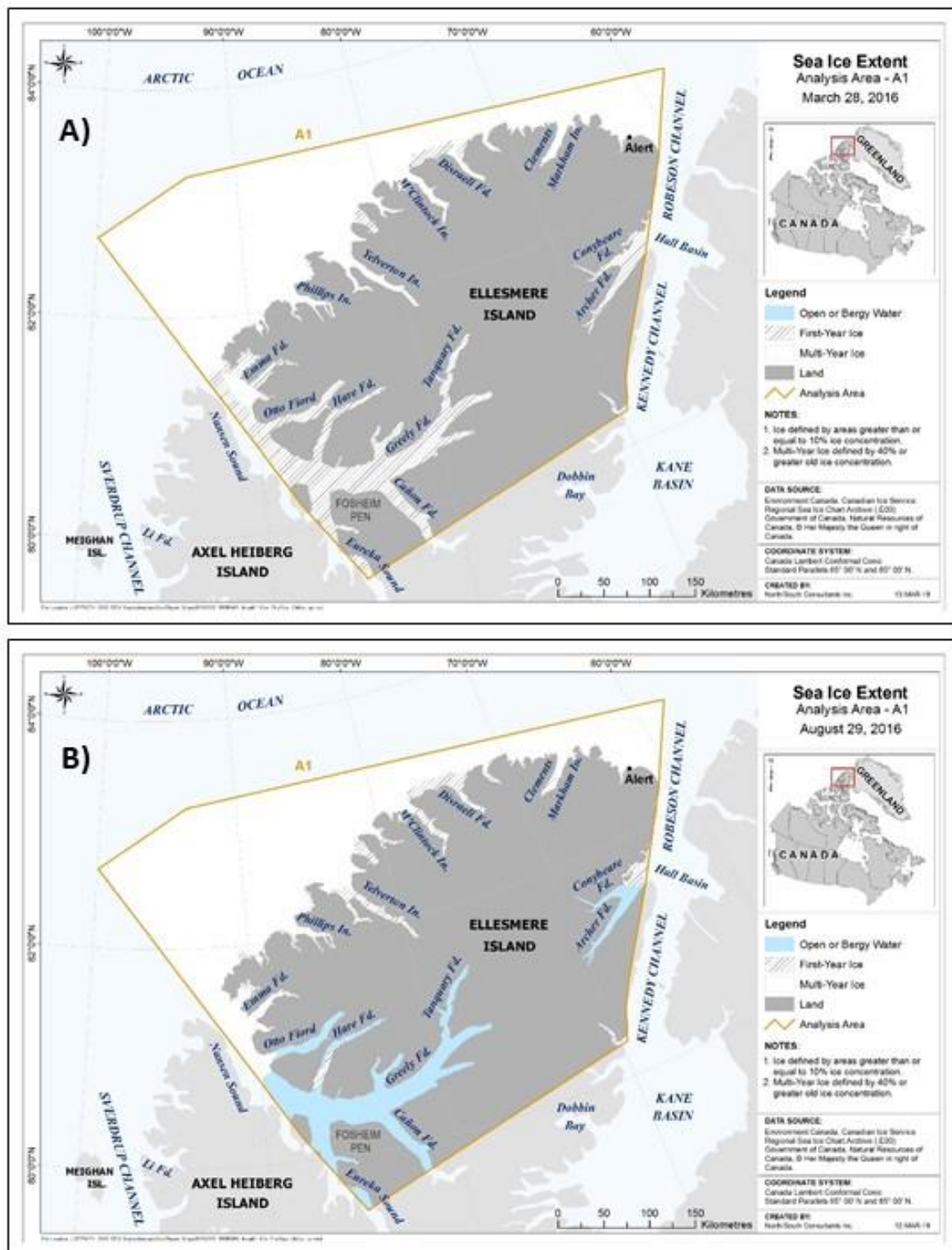
Figure 21. Extent of MYI, FYI and open water on maximum sea ice extent date (A) and minimum sea ice extent date (B) in 2016 within region A1.
