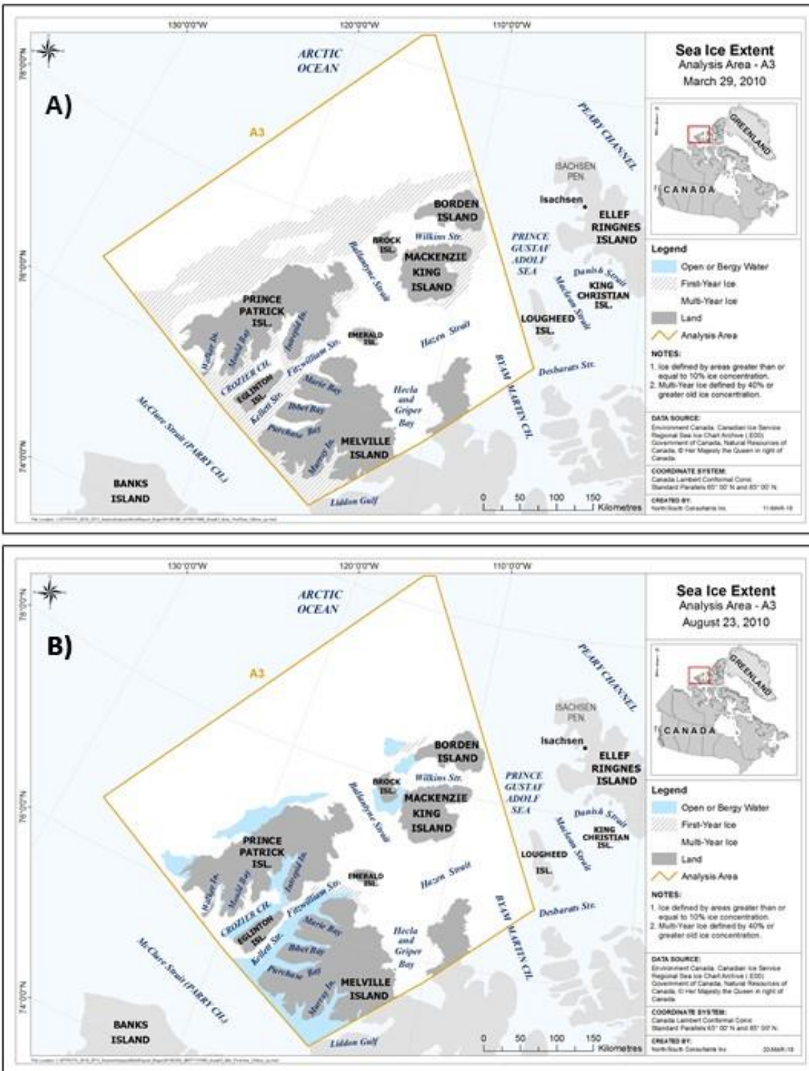
Figure 55. Extent of MYI, FYI and open water on maximum sea ice extent date (A) and minimum sea ice extent date (B) in 2010 within region A3.
