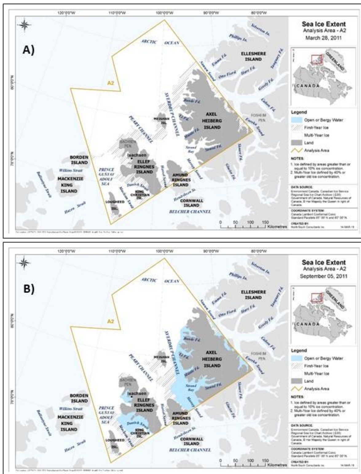
Figure 36. Extent of MYI, FYI and open water on maximum sea ice extent date (A) and minimum sea ice extent date (B) in 2011 within region A2.
