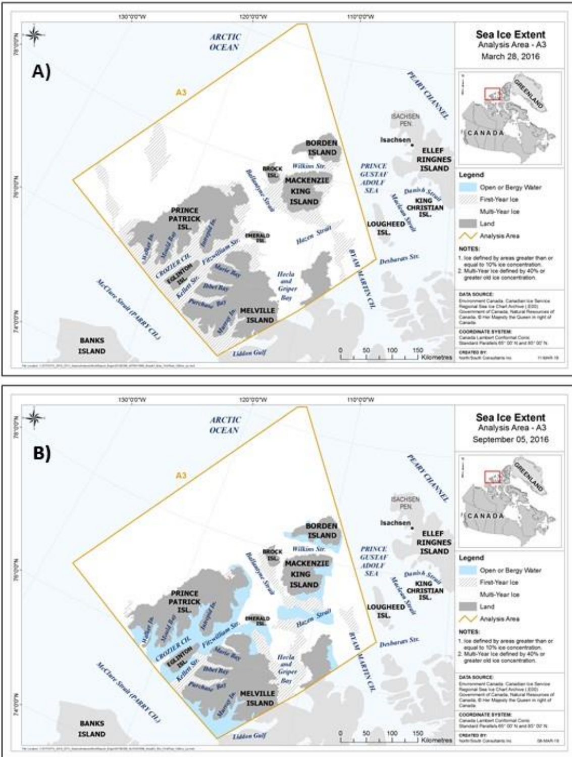
Figure 61. Extent of MYI, FYI and open water on maximum sea ice extent date (A) and minimum sea ice extent date (B) in 2016 within region A3.
