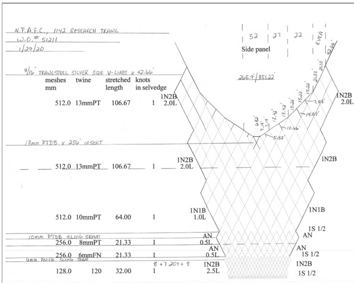
Figure A.1. Net specifications (side view) for the LFS 1142 offshore trawl net used during the Eastern Gulf of Alaska Pacific Salmon Trawl Survey for the NPAFC International Year of the Salmon Pan-Pacific Winter High Seas Expedition from February 19 to March 21, 2022 on the CCGS Sir John Franklin.
