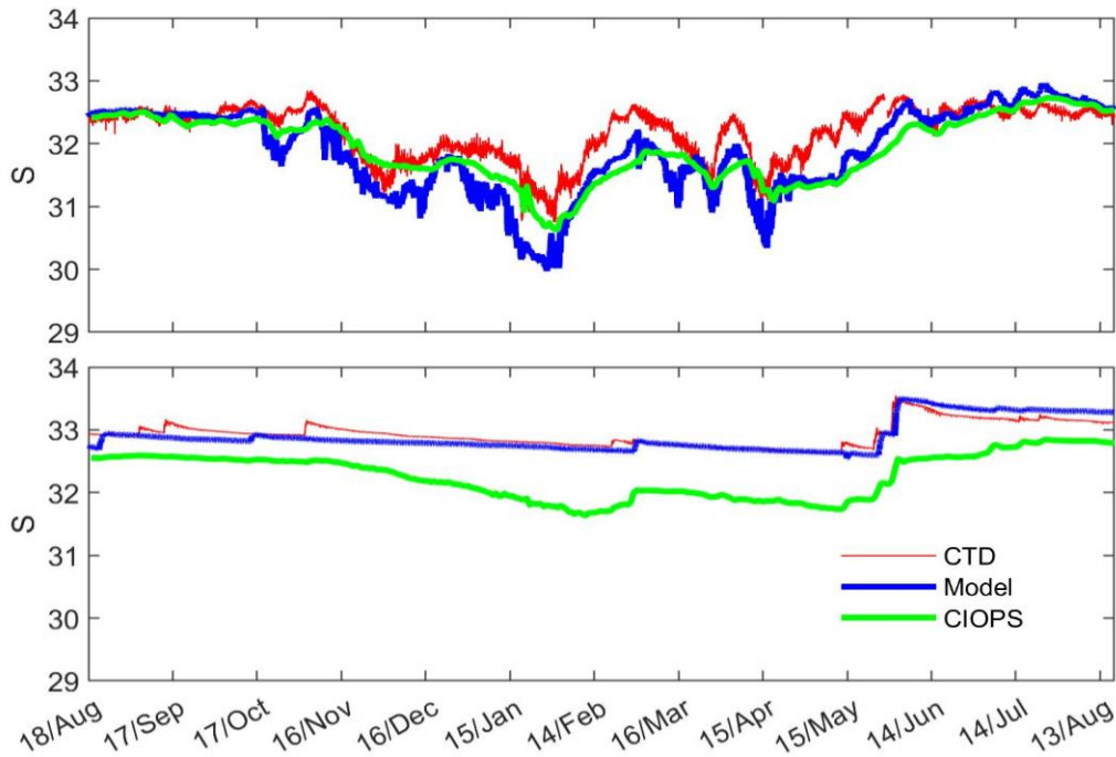
Figure 11. Relocatable model produced water salinity (blue lines) compared with daily CIOPS-W results (green lines) and CTD data (red lines) at subsurface (~40 m, upper panel) and near bottom (~150 m, lower panel) in Cook Channel. RMSE values of the relocatable model are 0.46 at subsurface and 0.12 near bottom.
