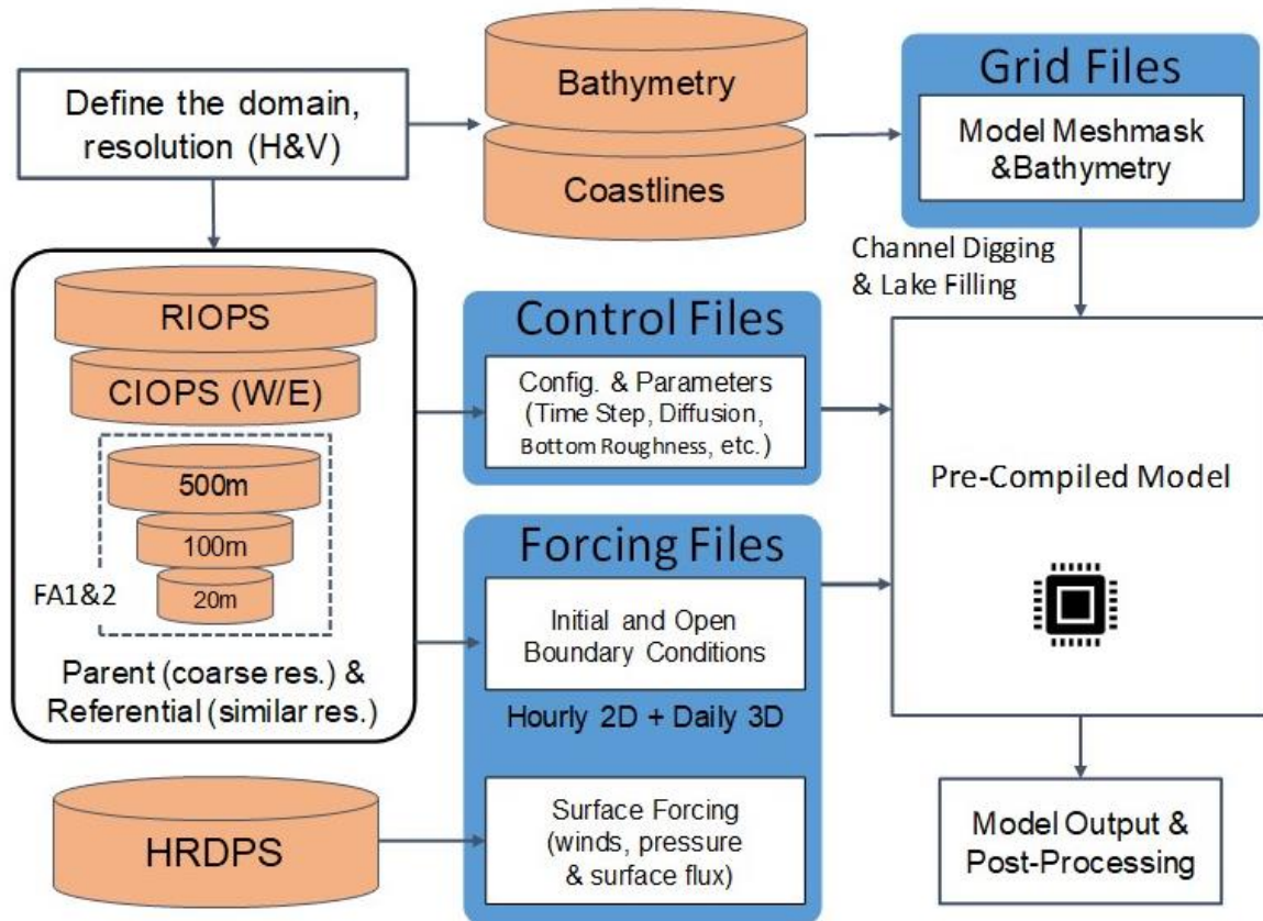
Figure 3. Workflow of the Fixed Domain On-demand Near-shore Drift Prediction System (Phase 1).
