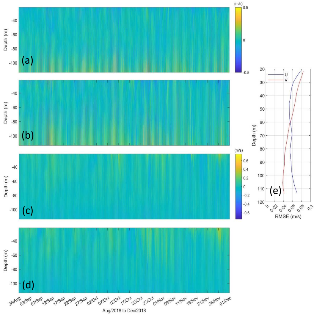
Figure 13. (a) U and (c) V components in ADCP data compared with relocatable model produced (b) U and (d) V components of ocean currents at the Chat1 site (as marked in Figure 12). Root mean square error (RMSE) of modeled U and V components is plotted in (e).
