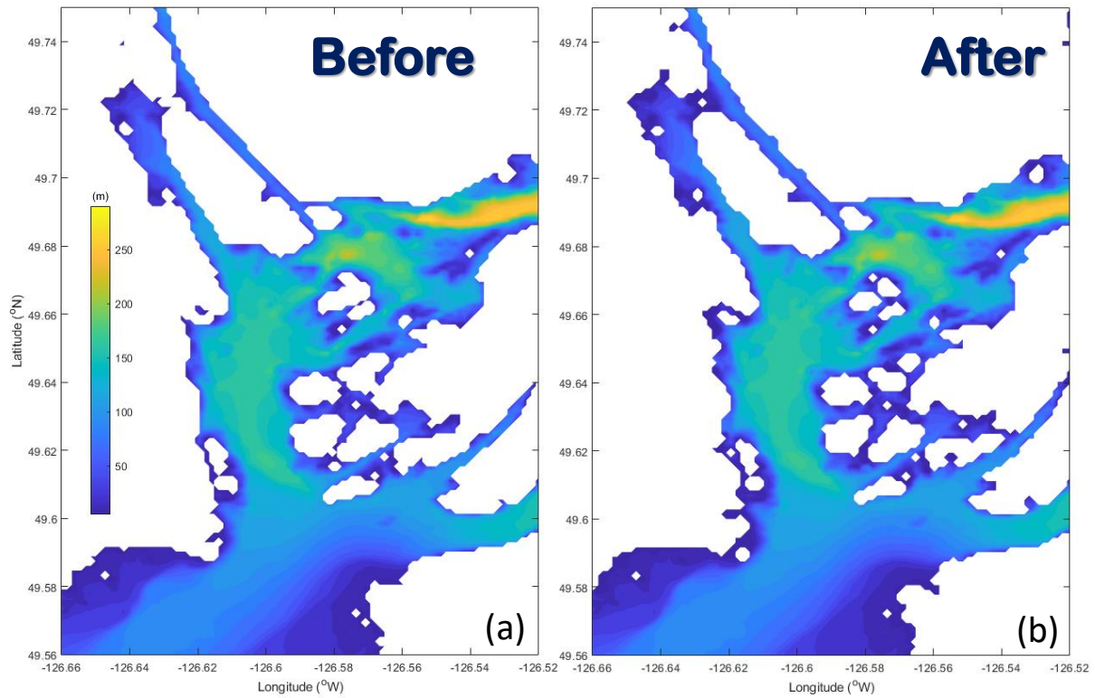
Figure 5. Automated coastline improvement in relocatable model grid over the Cook Channel area based on GSHHG coastlines using Gridtools. (a) pre-processing; (b) post-processing.
