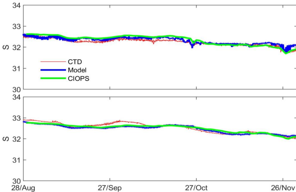
Figure 15. Nested grid model (Level-2) produced water salinity (blue lines) compared with CIOPS-W results (green lines) and CTD data (red lines) at subsurface (~50 m, upper panel) and near bottom (~103 m, lower panel) at the Chat1 site (as marked in Figure 12). RMSE values for the relocatable model are 0.10 subsurface and 0.11 near bottom.
