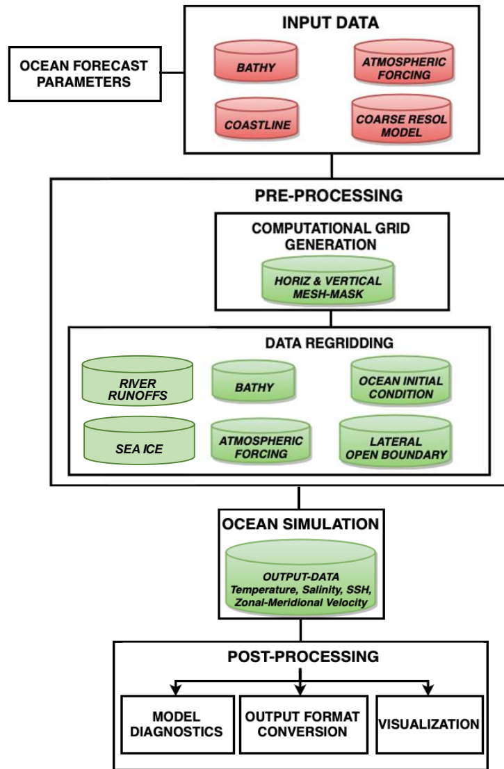
Figure 1. The structure of Fixed Domain On-demand Near-shore Drift Prediction System. Adapted from Trotta et al. (2016).
