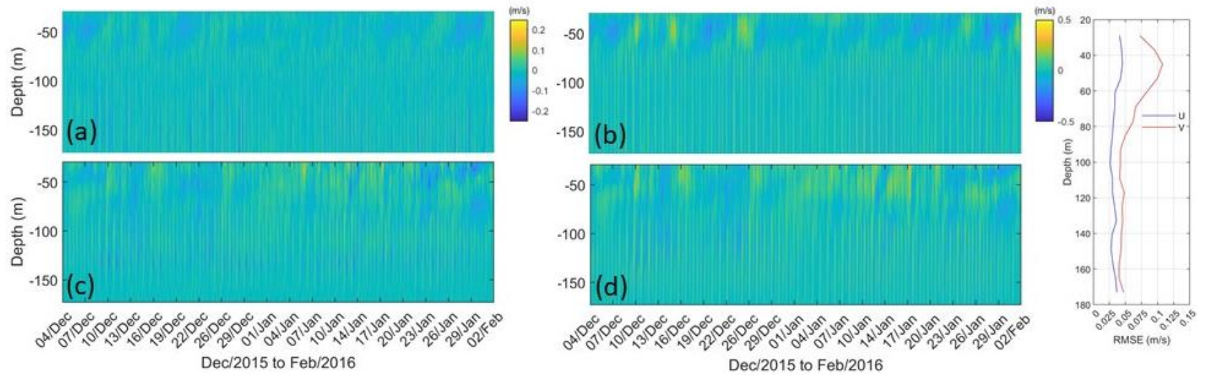
Figure 8. (a) U and (b) V components of ocean currents of near-bottom ADCP data in Zuciarte Channel. Relocatable model produced results are shown in (c) U and (d) V components for comparison. Root mean square error (RMSE) of modeled U and V components is plotted in the right panel.
