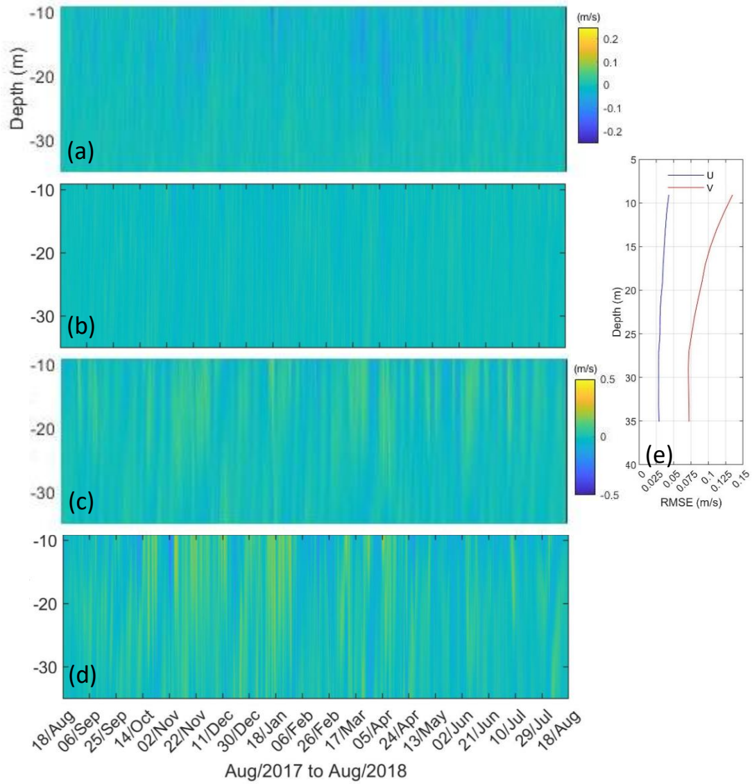
Figure 9. (a) U and (c) V components in ADCP data compared with relocatable model produced (b) U and (d) V components of ocean currents in Cook Channel. Root mean square error (RMSE) of modeled U and V components is plotted in (e).
