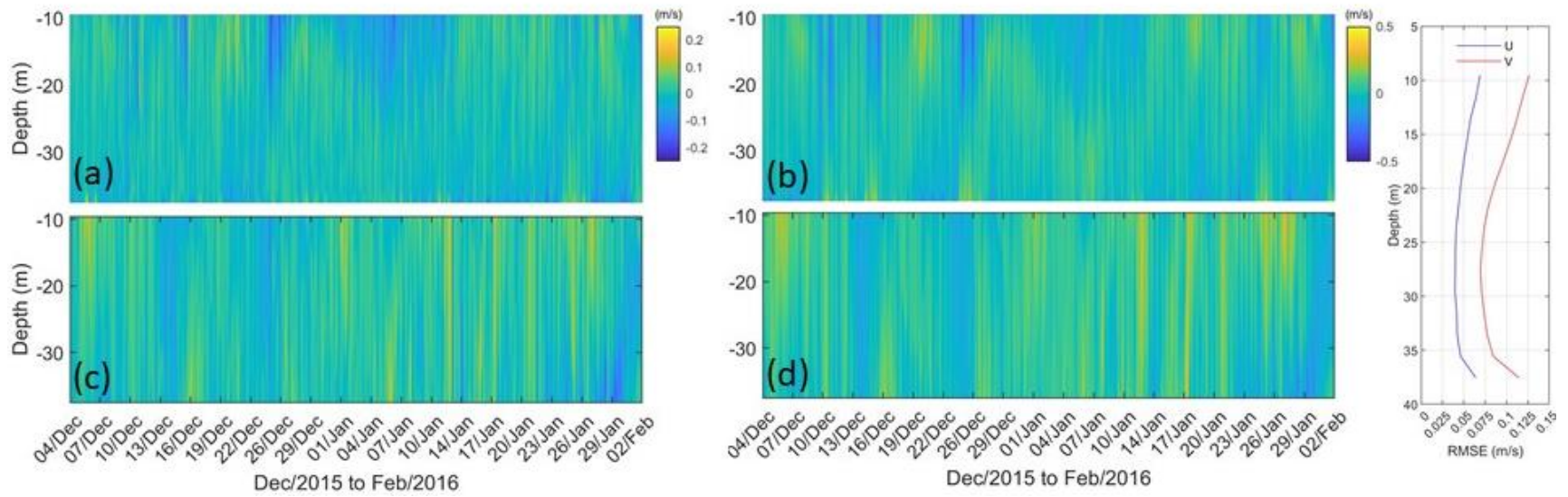
Figure 7. (a) U and (b) V components of ocean currents of subsurface ADCP data in Zuciarte Channel. Relocatable model produced results are shown in (c) U and (d) V components for comparison. Root mean square error (RMSE) of modeled U and V components is plotted in the right panel.
