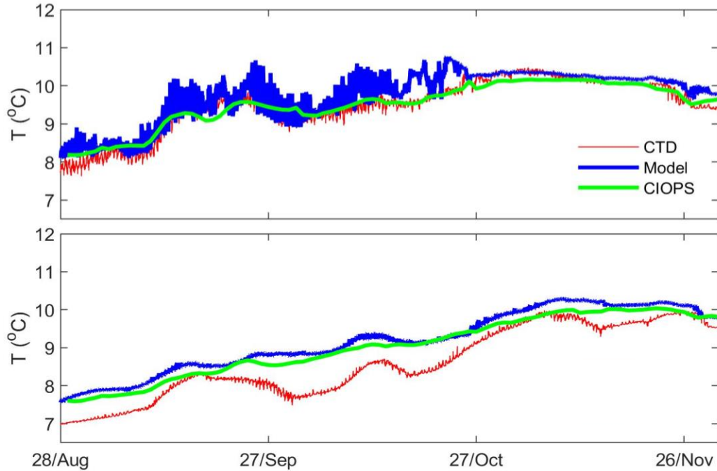
Figure 14. Nested grid model (Level-2) produced water temperature (blue lines) compared with CIOPS-W results (green lines) and CTD data (red lines) at subsurface (~50 m, upper panel) and near bottom (~103 m, lower panel) at the Chat1 site (as marked in Figure 12). RMSE values for the relocatable model are 0.36 °C subsurface and 0.64 °C near bottom.
