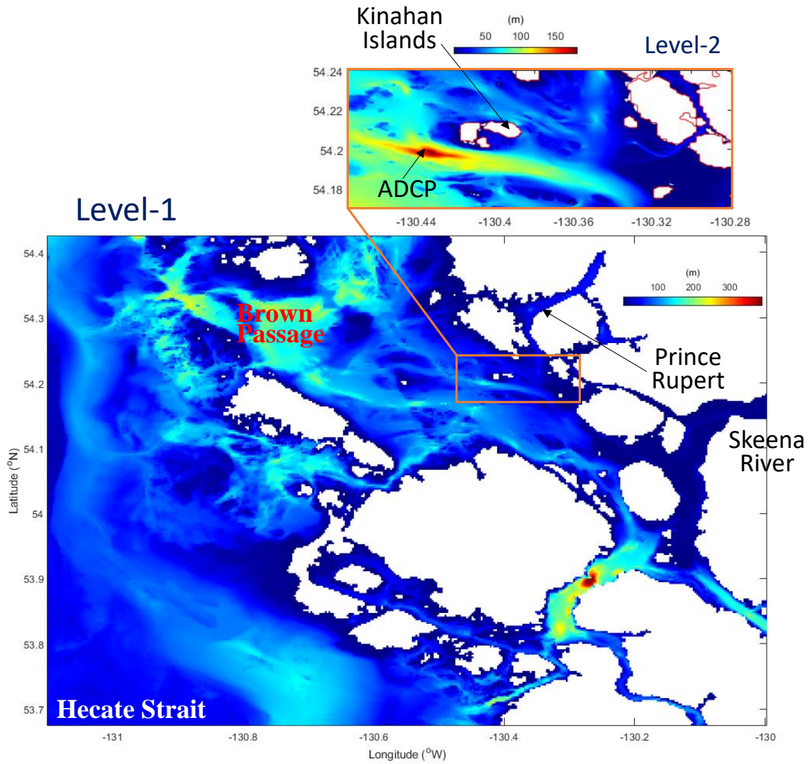
Figure 12. Relocatable model domain and bathymetry (nested grid: Level-1 and Level-2) of the case study for Prince Rupert, BC. Chat1 ADCP site has been marked on the Level-2 domain subplot.
