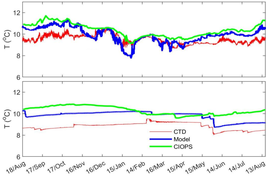
Figure 10. Relocatable model produced water temperature (blue lines) compared with daily CIOPS-W results (green lines) and CTD data (red lines) at subsurface (~40 m, upper panel) and near bottom (~150 m, lower panel) in Cook Channel. RMSE values for the relocatable model are 0.70 °C subsurface and 0.99 °C near bottom.
