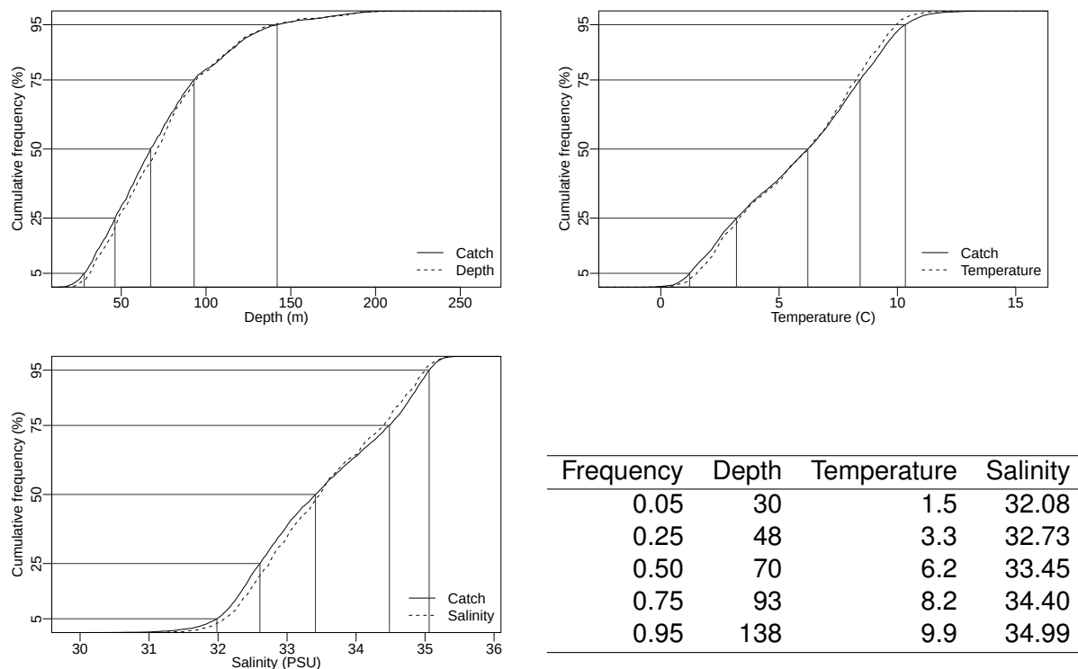
Figure 6.10E. Catch distribution by depth, temperature and salinity of Witch flounder.
