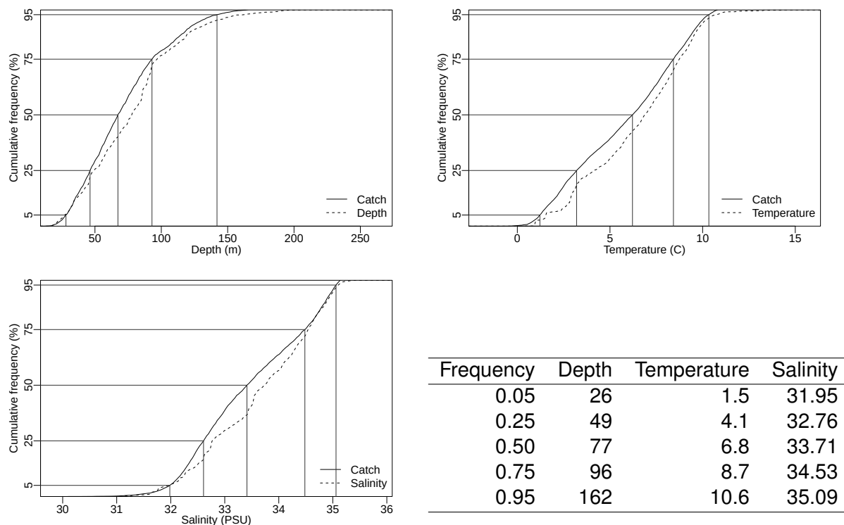
Figure 6.17E. Catch distribution by depth, temperature and salinity of Monkfish.
