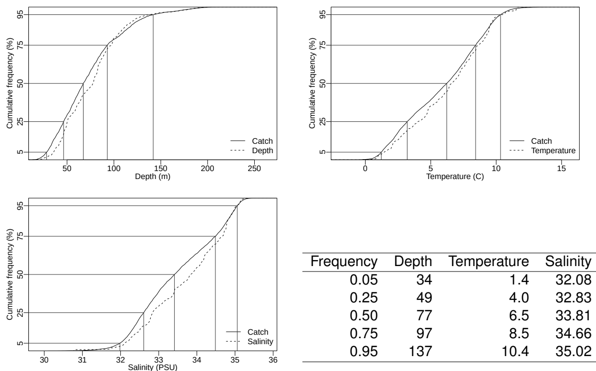
Figure 6.13E. Catch distribution by depth, temperature and salinity of Atlantic redfishes.
