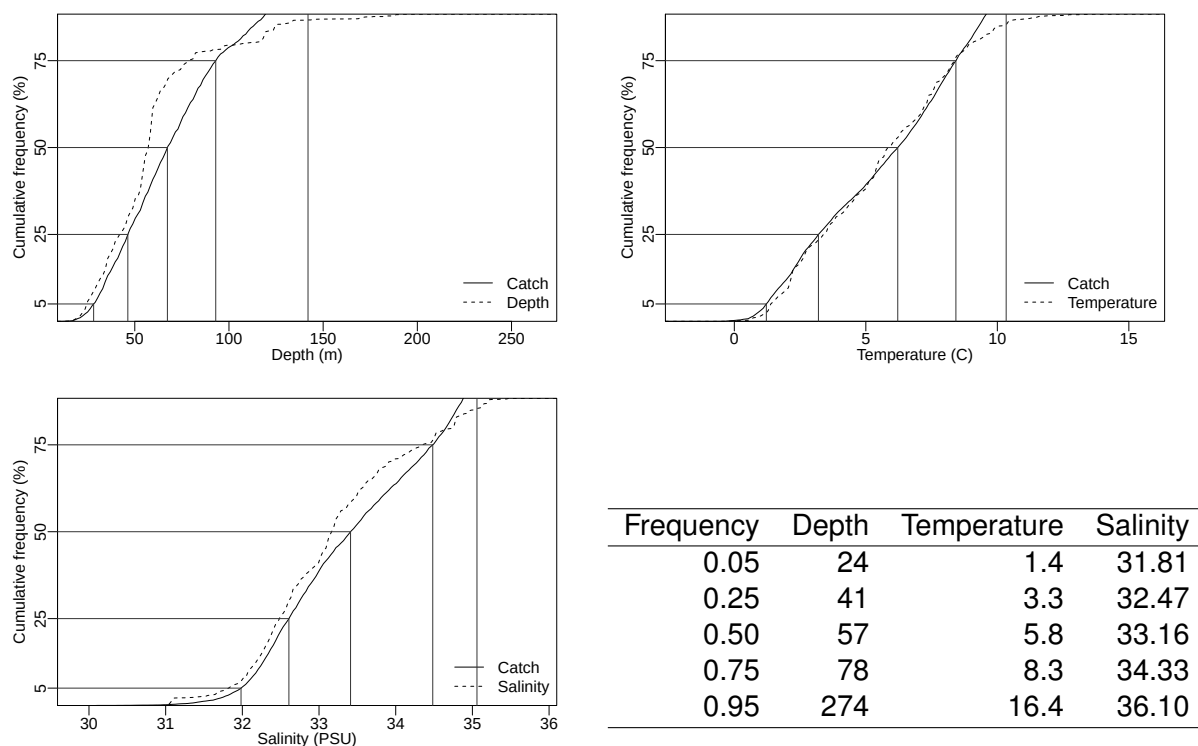
Figure 6.11E. Catch distribution by depth, temperature and salinity of Yellowtail flounder.
