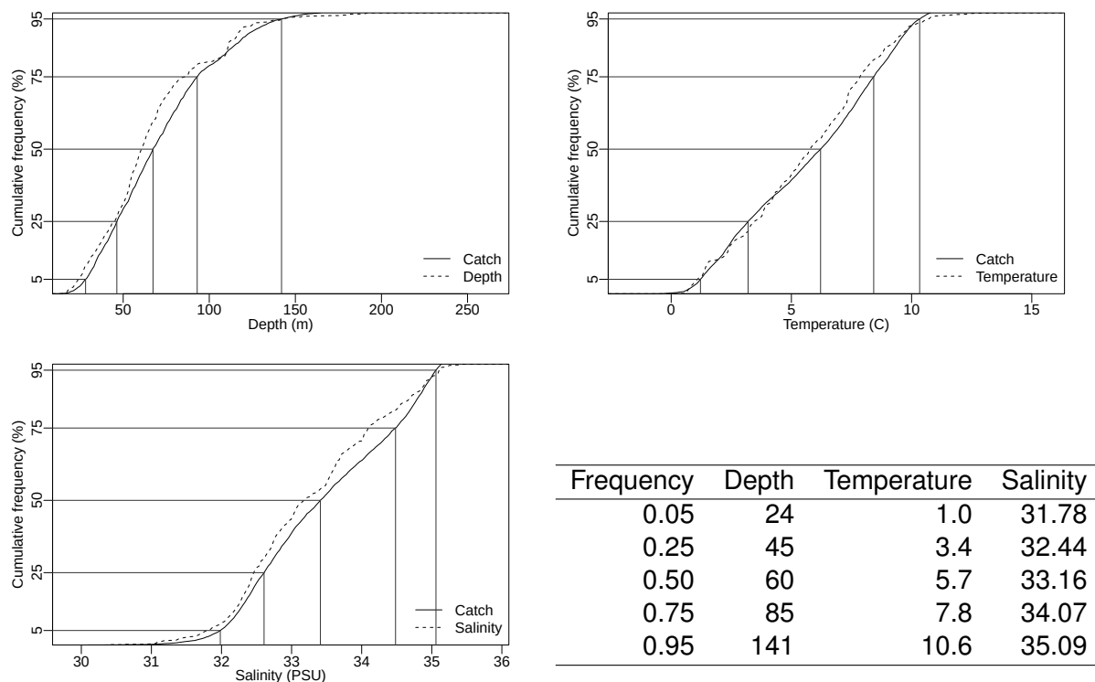
Figure 6.15E. Catch distribution by depth, temperature and salinity of Longhorn sculpin.
