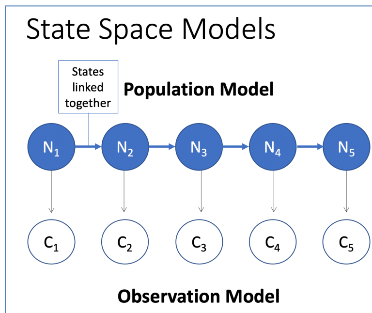
Figure E2. Example of a simple State Space Model where the population estimates are explicitly connected over time. In this type of model estimates for later years inform the estimates for all previous years. For example: a 10-year-old fish detected in the current year must have been alive in the population in each of the previous 9 years.
