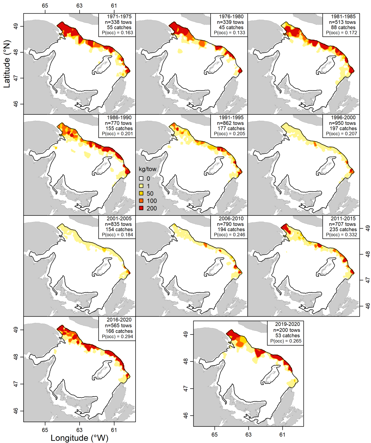
Figure 7. Spatial distribution of Redfish catches by blocks of years in the southern Gulf of St. Lawrence bottom trawl research vessel survey from 1971 to 2020. P(\text{occ}) indicates probability of occurrence (the number of tows catching Redfish divided by the total number of tows).
