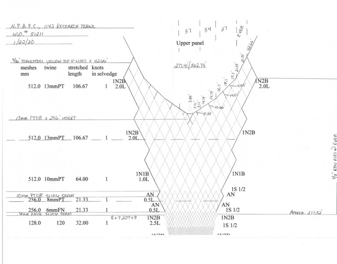
Figure A.1. Net specifications (upper view) for the offshore LFS 1142 trawl net used on the the ecosystem-based juvenile Pacific Salmon survey from October 6 to 16, 2020 on the CCGS Sir John Franklin .
