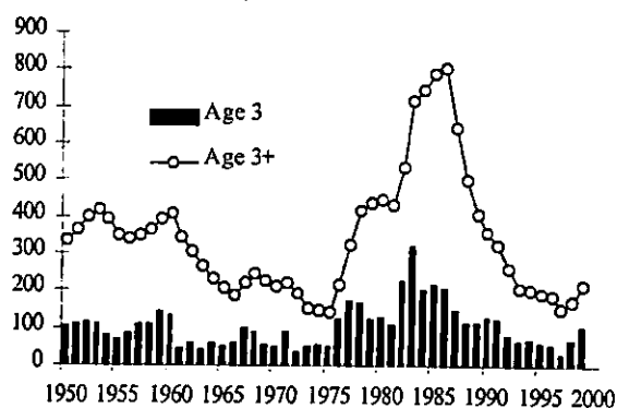
Abundance (millions)
