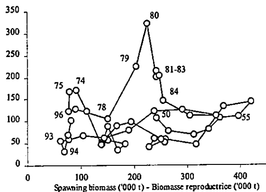
Recruits ('000)
