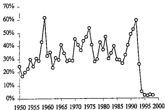
Exploitation rate (7+)
