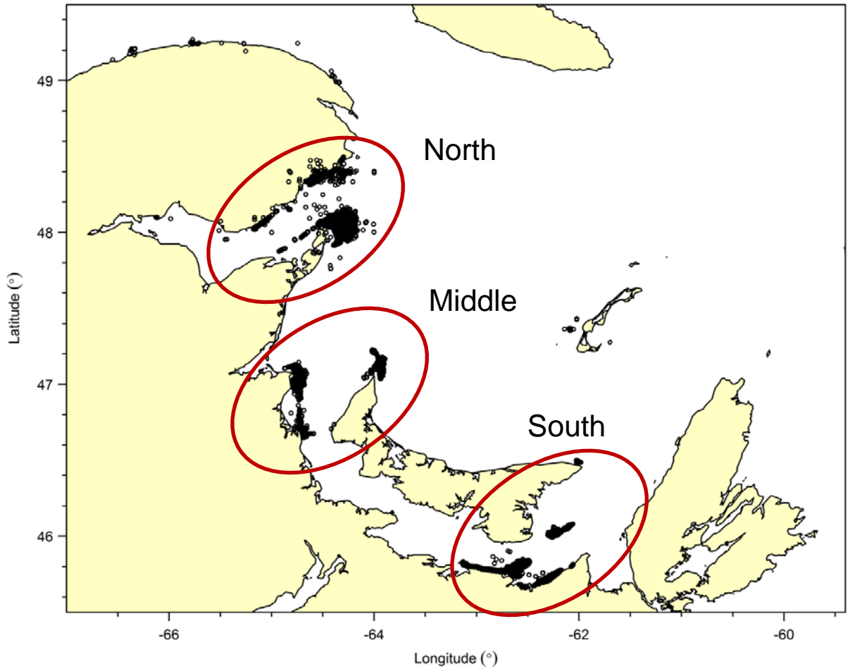
Figure 2. Geographic locations of fall herring spawning grounds in the southern Gulf of St. Lawrence and their grouping into three putative populations (north, middle, and south) for assessment and management purposes. The points represent locations of industry acoustic surveys in all area and fishing locations are from logbooks for Gaspé harvesters in the North region.
