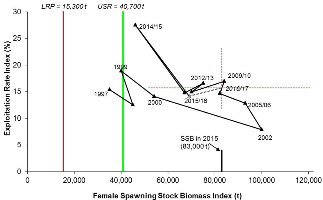
Figure 10 9 . SFA 5 IFMP Precautionary Approach framework with trajectory of exploitation rate index versus female SSB index. Data point labels denote management year. The 2015/16 fishery was ongoing; therefore the 2015/16 point is preliminary. The red cross indicates 95% confidence intervals for the fall 2015 female SSB index (horizontal line) and projected exploitation rate (vertical line), assuming that the 23,300 t TAC is maintained and taken in the 2016/17 fishery.
