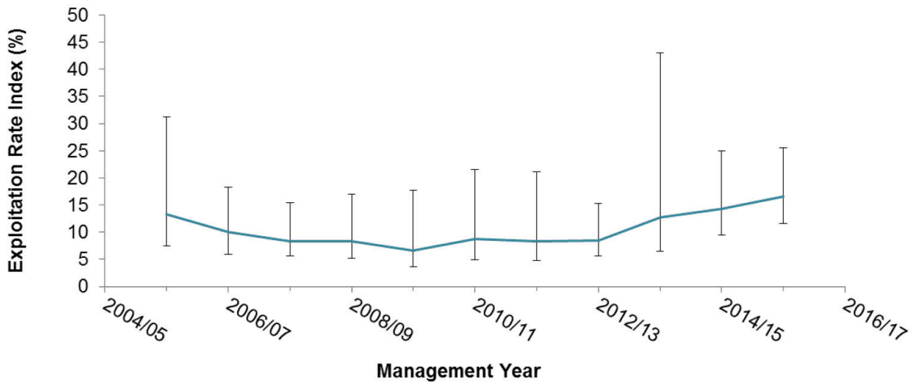
Figure 14 12 . SFA 4 Pandalus borealis Exploitation rate index based on total catch/fishable biomass index from the same year, expressed as a percentage. Error bars indicate 95% confidence intervals. The 2015/16 value is based on the February 10, 2016 CAQR, at which time the TAC had been taken.
