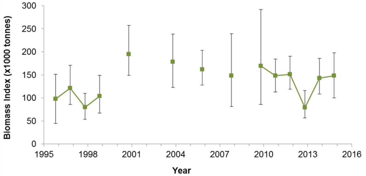
Figure 7. SFA 5 fishable biomass index. Error bars indicate 95% confidence intervals.
