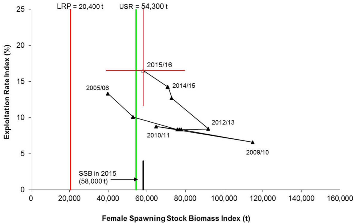
Figure 15 13 . SFA 4 Pandalus borealis IFMP Precautionary Approach framework with exploitation rate index versus female SSB index. Data point labels denote management year. The 2015/16 fishery was ongoing; therefore the 2015/16 point is preliminary. However, the TAC had been taken and that point is based on a catch of 15,065 t (101% of the TAC). The red cross indicates 95% confidence intervals for the summer 2015 female SSB index (horizontal line) and the 2015/16 exploitation rate index (vertical line).
