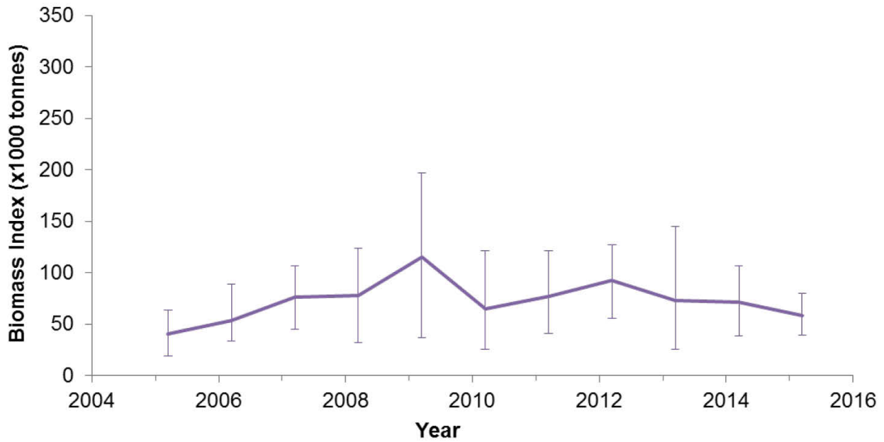
Figure 13 11 . SFA 4 Pandalus borealis female SSB index. Error bars indicate 95% confidence intervals.
