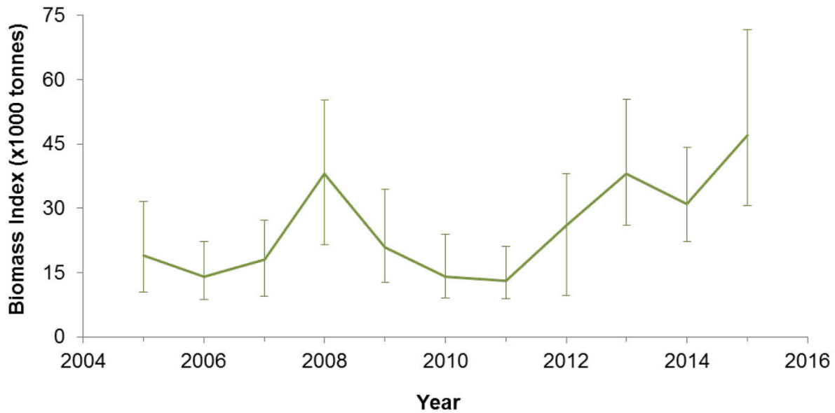
Figure 17 14 . SFA 4 fishable biomass index for Pandalus montagui . Error bars indicate 95% confidence intervals.
