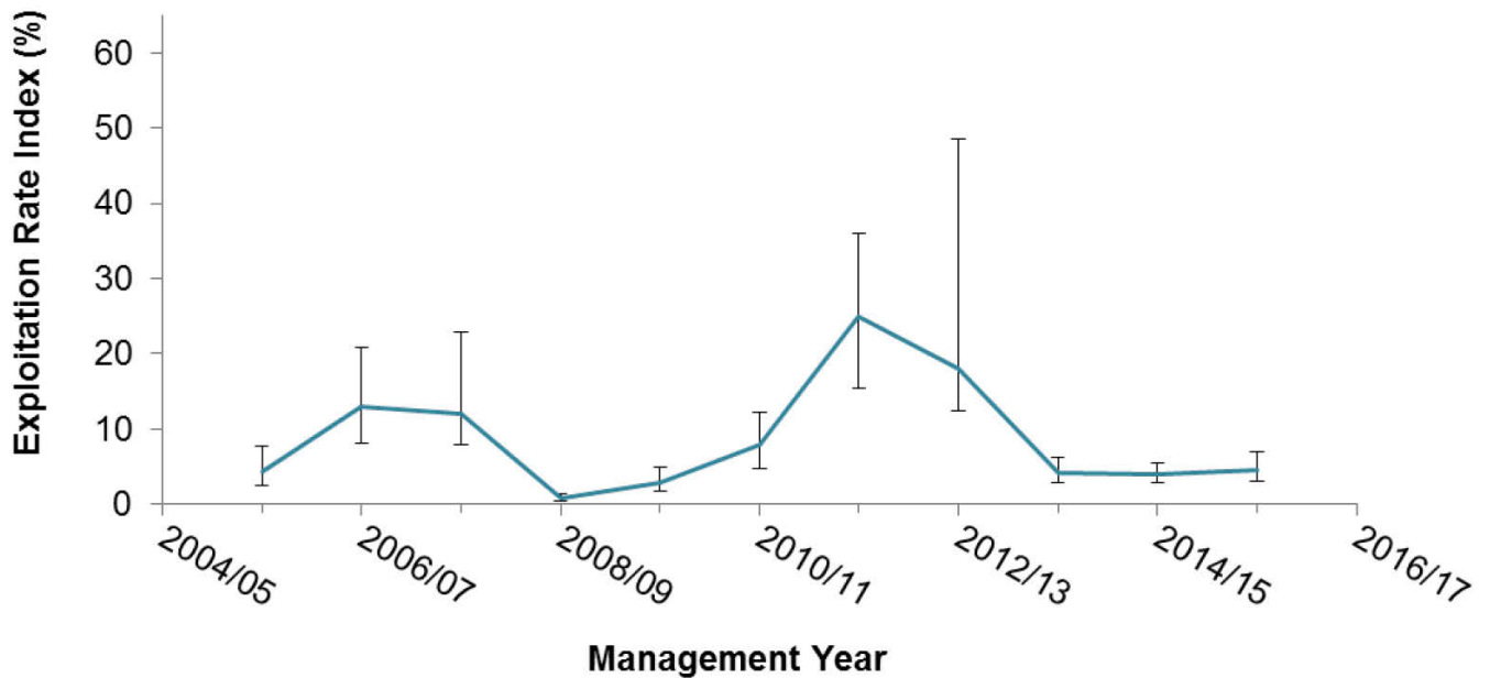
Figure 18 15 . SFA 4 Pandalus montagui exploitation rate index based on total catch/fishable biomass index from the same year, expressed as a percentage. Error bars indicate 95% confidence intervals. The 2015/16 value is preliminary.
