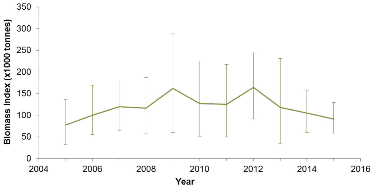
Figure 12 10 . SFA 4 Pandalus borealis fishable biomass index. Error bars indicate 95% confidence intervals.
