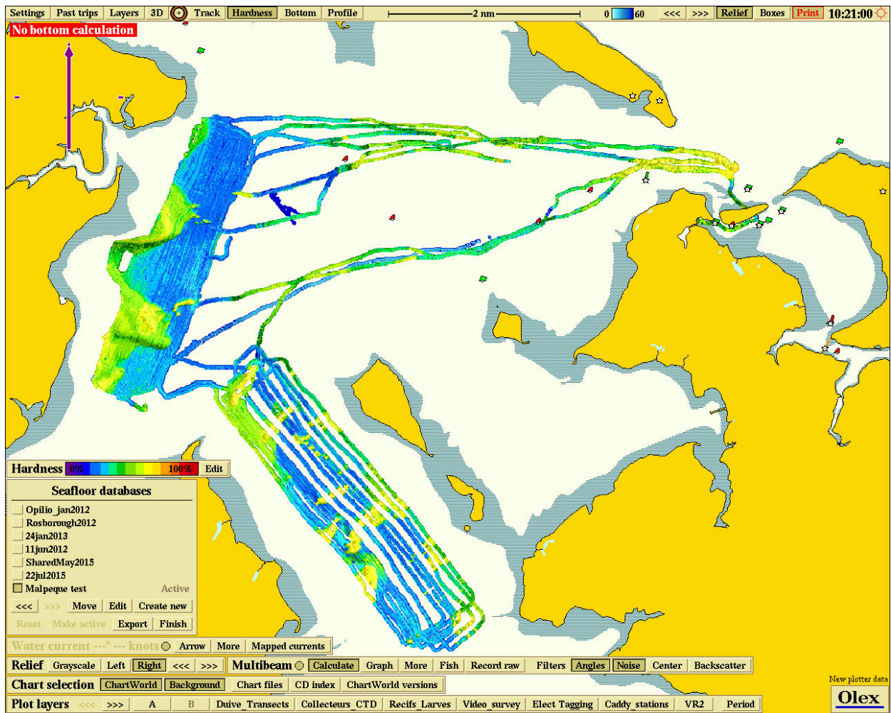
Figure 9. Total coverage of the acoustic seabed survey conducted in Malpeque Bay, PEI in August 2015 with the yellow-orange hardness variable classification identifying zones of interest.
