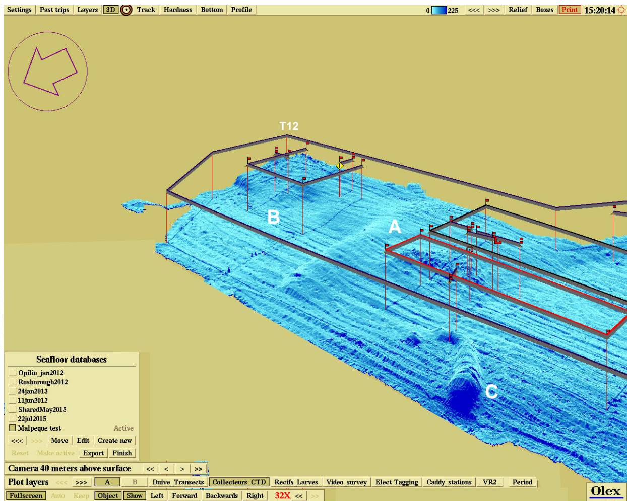
Figure 15. 3D rendering of the roughness map of the sites in the Richmond Bay area (west block; with a southwest heading), that shows a lobster reef (A: prime lobster ground) located in the southern portion and the most southern site (B), where good lobster habitat was found (T12). Map includes the proposed shellfish aquaculture sites (inner-open polygons) and location of SCUBA transects (double red flags). The seabed feature (C) was identified by SCUBA as a mound of shells.
