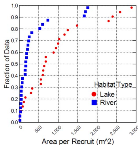
Figure 2. The cumulative distributions of area per recruit values for lake and river habitats, based on the data set available to the meeting.
