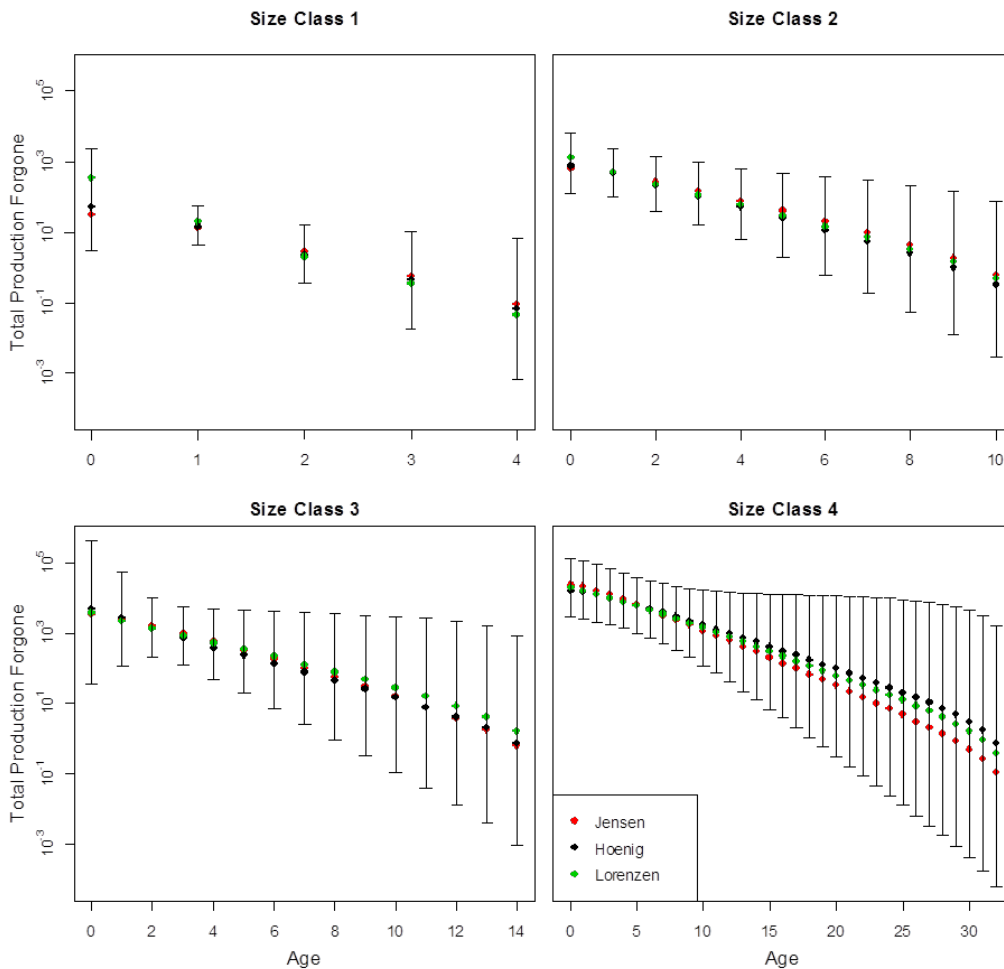
Figure 3. Total production forgone ( g \cdot APR^{-1} \cdot y^{-1} ) for the loss of the number of individuals equal to one adult at the age-of-maturity. Size classes were: Class 1 <20 cm; Class 2 20-40 cm; Class 3 40-70 cm; and Class 4 > 70 cm. The error bars represent 95% confidence intervals.
