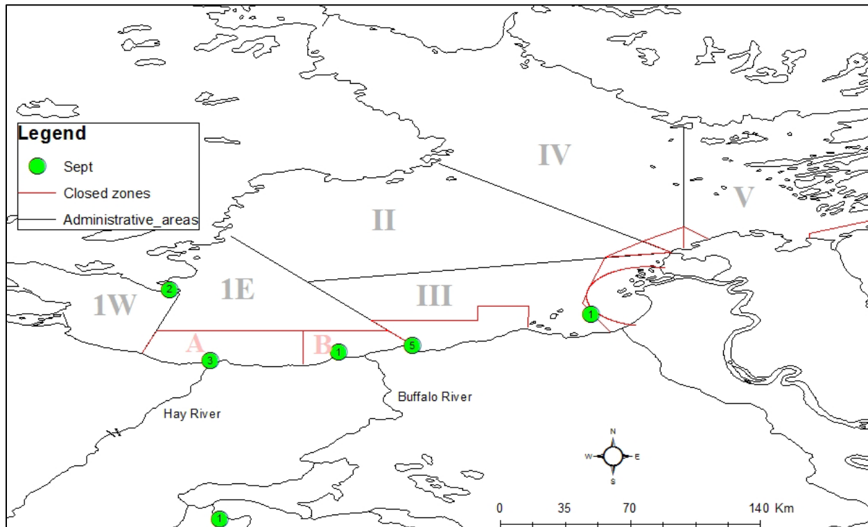
Figure 3. Great Slave Lake showing September recapture locations (circles) for Inconnu marked with T-bar anchor tags at the mouths of the Buffalo River and Yates River in 1976-1978 (DFO unpubl. data) and from 1995-2008 (VanGerwen-Toyne et al. 2013) (X). Numbers inside the circle indicate the number of Inconnu recaptured.
