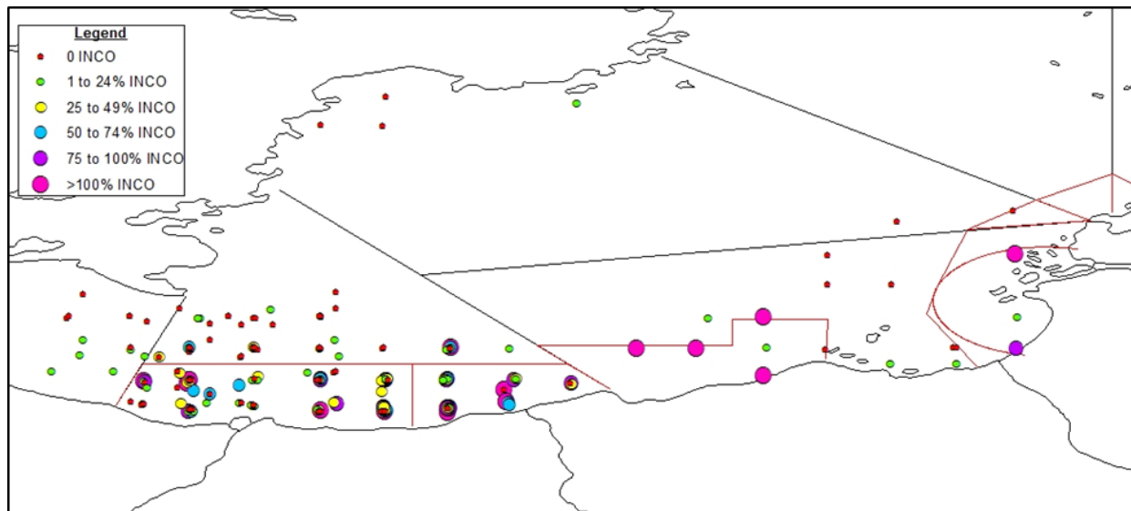
Figure 10. Percent of Inconnu caught compared to Lake Whitefish in Great Slave Lake during the Fishery Independent Harvest Study from late June to Mid- to late August, 2010 to 2013.
