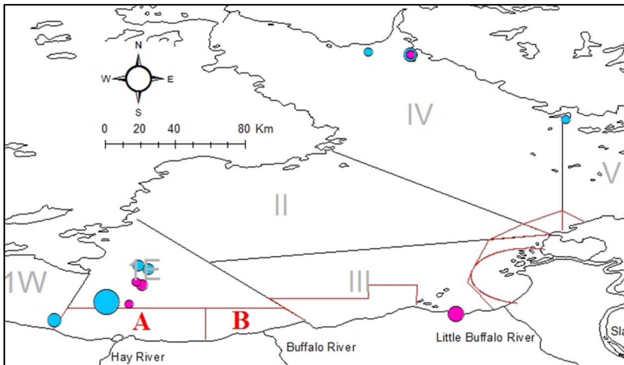
Figure 4. Great Slave Lake showing location and catch-per-unit-effort (circles) of Inconnu reported in commercial logbooks in September (blue) and October (pink) 2010-2013. Circle diameter increases with CPUE.
