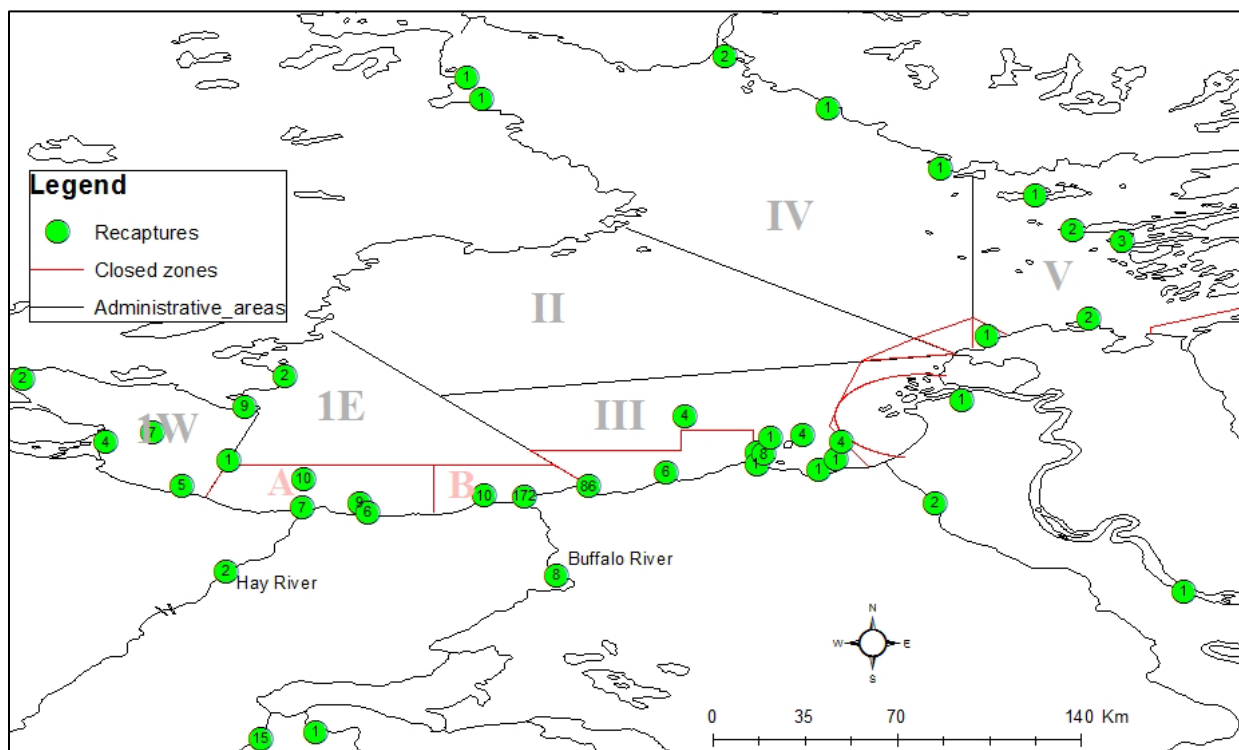
Figure 2. Great Slave Lake showing all recapture locations (circles) for Inconnu marked with T-bar anchor tags at the mouths of the Buffalo River and Yates River in 1976-1978 (DFO unpubl. data) and from 1995-2008 (VanGerwen-Toyne et al. 2013) (X). Numbers inside the circle indicate the number of Inconnu recaptured.
