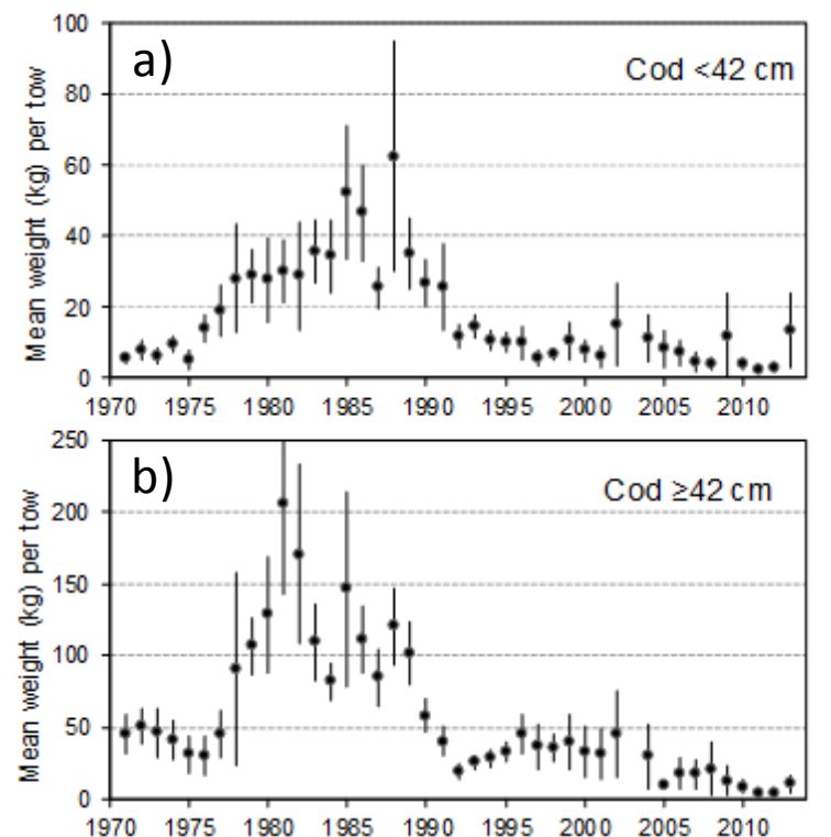
Figure 2. RV survey biomass indices for Atlantic cod of pre-commercial (a) and commercial (b) lengths. These size classes correspond approximately to juvenile and adult cod. Vertical lines denote approximate 95% confidence limits ( \pm 2 standard errors).
