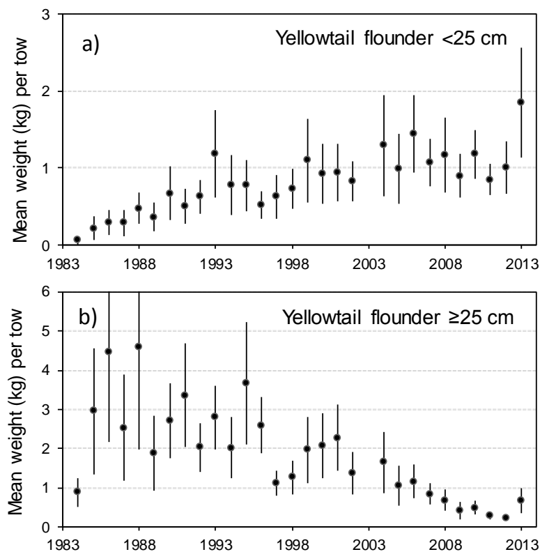
Figure 11. RV survey biomass indices for yellowtail flounder of pre-commercial (a) and commercial (b) lengths. Vertical lines denote approximate 95% confidence limits. Indices are based on strata 401-403 in addition to the standard strata 415-439; hence the indices begin in 1984 instead of 1971.
