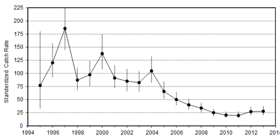
Figure 4. Standardized catch rate (kg/1000 hooks) for Atlantic cod (all sizes) from the sentinel longline program. Vertical lines denote approximate 95% confidence limits.
