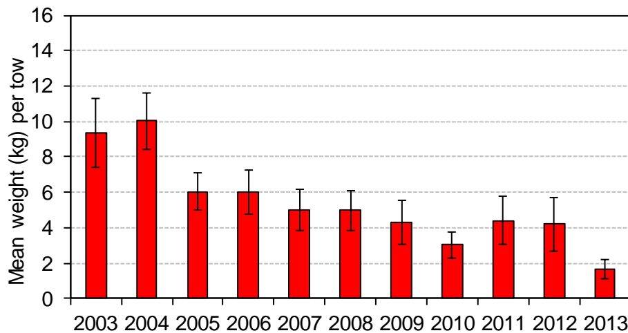
Figure 6. Biomass index for American plaice (all sizes) from the sentinel bottom-trawl survey. Vertical lines denote approximate 95% confidence limits. The indices have been standardized for differences in fishing efficiency between vessels.
