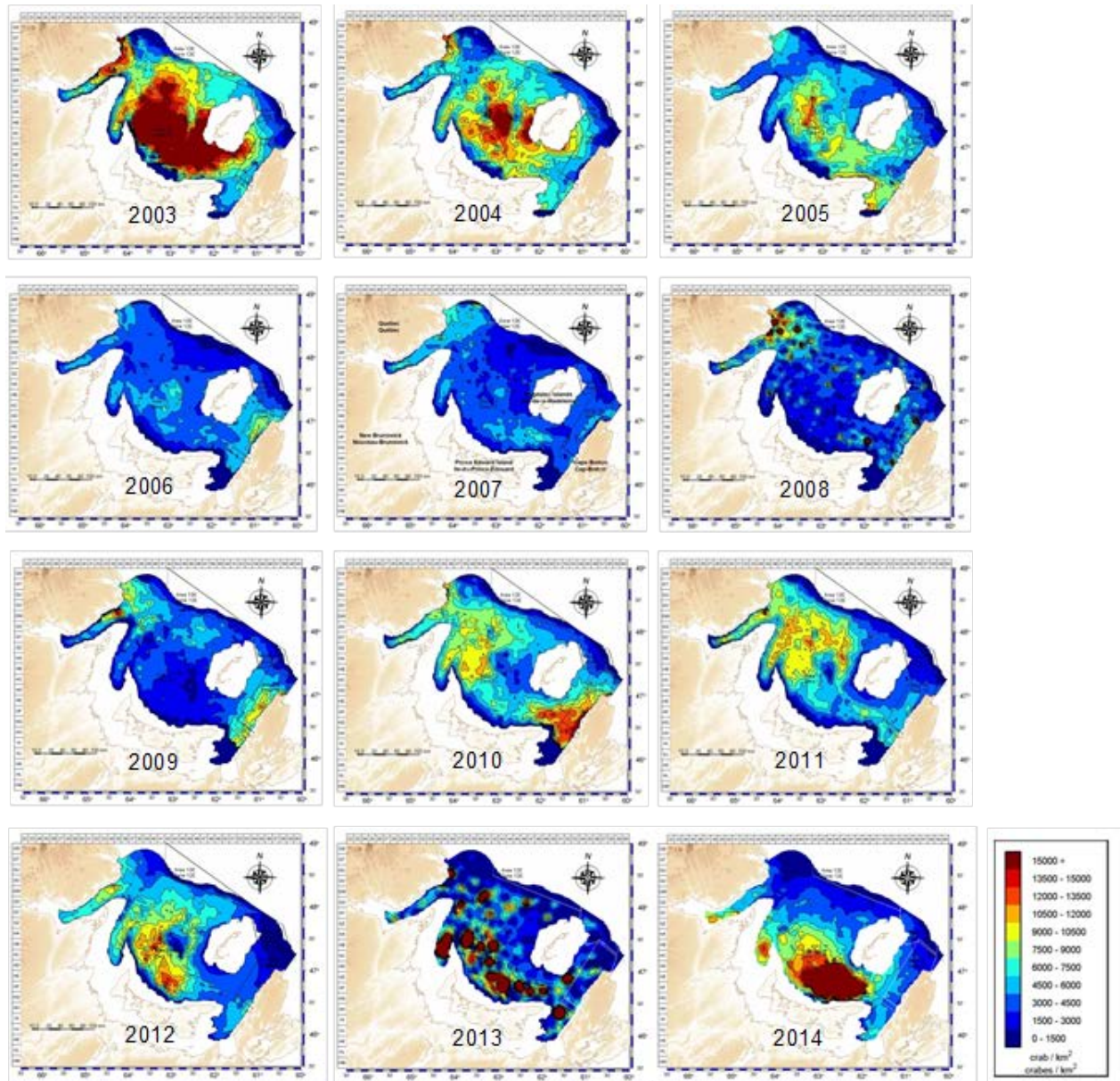
Figure 20. Density (number per km 2 ) contours of adolescent male snow crab, ( Chionoecetes opilio ), \geq 56 mm of carapace width, based on the trawl surveys conducted in the southern Gulf of St. Lawrence, 2003 to 2014.
