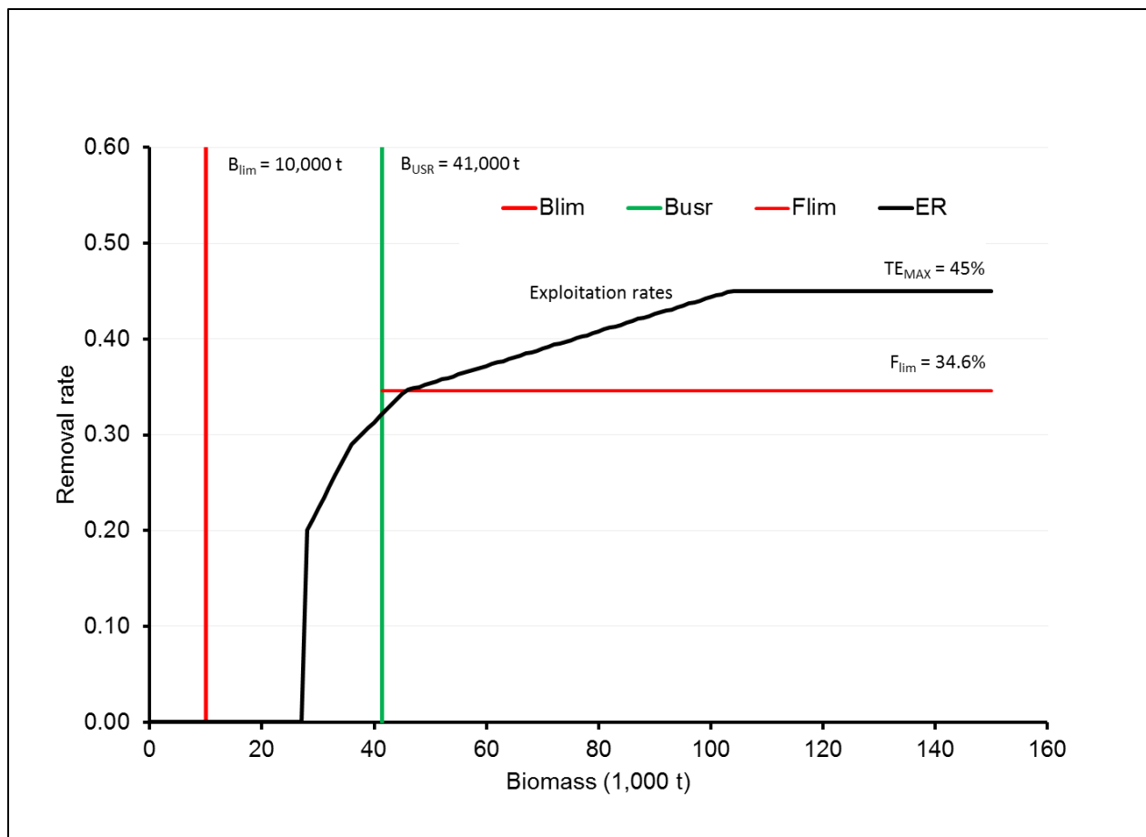
Figure 16. Harvest proportional decision rule (variant 4) compliant with the precautionary approach for the southern Gulf of St. Lawrence snow crab ( Chionoecetes opilio ) fishery (DFO 2014b). B_{lim} = The limit reference point for biomass; F_{lim} = Fishing removal rate limit reference point; B_{USR} = The upper stock reference point; ER = The exploitation rates based on the proportional harvest decision rule (variant 4).
