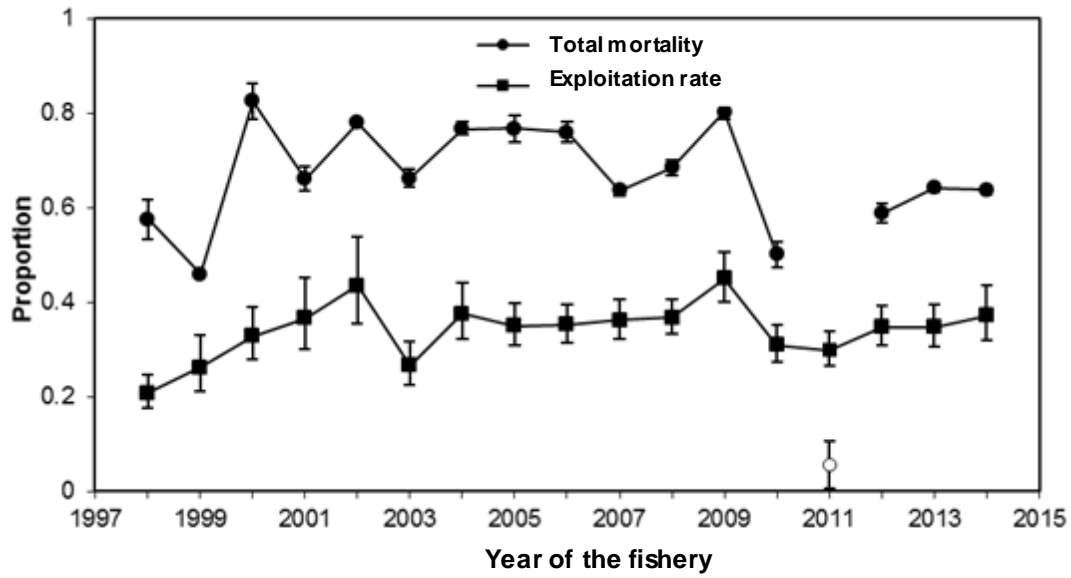
Figure 9. Estimated annual rates of exploitation and total loss of commercial-sized adult male snow crab ( Chionoecetes opilio ) in the southern Gulf of St. Lawrence, 1997 to 2014. The 2011 total mortality value is not reliable (Hébert et al. 2012).
