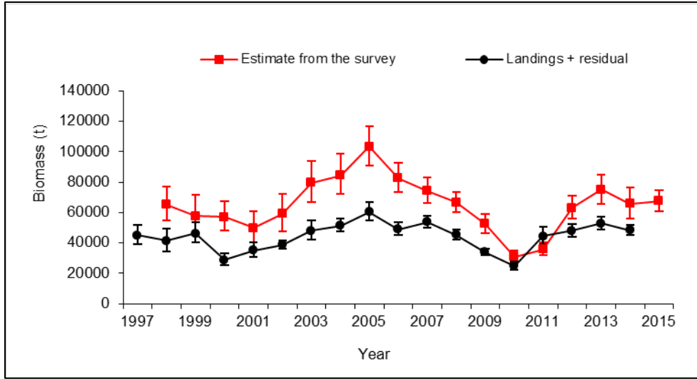
Figure 10. Comparison of the post-fishery calculated biomass ( t ; residual biomass plus the landings in year t+1 ) and the pre-fishery commercial-sized adult male snow crab ( Chionoecetes opilio ) biomass ( t ; recruitment plus residual biomass in year t ) estimated from the trawl survey in the southern Gulf of St. Lawrence.
