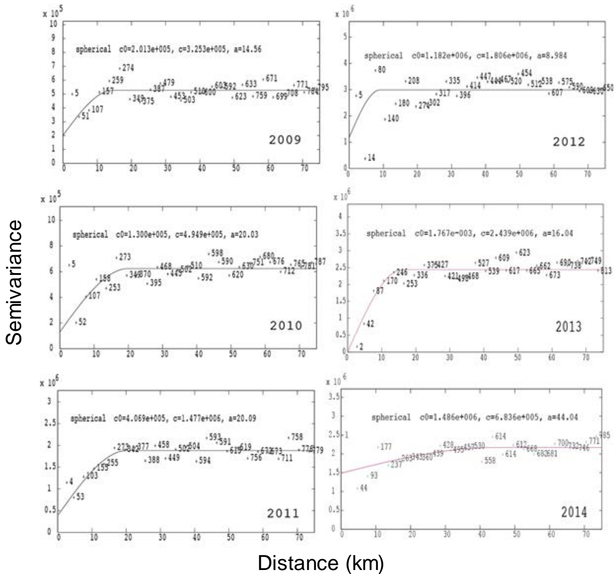
Figure 5. Annual variogram models for commercial-sized adult male snow crab ( Chionoecetes opilio ) in the southern Gulf of St. Lawrence, 2009 to 2014. Indicated is the number of paired observations used per distance lag semi-variance calculation.
