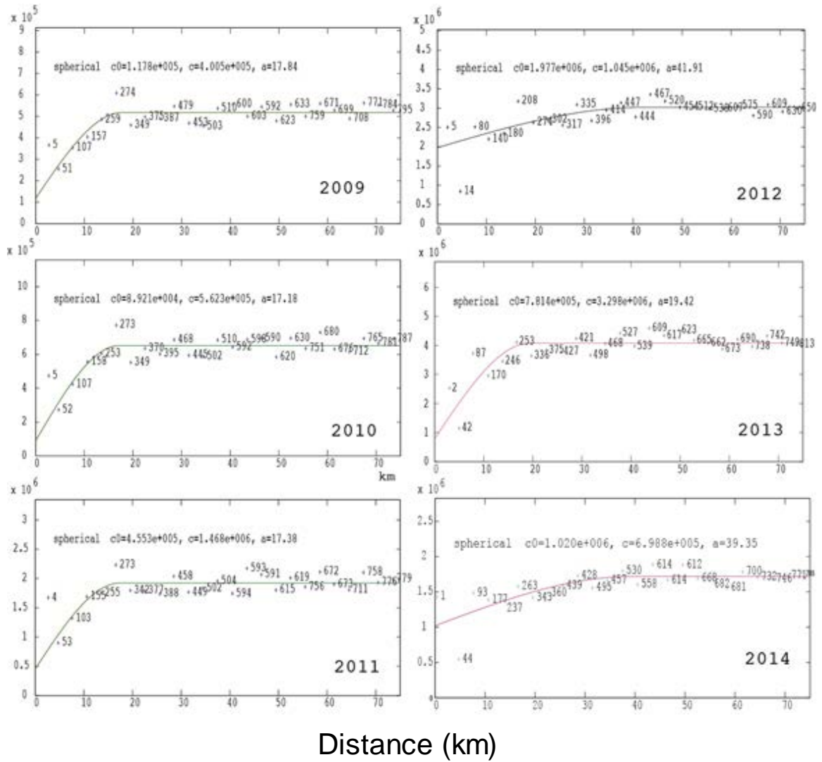
Figure 4. Three-year moving average variogram models for commercial-sized adult male snow crab ( Chionoecetes opilio ) in the southern Gulf of St. Lawrence, 2009 to 2014. Indicated is the number of paired observations used per distance lag semi-variance calculation.
