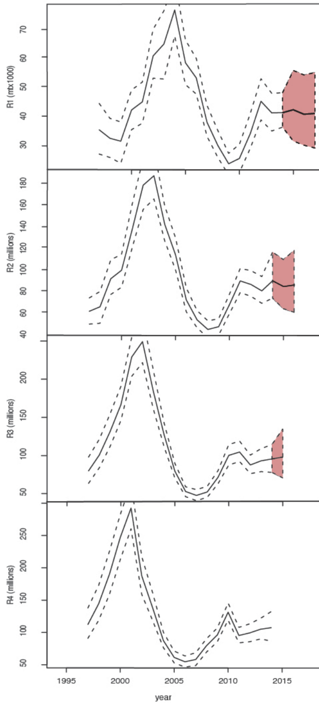
Figure 15. Snow crab ( Chionoecetes opilio ) recruitment ( R ) abundance (mean with 95% confidence intervals) by pre-recruit stages ( R_j ), where j=1, \dots, 4 years until recruitment to the fishery based on the survey data estimates. Shaded areas are forecasted abundance from the Bayesian model (Surette and Wade 2006).
