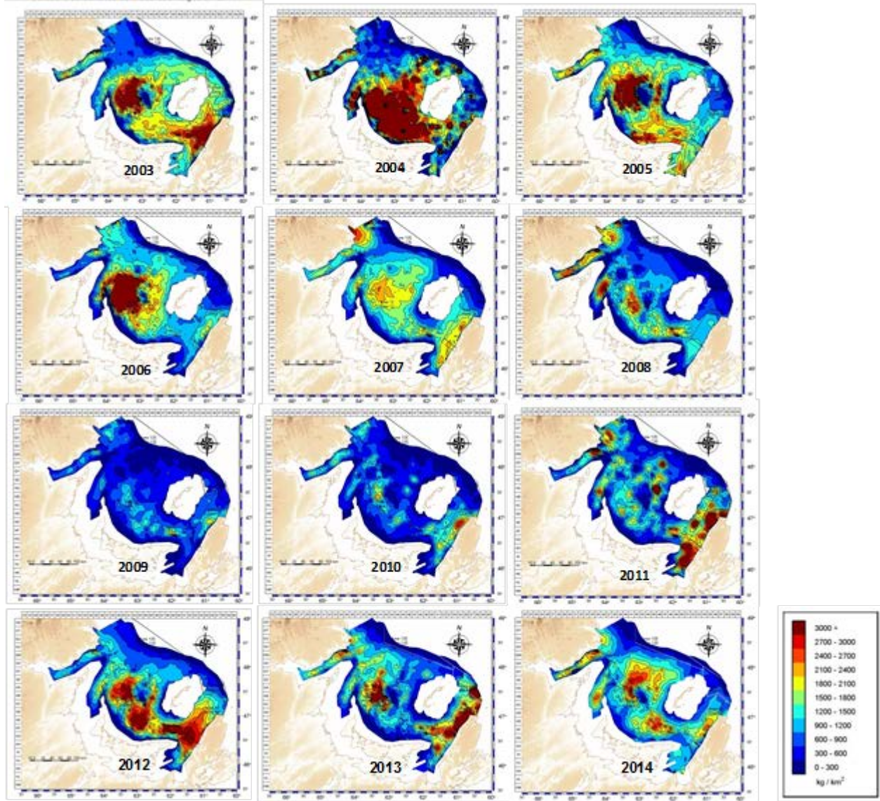
Figure 6. Density (kg per km 2 ) contours of commercial-sized ( \geq 95 mm of carapace width) adult male snow crab ( Chionoecetes opilio ) based on trawl survey data in the southern Gulf of St. Lawrence, 2003 to 2014.
