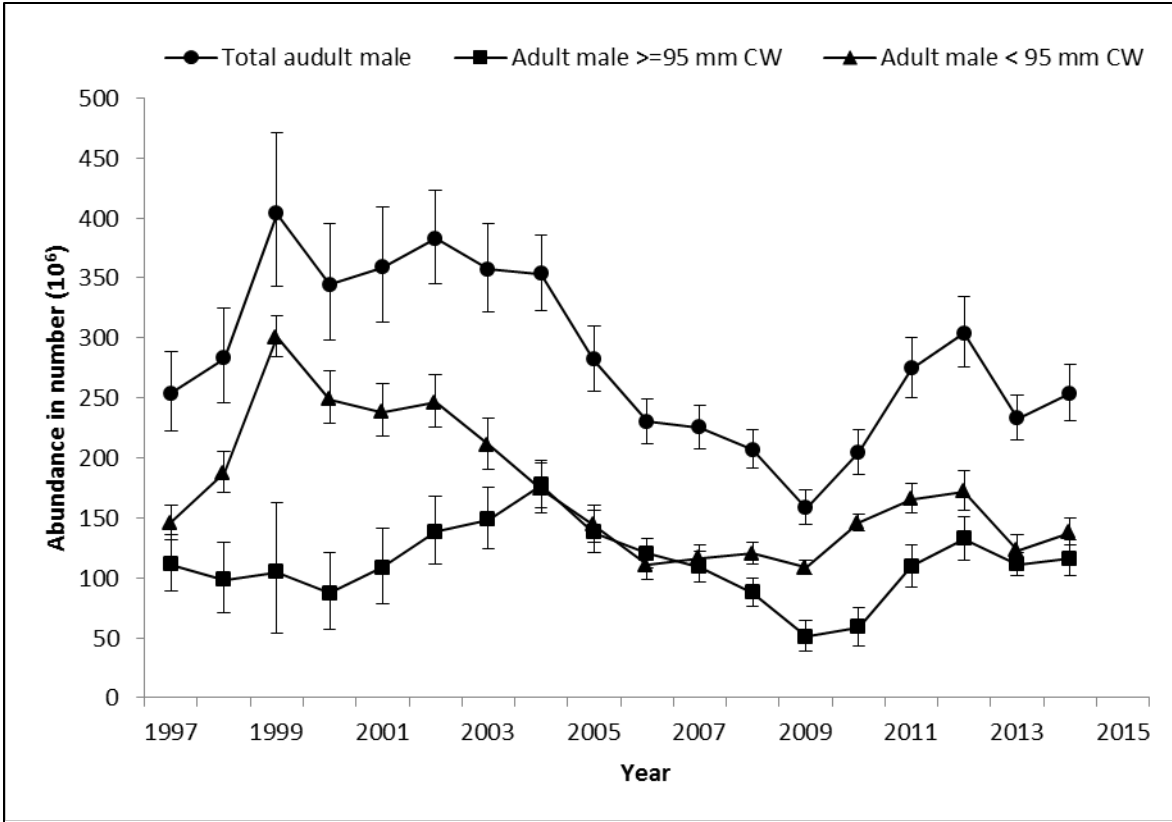
Figure 11. Estimated abundance (number in millions) of snow crab ( Chionoecetes opilio ) adult males in the southern Gulf of St. Lawrence, 1997 to 2014. CW = Carapace width.
