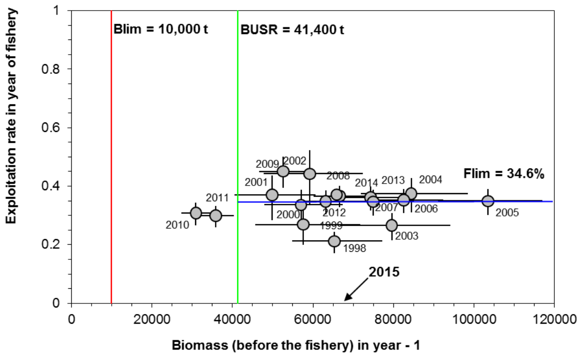
Figure 14. Trajectory of stock abundance (biomass of commercial-sized adult male snow crab ( Chionoecetes opilio ) as estimated from the trawl survey in year t - 1 versus exploitation rate of this biomass in the fishery of year t . Year of the fishery is labelled on the figure. B_{lim} = The limit reference point for biomass; F_{lim} = Fishing removal rate limit reference point; B_{USR} = The upper stock reference point.
