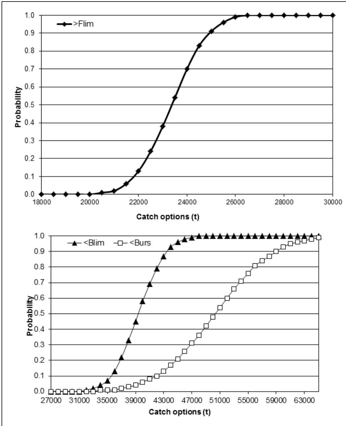
Figure 17. Risk analysis of catch options ( t ) for the 2015 fishery based on the expanded polygon for the southern Gulf of St. Lawrence snow crab, Chionoecetes opilio , showing probabilities of exceeding the fishing removal rate limit reference point ( F_{lim} ), of the hard-shelled commercial-sized adult male remaining biomass in 2015 falling below the limit reference point for biomass ( B_{lim} ) and of the commercial-sized adult male biomass in 2015 will be below the upper reference point ( B_{USR} ) after the 2015 fishing season.
