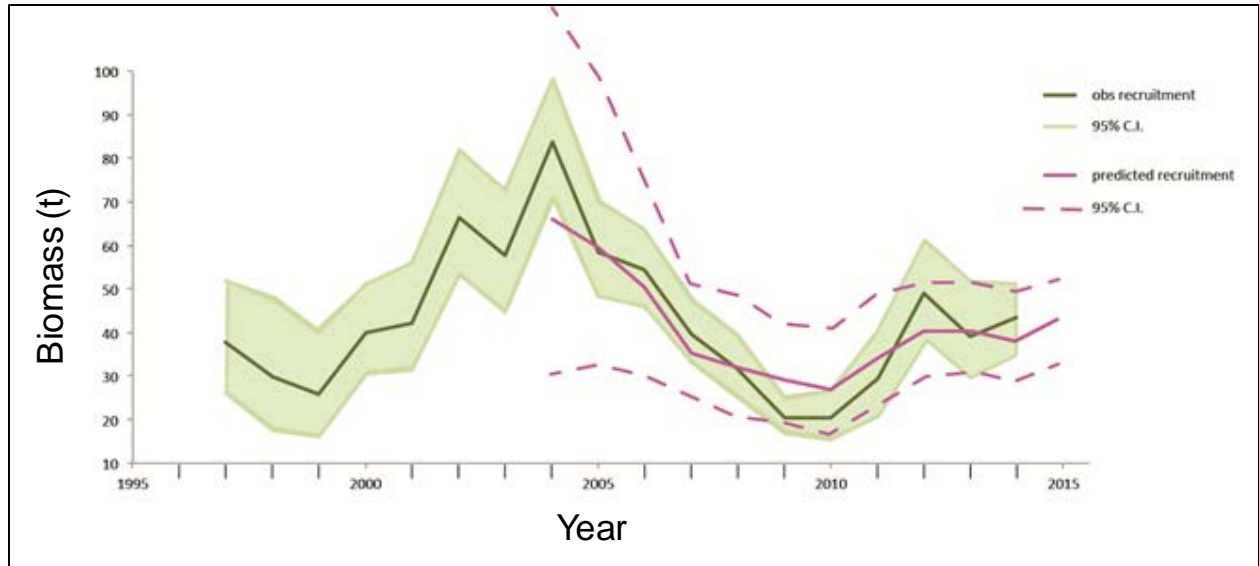
Figure 7. Comparison between the observed (mean with 95% confidence intervals) and predicted (mean with 95% confidence intervals) recruitment ( R-1 ) of male snow crab ( Chionoecetes opilio ) based on the Bayesian model on prerecruits (Surette and Wade 2006; Wade et al. 2014).
