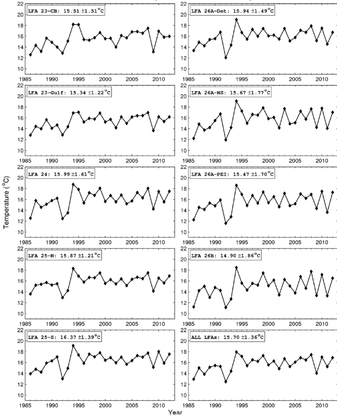
Figure 15. Time series of Sea Surface Temperature in July for each Lobster Fishing Area (LFA).
