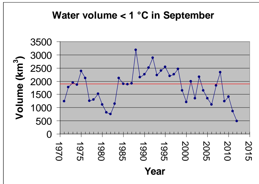
Figure 10. Cold Intermediate Layer volume ( T < 1^{\circ}\text{C} ) over the southern Gulf of St. Lawrence for September from 1971 to 2012.
