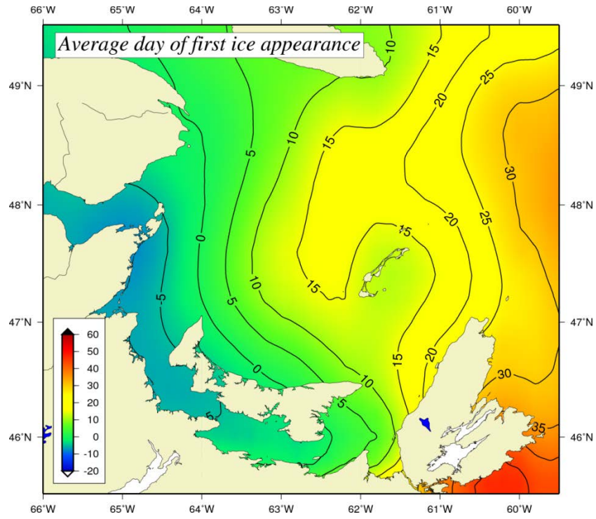
Figure 5. Average day of the year of the first ice appearance (1971-2000 climatology).
