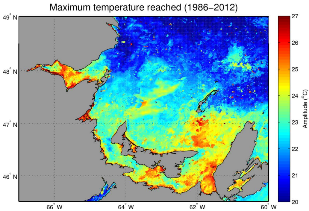
Figure 13. Highest Sea Surface Temperature recorded from 1986 to 2012 in the southern Gulf of St. Lawrence.
