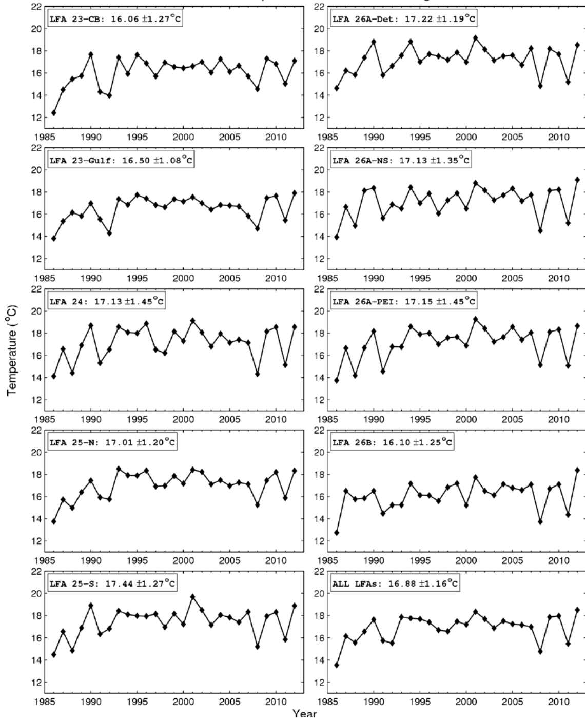
Figure 16. Time series of Sea Surface Temperature in August for each Lobster Fishing Area (LFA).
