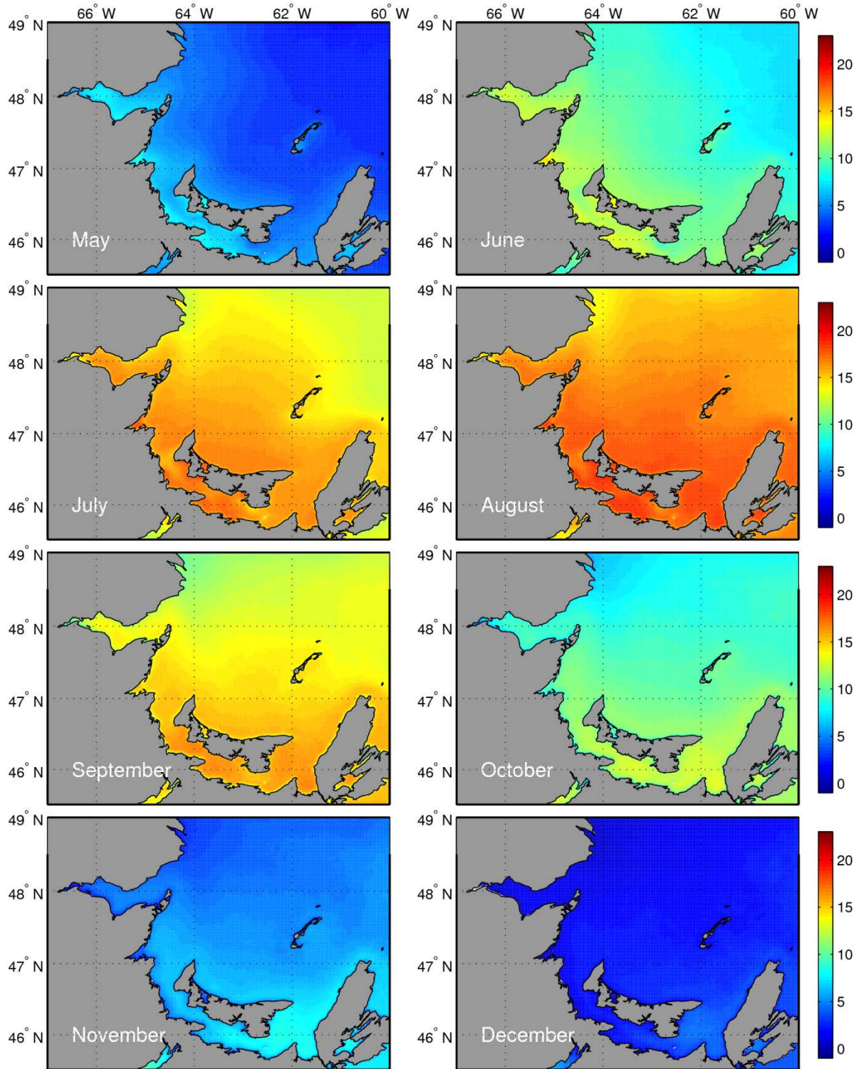
Figure 11. Sea Surface Temperature (SST) climatology (1986-2012) from May to December obtained from Institut Maurice-Lamontagne remote sensing laboratory.
