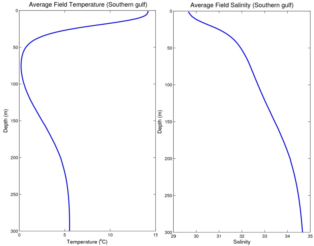
Figure 9. Average temperature (left) and salinity (right) profiles between 1971 and 2010 for September in the southern Gulf of St. Lawrence.
