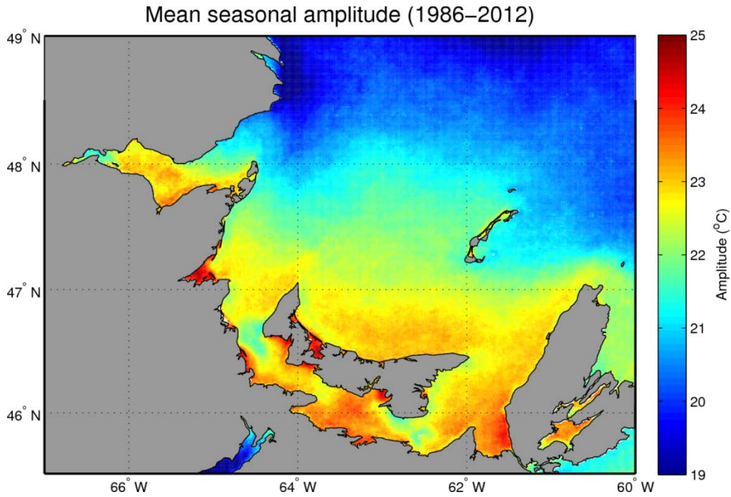
Figure 12. Average (1986-2012) seasonal amplitude of the sea surface temperature cycle.
