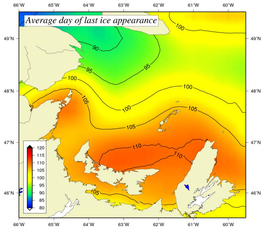
Figure 6. Average day of the year of the last ice appearance (1971-2000 climatology).
