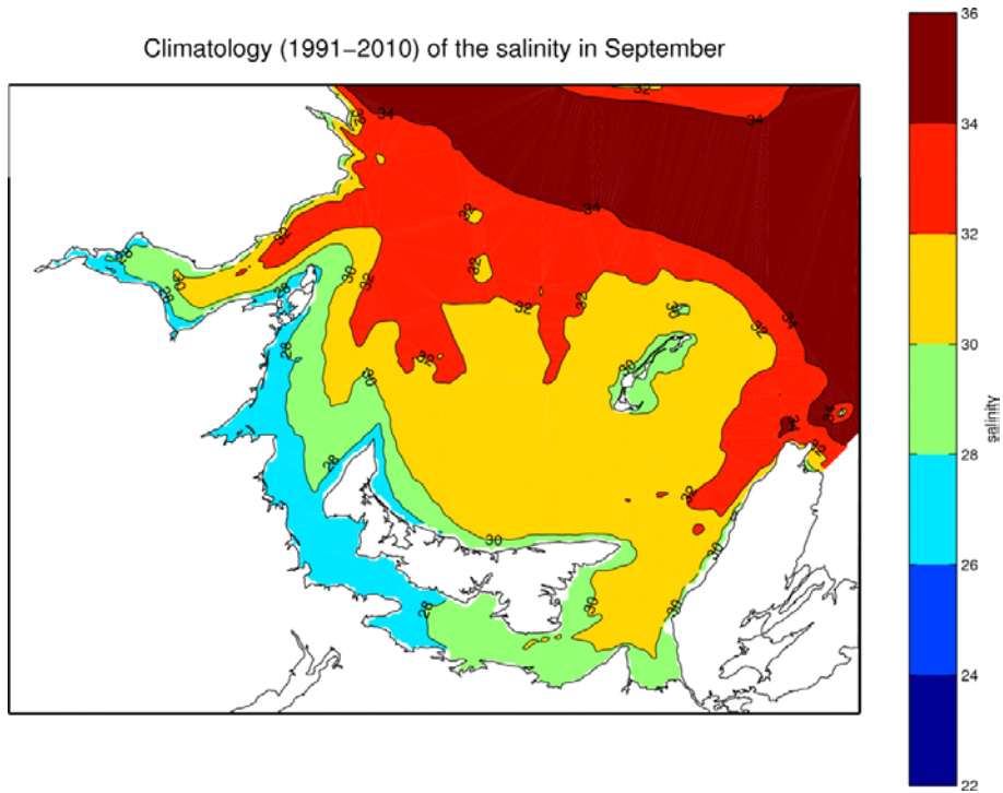
Figure 26. Average bottom water salinity (psu) in September between 1991 and 2010 for the southern Gulf of St. Lawrence.
