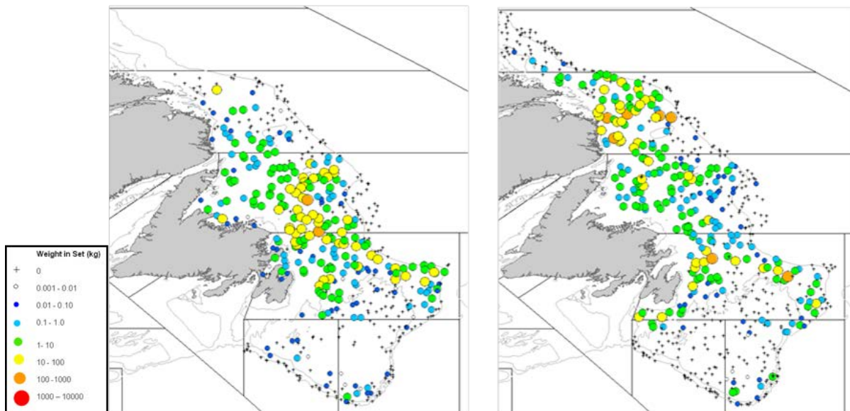
Figure 2. Distribution of capelin catch in the Campelen trawl during fall multi-species bottom trawl survey in 1995 (left) and 2012 (right). Symbol size is proportional to catch rates (kgs per standard tow).
