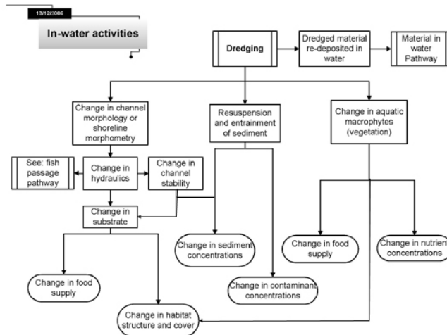
Figure 1: Pathway of Effects diagram established by DFO by expert consultation for evaluation of dredging activities.
