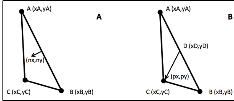
Figure B.1. Structure of the element defined by the nodes A (x_A, y_A) , B (x_B, y_B) and C (x_C, y_C) and vectors used to calculate the flow through the link A-B. For panel A (left panel), the vector (n_x, n_y) originates at the bisection of link A-B and is oriented perpendicular to A-B. For panel B (right panel), the vector (p_x, p_y) originates at the bisection of the link A-B and D (x_D, y_D) , and is directed to the node that opposes A-B, C ( x_C, y_C ).
