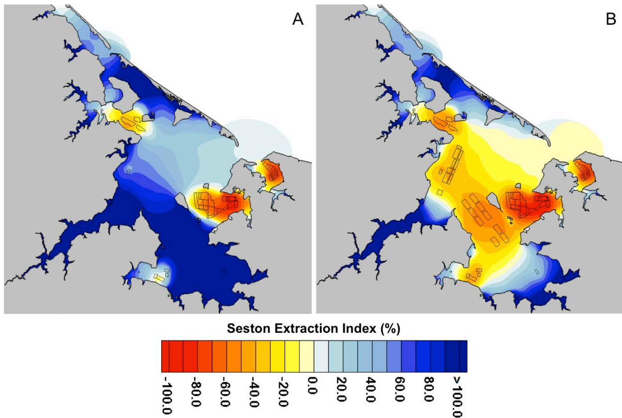
Figure 4. Seston Extraction Index (SEI, %) for current leases (A, left panel) and current leases plus projected leases (B, right panel).
