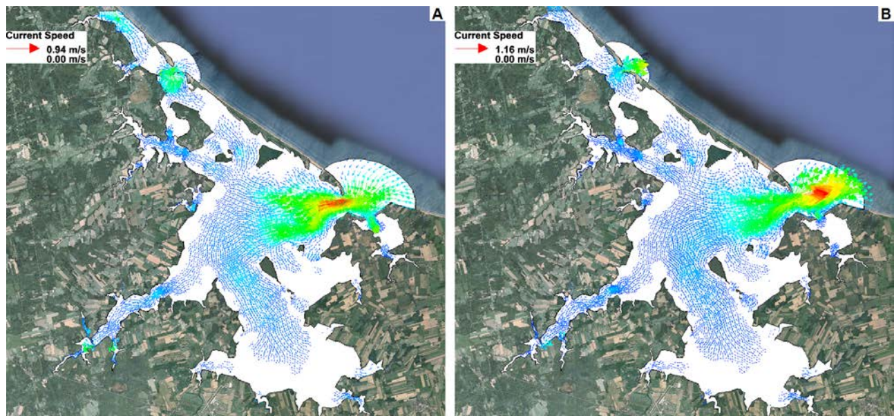
Figure A.2. Map of tidal currents predicted in Malpeque Bay at a) maximum flood (left panel) and b) maximum ebb (right panel).
