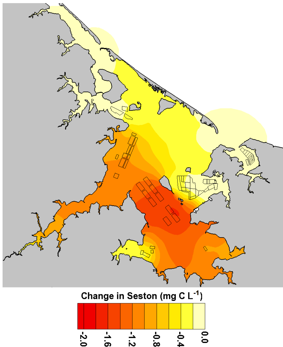
Figure 5. Absolute change in organic seston concentration in the projected scenario compared to the current scenario.
