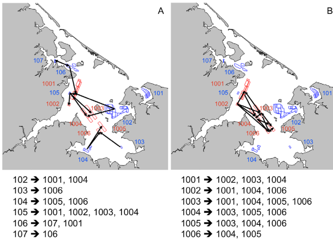
Figure 3. The most significant inter-lease connections from current to other leases (A, left panel) and from projected leases to leases (B, right panel). These connections are identified in each panel for clarification.
