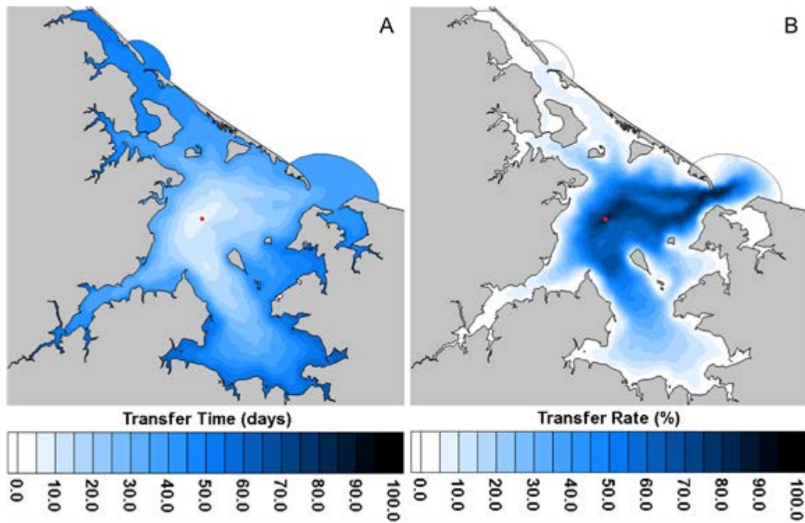
Figure 2. Transfer time (left panel, A) and transfer rate (right panel, B) between element #1004 (in red) and all other elements of the grid.
