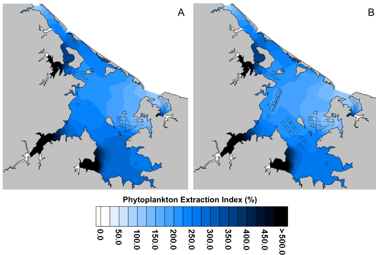
Figure 6. Phytoplankton Extraction Index (PEI, %) for current leases (A, left panel) and current leases plus projected leases (B, right panel).
