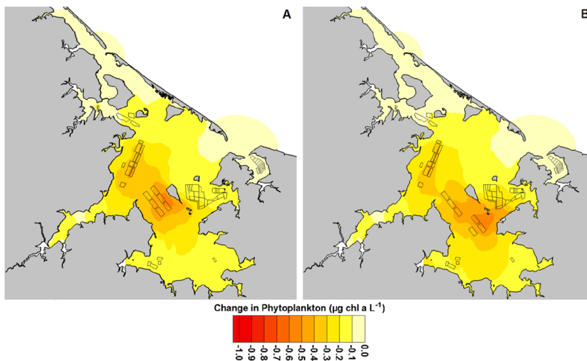
Figure 8. Absolute change in phytoplankton concentration in projected scenario (A, left panel) without leased areas #1005 and #1006, and (B, right panel) without leased area #1003, compared to the current scenario.
