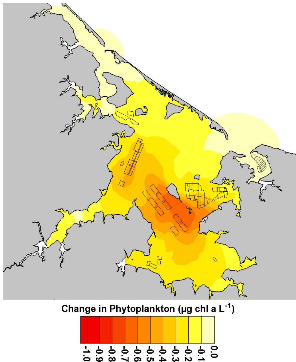
Figure 7. Absolute change in phytoplankton concentration in the projected scenario compared to the current scenario.
