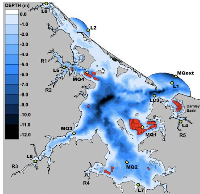
Figure C.1. Map of Malpeque, including bathymetry, current leases (red polygons), sampling stations (MQ1, MQ2, MQ3, MQ4 and MQext), rivers (R1, R2, R3, R4 and R5), and hydrodynamic stations (L1, L2, LC3, L4, L5, L6, L7 and L8. L = Water level. C = Current meter).
