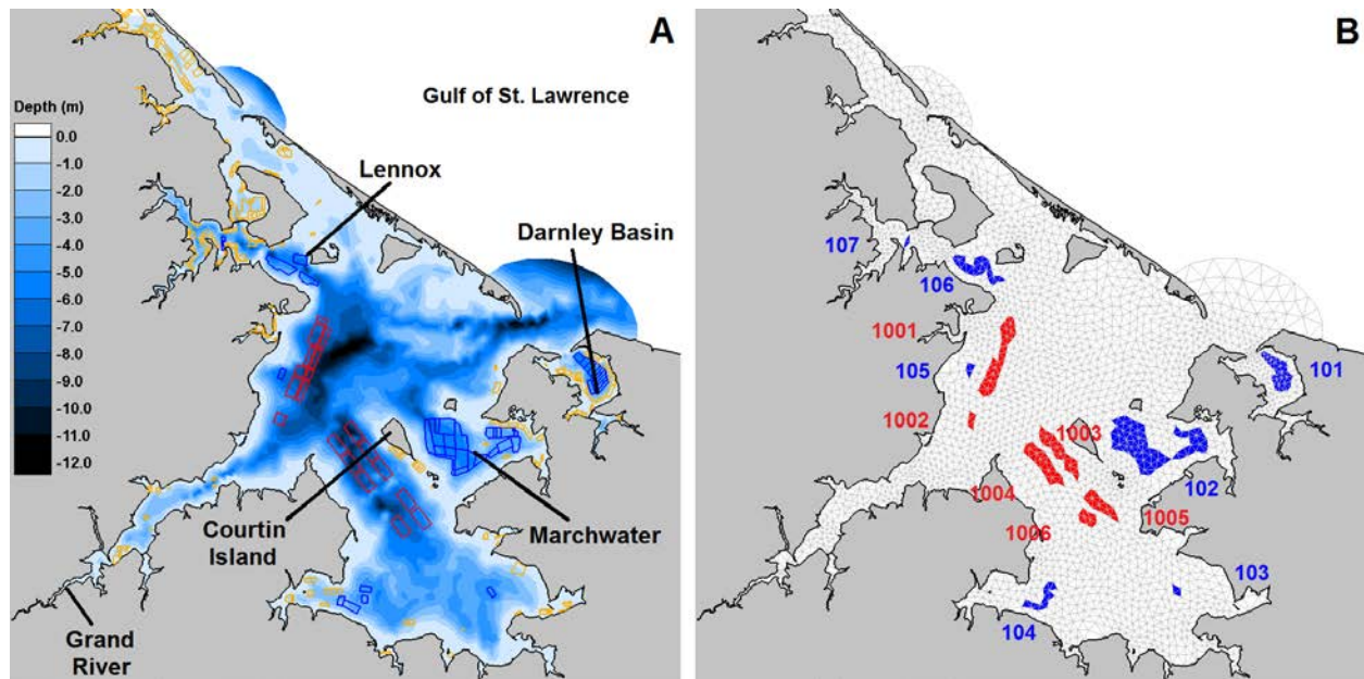
Figure 1. A (left panel). Water depth, current and new mussel leases (blue and red polygons respectively), as well as oyster leases (orange). B (right panel). Triangular mesh used in the modelling exercises and current and future mussel cultivation areas, blue and red, respectively. Cultivation areas have been coded to facilitate the description of the results.
