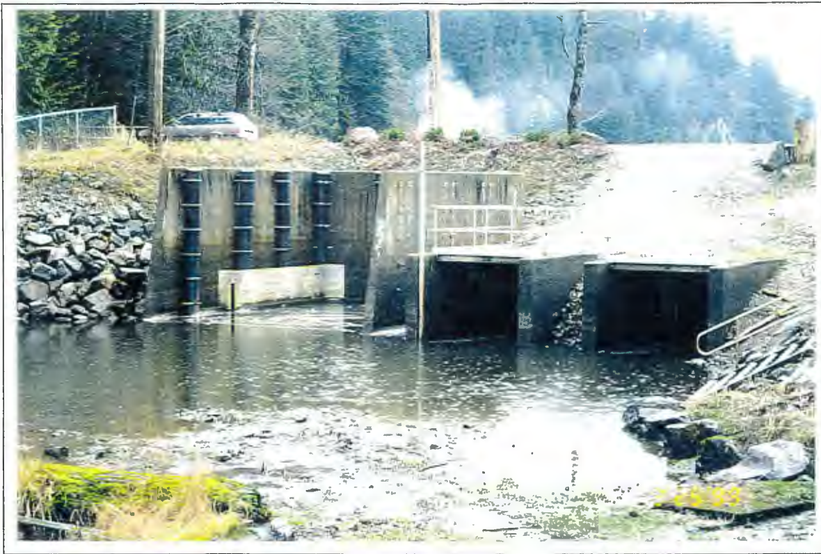
Photo 11: Miami Creek station: flood box entrance (R), future pump house sump (L)
