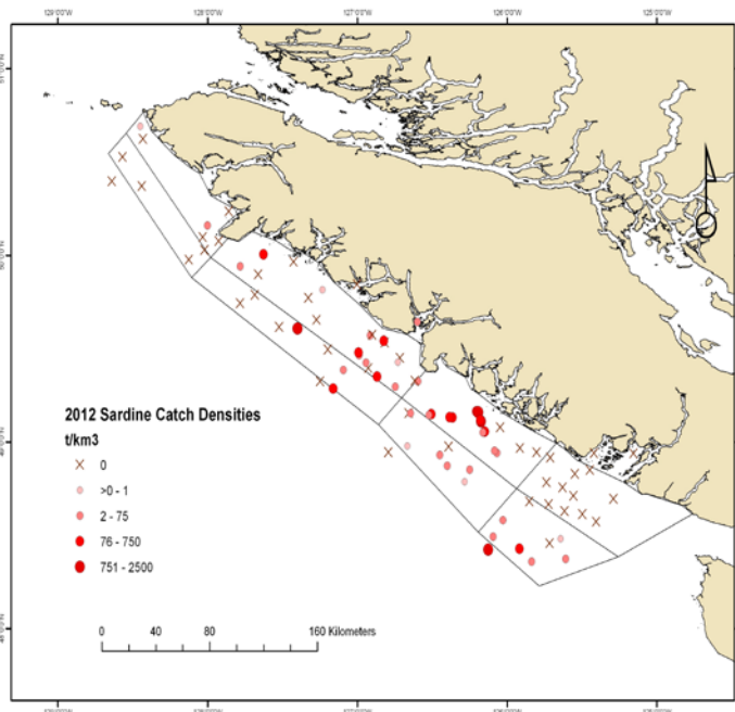
Figure 1. Sardine catch densities (tonnes/km 3 ) for the 2012 WCVI trawl survey). The core survey region is delineated by the outer bounds of the 8 sub regions zones shown above.
