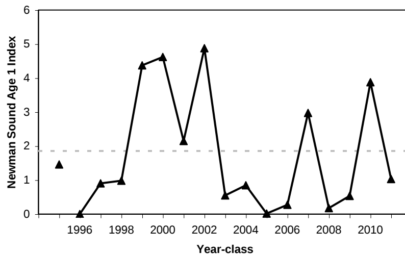
Figure 16. Trends in the numbers of age 1 cod from beach seine surveys in Newman Sound. Series mean is plotted as dashed line.
