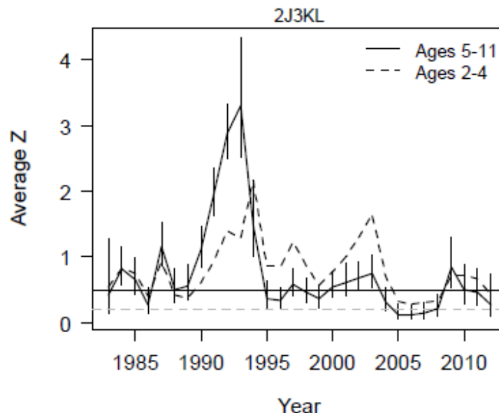
Figure 12. Trends in total mortality rates ( Z ) for two age groups of cod estimated from cohort analysis of autumn RV survey data. The horizontal lines indicate values of Z=0.5 (solid line) and Z=0.2 (grey dashed line) which correspond to annual mortality rates of 39 % and 18 %, respectively. Error bars are 95 % confidence intervals.
