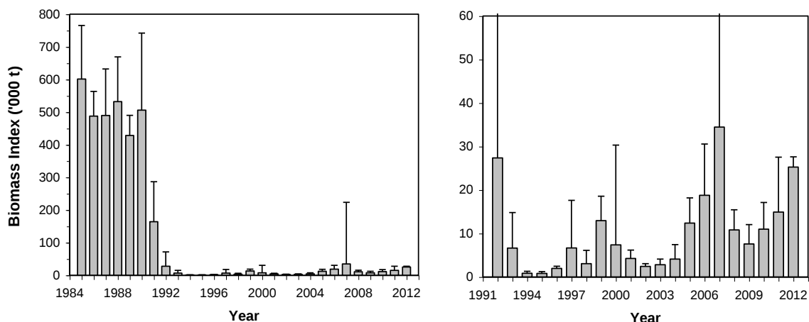
Figure 6. Offshore biomass index (+2 SE's) from spring RV surveys in Div. 3L. The right panel is expanded to show trends from 1992 onwards.
