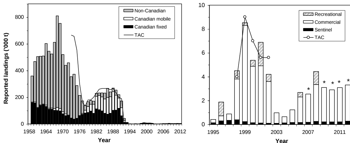
Figure 2. Total Allowable Catches (TACs) and landings (thousands of tons) in 1959-2012. The right panel is expanded to show trends from 1995 onwards. Asterisks indicate that recreational catches in 2007 and 2009-2012 are unknown.
