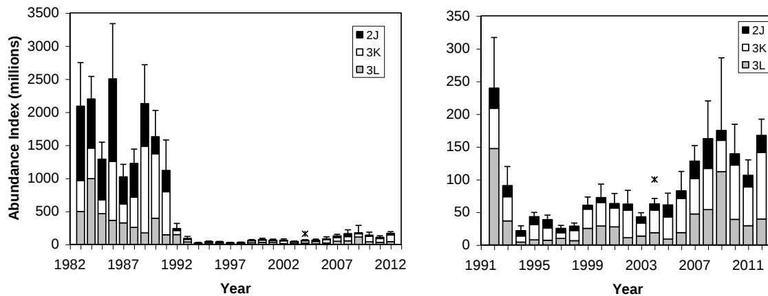
Figure 4. Offshore abundance index (+2 SE's) from autumn RV surveys in Div. 2J3KL. The right panel is expanded to show trends from 1992 onwards. Asterisks indicate partial estimates from incomplete survey coverage of Div. 3L in 2004.
