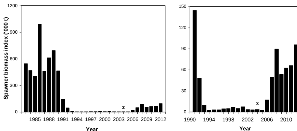
Figure 7. Offshore spawning stock biomass index from autumn RV surveys in Div. 2J3KL. The right panel is expanded to show trends from 1991 onwards. Asterisks indicate partial estimates from incomplete survey coverage of Div. 3L in 2004.
