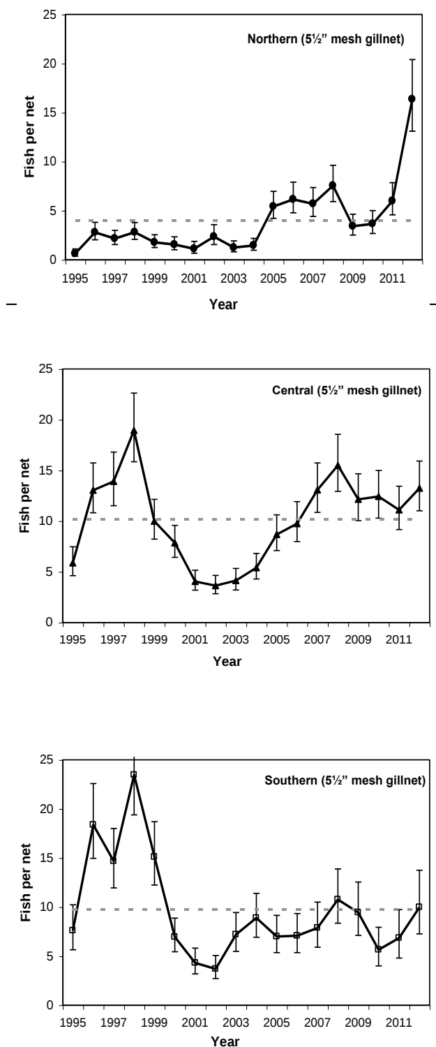
Figure 14. Standardized catch rates, with 95 % confidence limits, from sentinel surveys using gillnets (5.5" mesh) for each of the three inshore areas as depicted in Fig.3. Series means are plotted as dashed lines.
