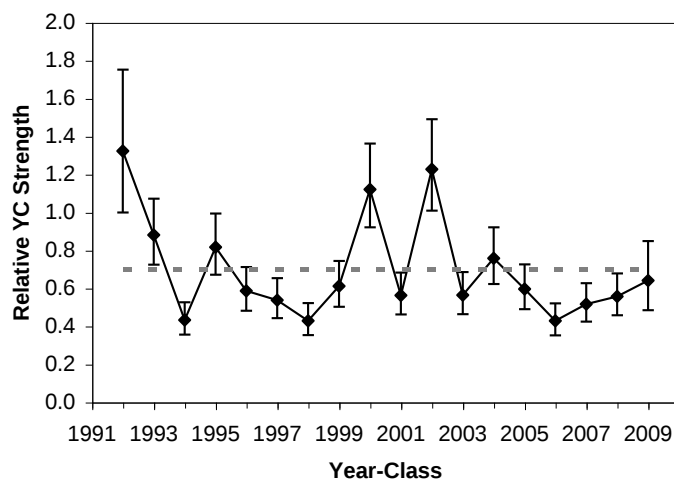
Figure 15. Standardized year class strength from sentinel survey catch rate data for ages 3 and 4 using 5½ inch and small mesh (3¼ inch) gillnets for the inshore central area. The dashed grey line is the time-series average.
