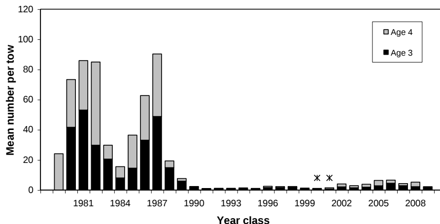
Figure 8. Abundance of the 1979-2009 year-classes at age 3 and age 4 in the offshore of Div. 2J3KL from the autumn RV surveys. Asterisks indicate partial estimates for the 2000 year-class at age 4 and the 2001 year-class at age 3 due to incomplete survey coverage of Div. 3L in 2004.
