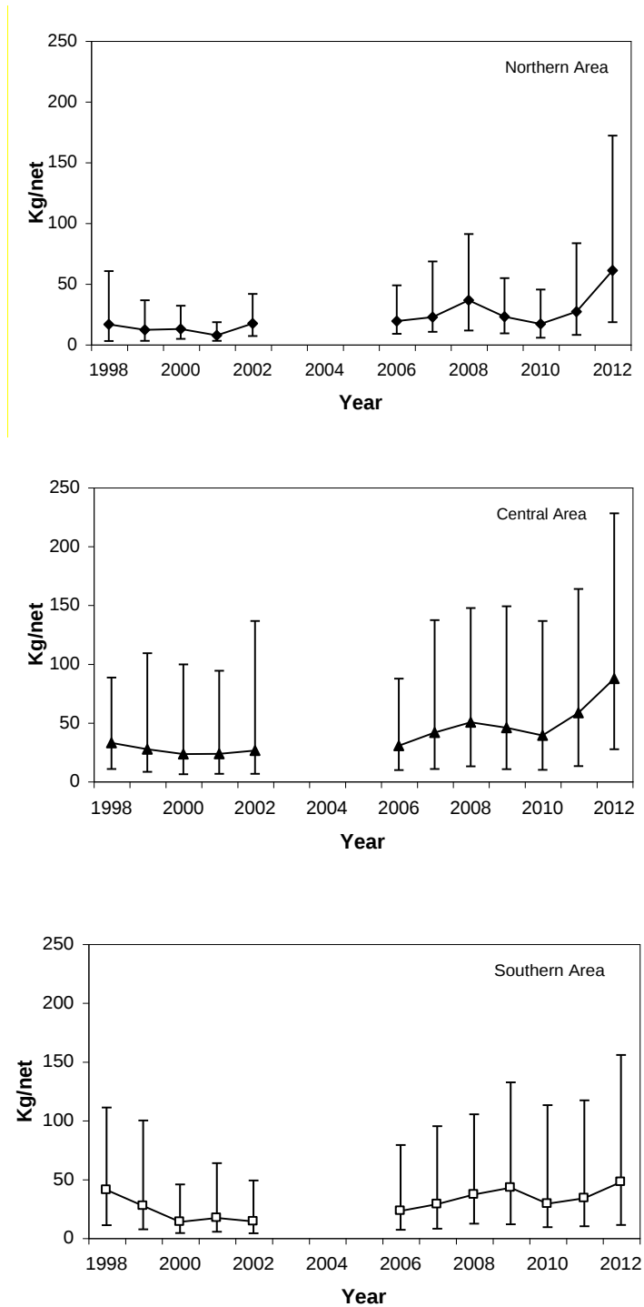
Figure 13. Median catch rates, with 10 th and 90 th percentiles, from log-books for the <35 ft vessel sector using gillnets in each of the three inshore areas in Fig.3. There was no directed fishery in 2003-2005.
