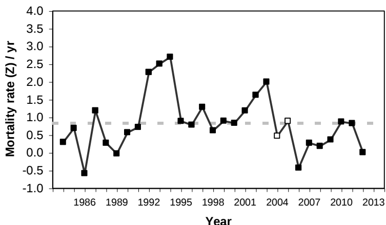
Figure 9. Trends in total mortality rate ( Z ) of cod aged 4-6 calculated using data from autumn RV surveys in the offshore of Div. 2J3KL. For example, the value in 1996 is the mortality experienced by the 1991-1989 year-classes from ages 4-6 in 1995 to ages 5-7 in 1996. The dashed line is the time-series average ( Z = 0.84 which corresponds to 57 % mortality per year). Open symbols indicate estimates based on an incomplete survey in 2004.
