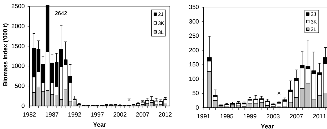
Figure 5. Offshore biomass index (+2 SE's) from autumn RV surveys in Div. 2J3KL. The right panel is expanded to show trends from 1992 onwards. Asterisks indicate partial estimates from incomplete survey coverage of Div. 3L in 2004.
