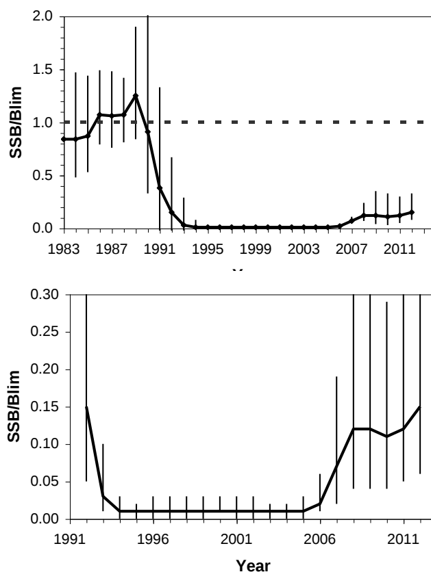
Figure 11. Trends in SSB relative to the LRP ( B_{lim} ) based on cohort analysis of autumn RV survey data. The upper panel shows the full time series (1983-2012) and the lower panel the more recent (1992-2012) period. Error bars are 95 % confidence intervals.
