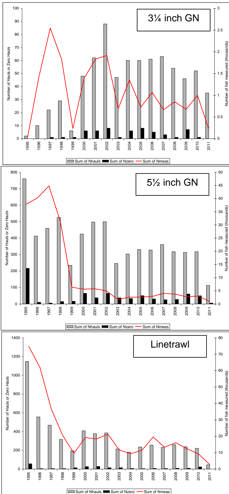
Figure 1. Summary information for Sentinel Survey activity in NAFO Subdivision 3Ps from 1995 to 2011. Nhaults= number of sets; Nzero= number of sets with no fish; Nmeas= number of fish measured. Data for 2011 are preliminary.
