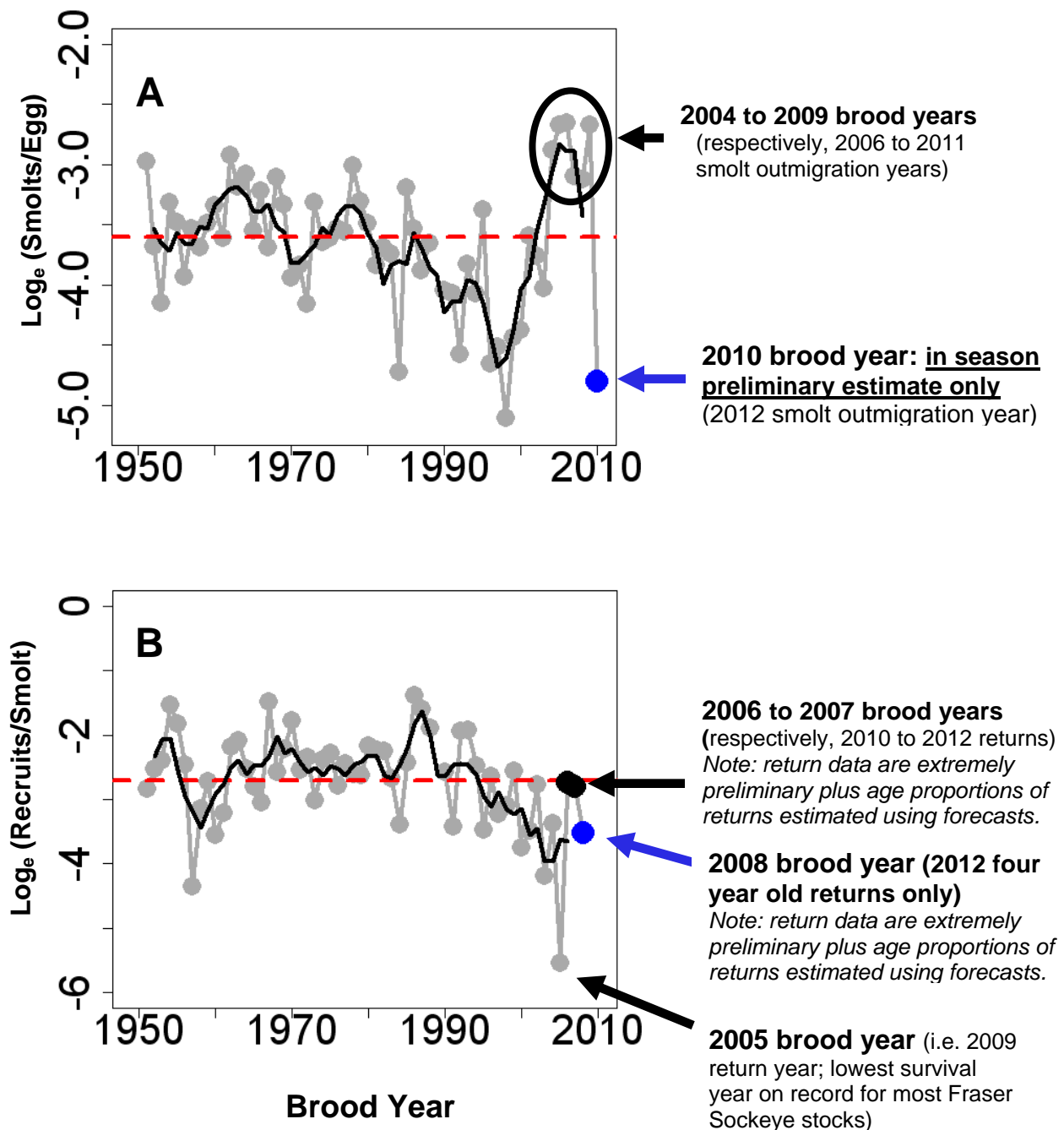
Figure 2. Chilkot River Sockeye A. freshwater ( \log_e smolts per egg) and B. marine ( \log_e recruits per smolt) annual survival (grey lines) and smoothed four-year running average survival (black lines). Red dashed lines in both plots indicate long-term average survival.
