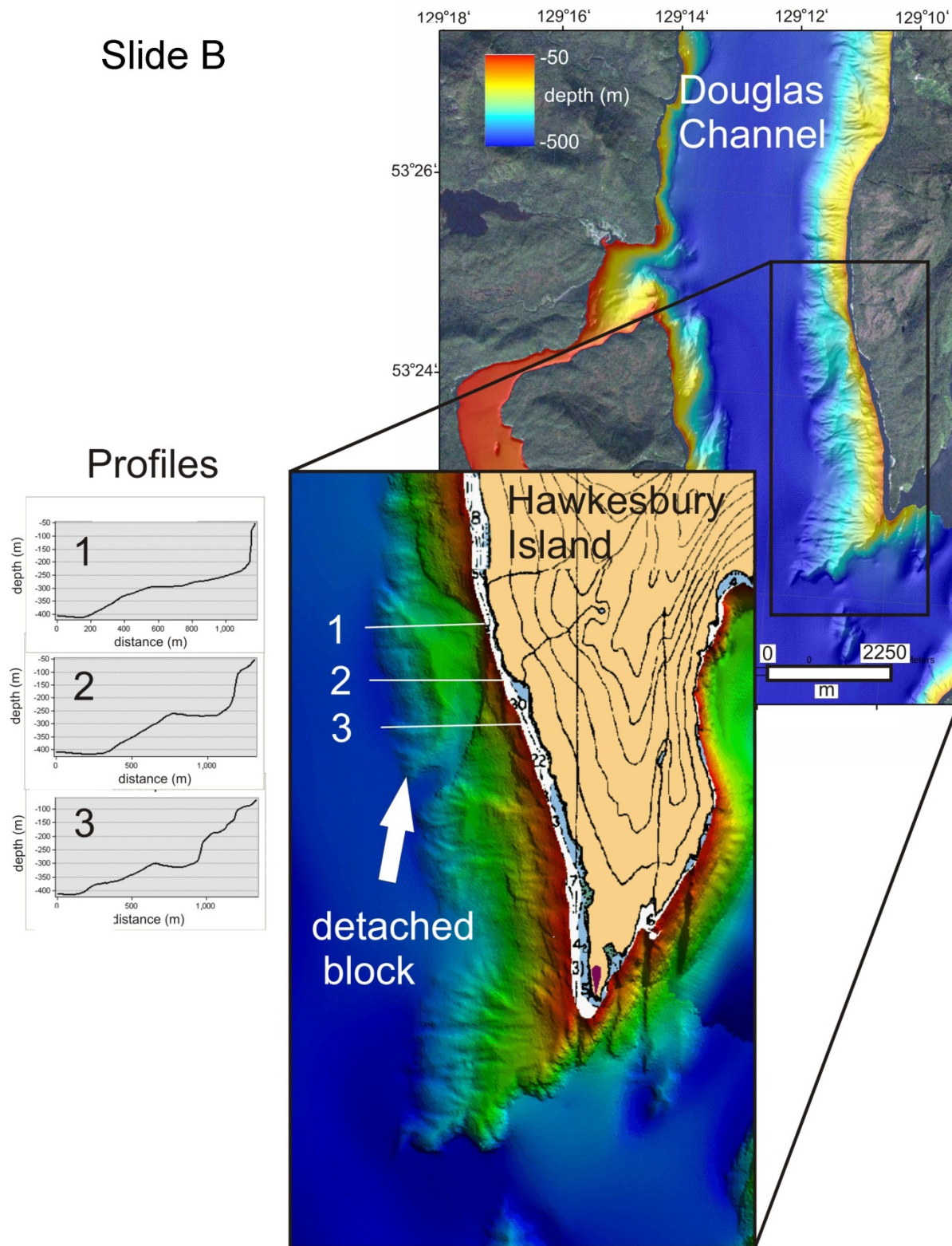
Figure 4 Detailed multibeam imagery of Slide B. Plotted to the left of each slide are numbered bathymetric profiles extracted from multibeam bathymetry; locations for each profile are shown in the slide image. From Conway et al. (2012).
