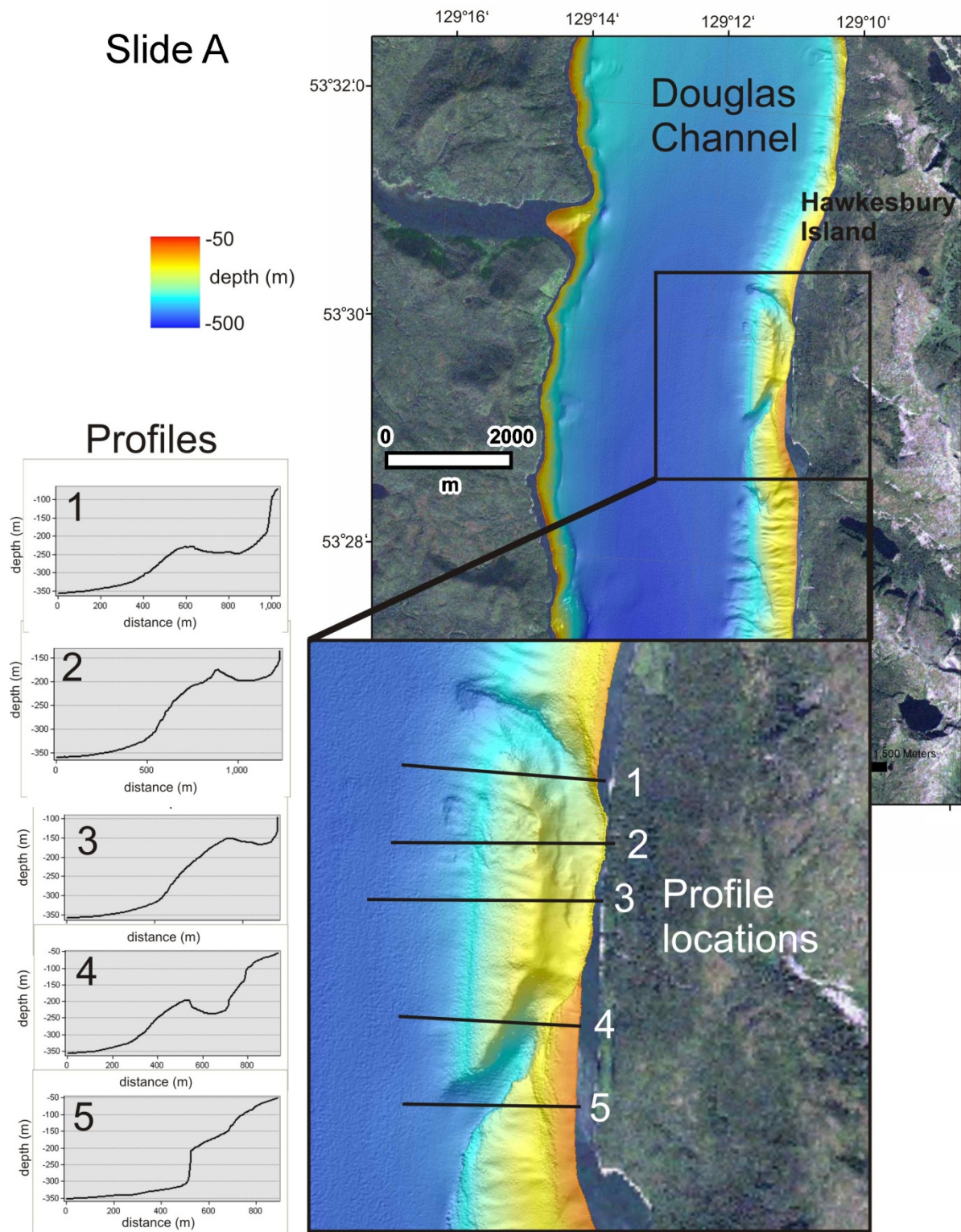
Figure 3. Detailed multibeam imagery of Slide A. Plotted to the left of each slide are numbered bathymetric profiles extracted from multibeam bathymetry; locations for each profile are shown in the slide image. From Conway et al. (2012).
