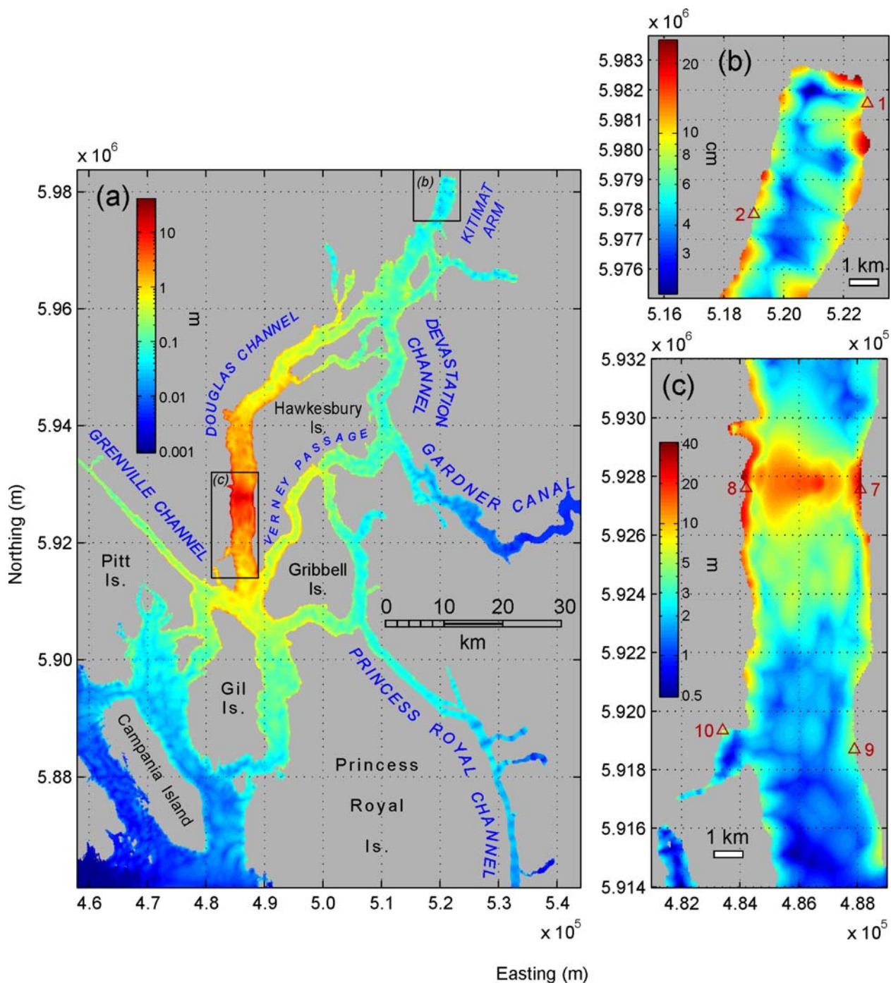
Figure 5 Maximum tsunami wave amplitudes generated by Slide A. Expanded regions are presented in (b) and (c); see (a) for locations. Note change in amplitude units in (b). From Thomson et al. (2012).
