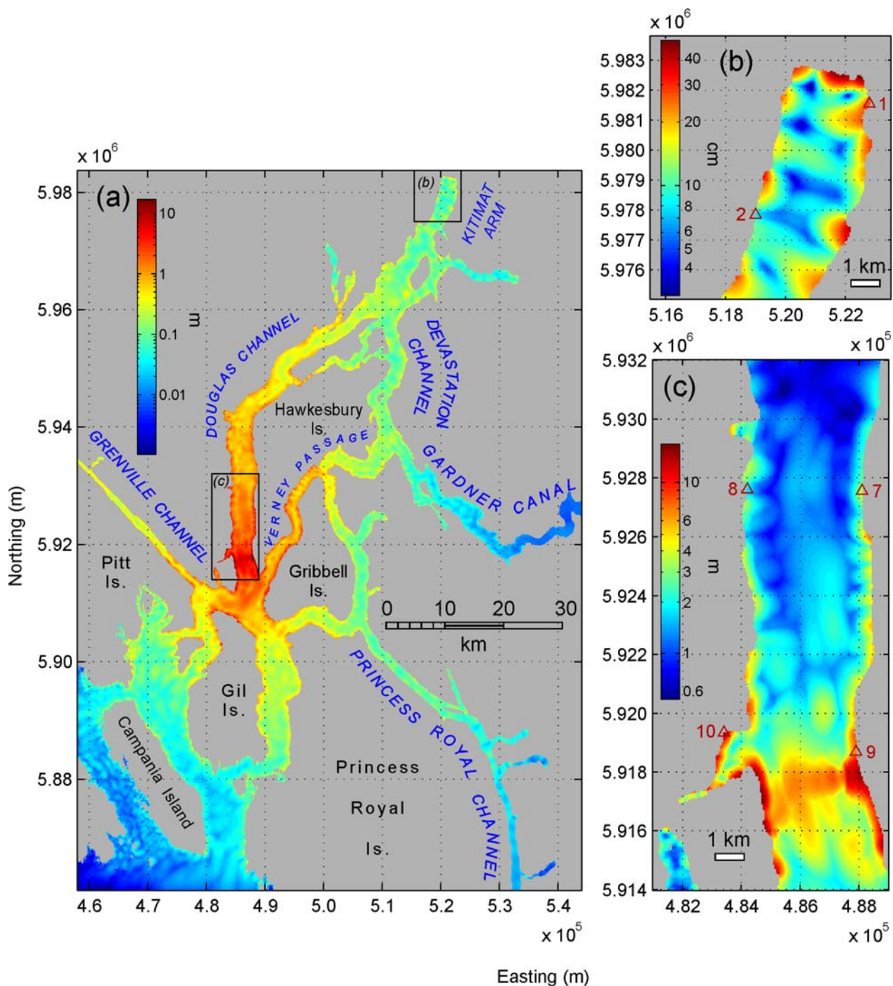
Figure 6 Maximum tsunami wave amplitudes generated by Slide B. Expanded regions are presented in (b) and (c); see (a) for locations. Note change in amplitude units in (b). From Thomson et al. (2012).
