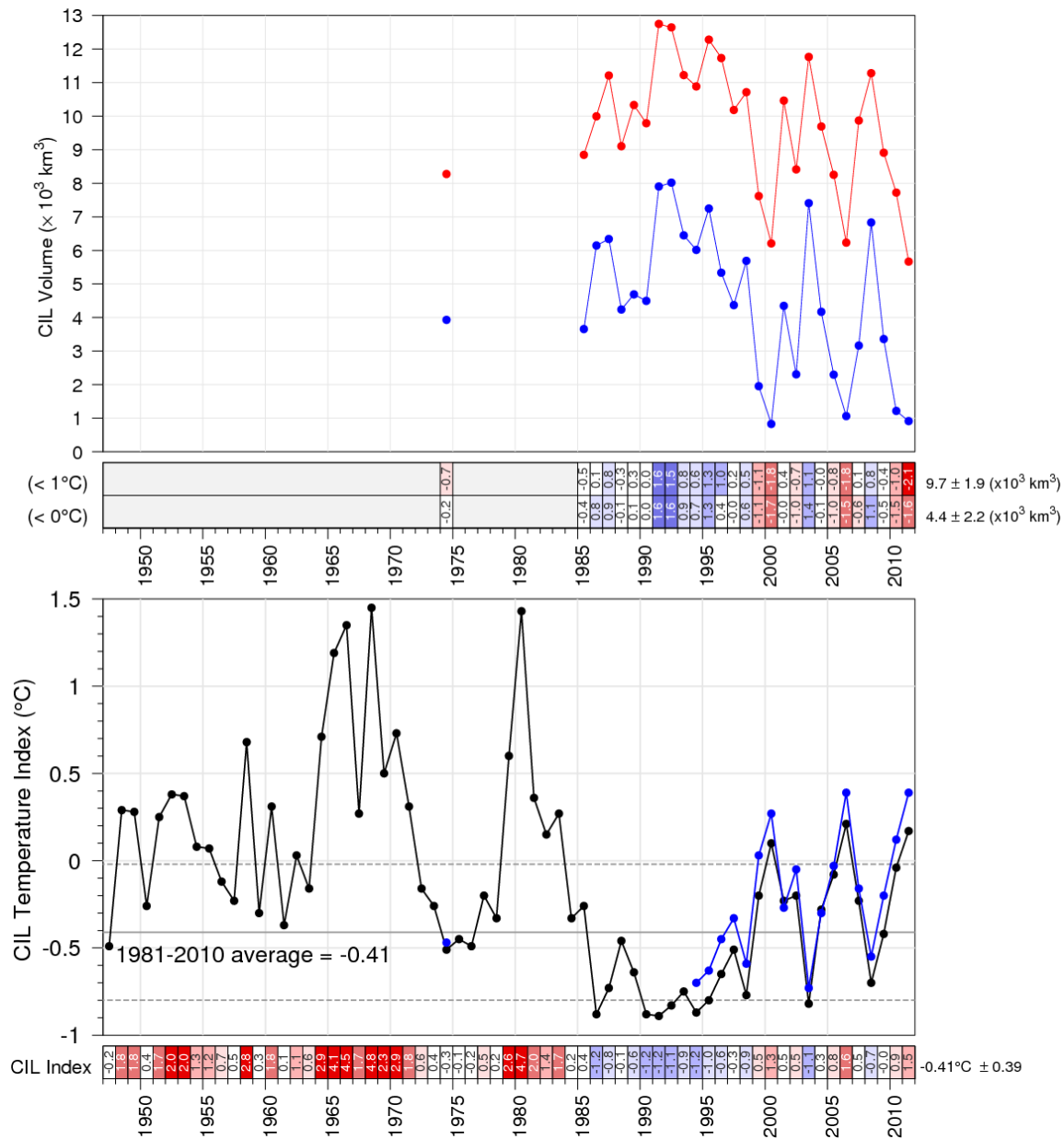
Fig. 29. CIL volume (top panel) delimited by the over- and underlying 0^{\circ}\text{C} (in blue) and 1^{\circ}\text{C} (in red) isotherms, and minimum temperature index (bottom panel) in the Gulf of St. Lawrence. The volumes are integrals of each of the annual interpolated thickness grids such as those shown in the top panels of Fig. 27. In the lower panel, the black line is the updated Gilbert and Pettigrew (1997) index interpolated to 15 July and the blue line is the spatial average of each of the annual interpolated grid such as those shown in the two bottom panels of Fig. 27. The numbers in the boxes are normalized anomalies.
