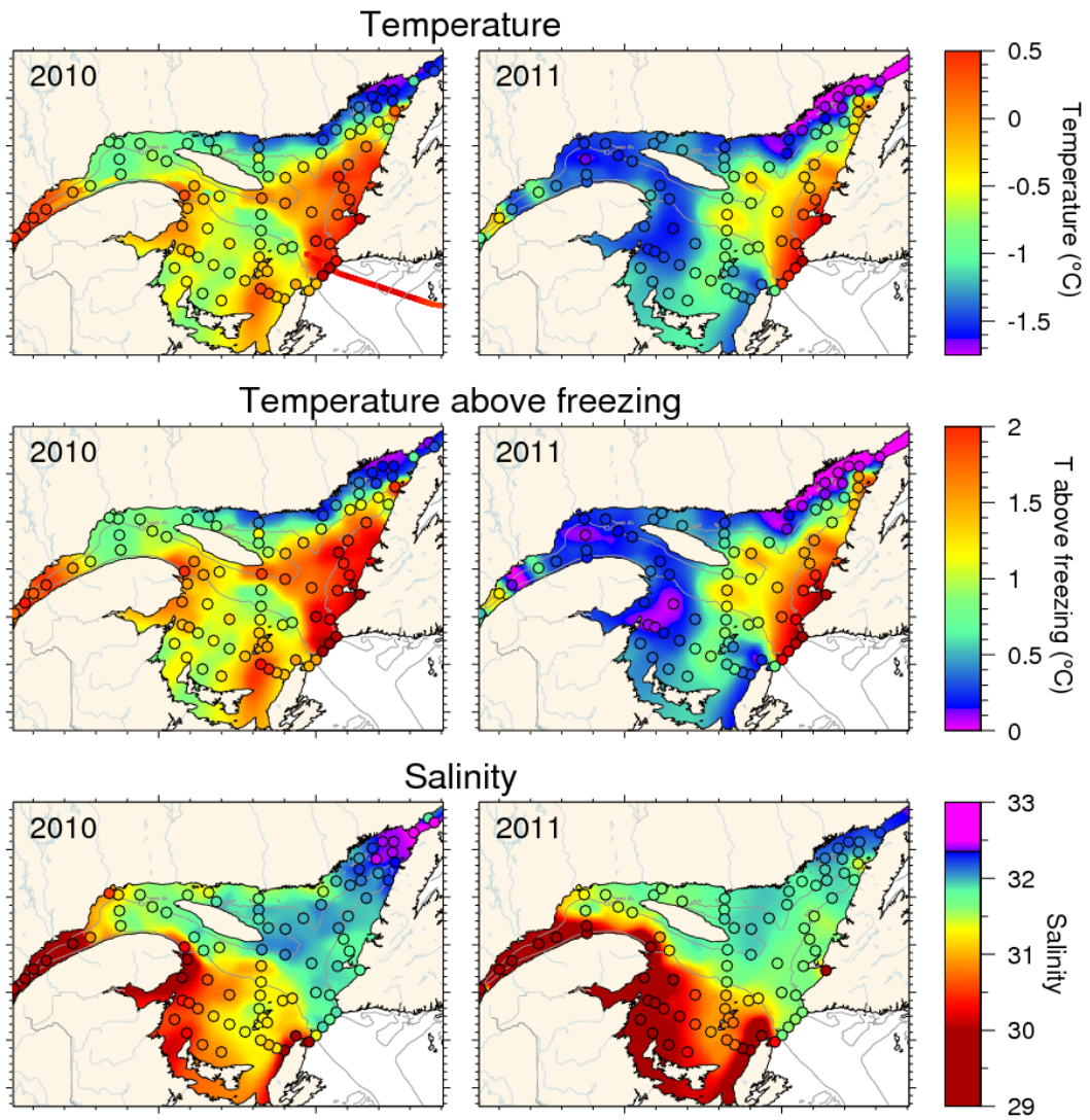
Fig. 23. Winter surface layer characteristics from the March 2010 and 2011 helicopter surveys: surface water temperature (upper panel), temperature difference between surface water temperature and the freezing point (middle panel), and salinity (lower panel). The temperature measurements from shipboard thermosalinographs taken during the 2010 survey are also shown in the upper panel. The symbols are coloured according to the value observed at the station, using the same colour palette as the interpolated image. A good match is seen between the interpolation and the station observations where the station colours blend into the background.
