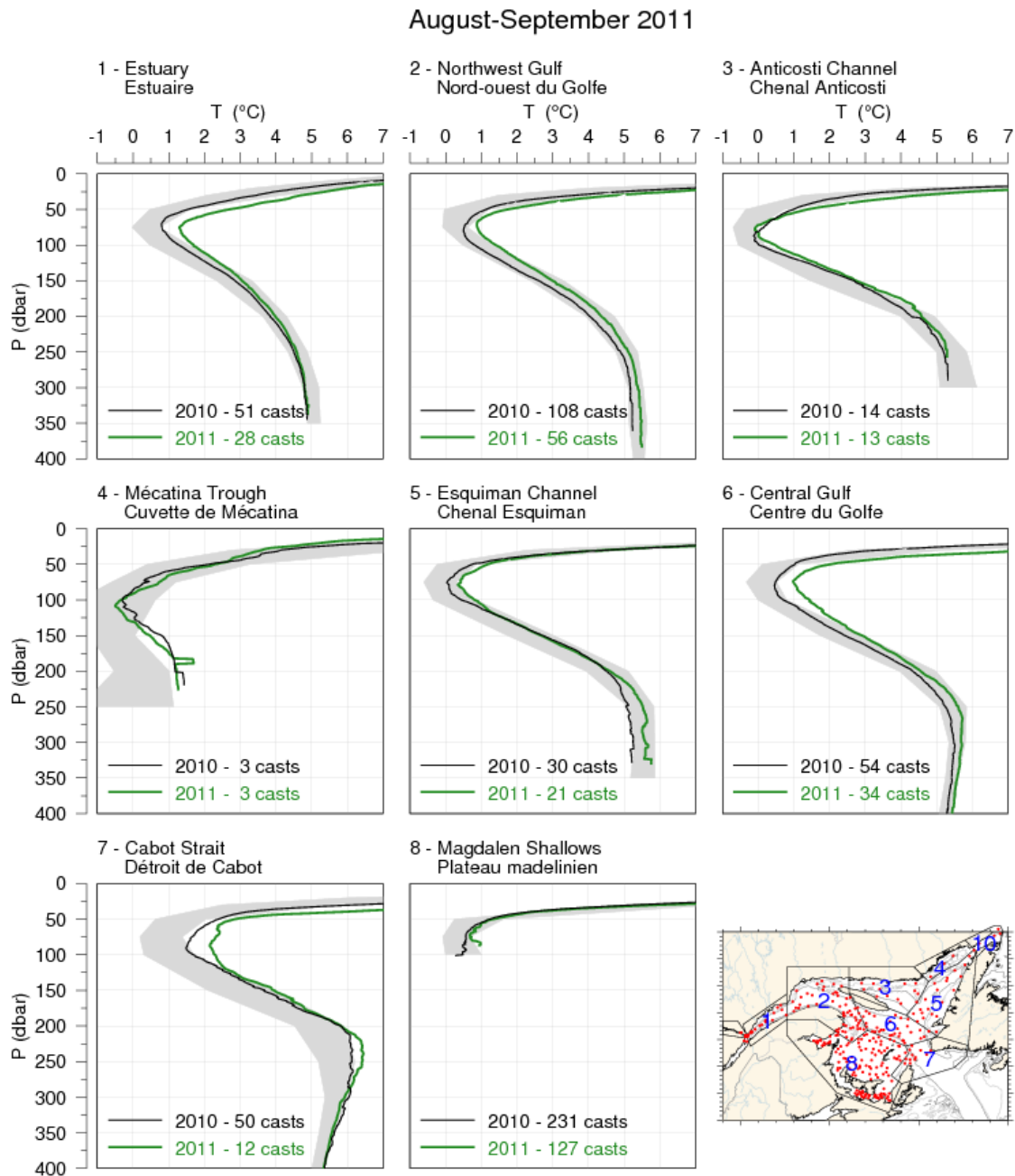
Fig. 39. Mean temperature profiles observed in each region of the Gulf during August and September. The shaded area represents the 1981–2010 climatological monthly mean \pm 1 SD for August for regions 1 through 7 and for September for region 8. Mean profiles for the 2010 survey are also shown for comparison.
