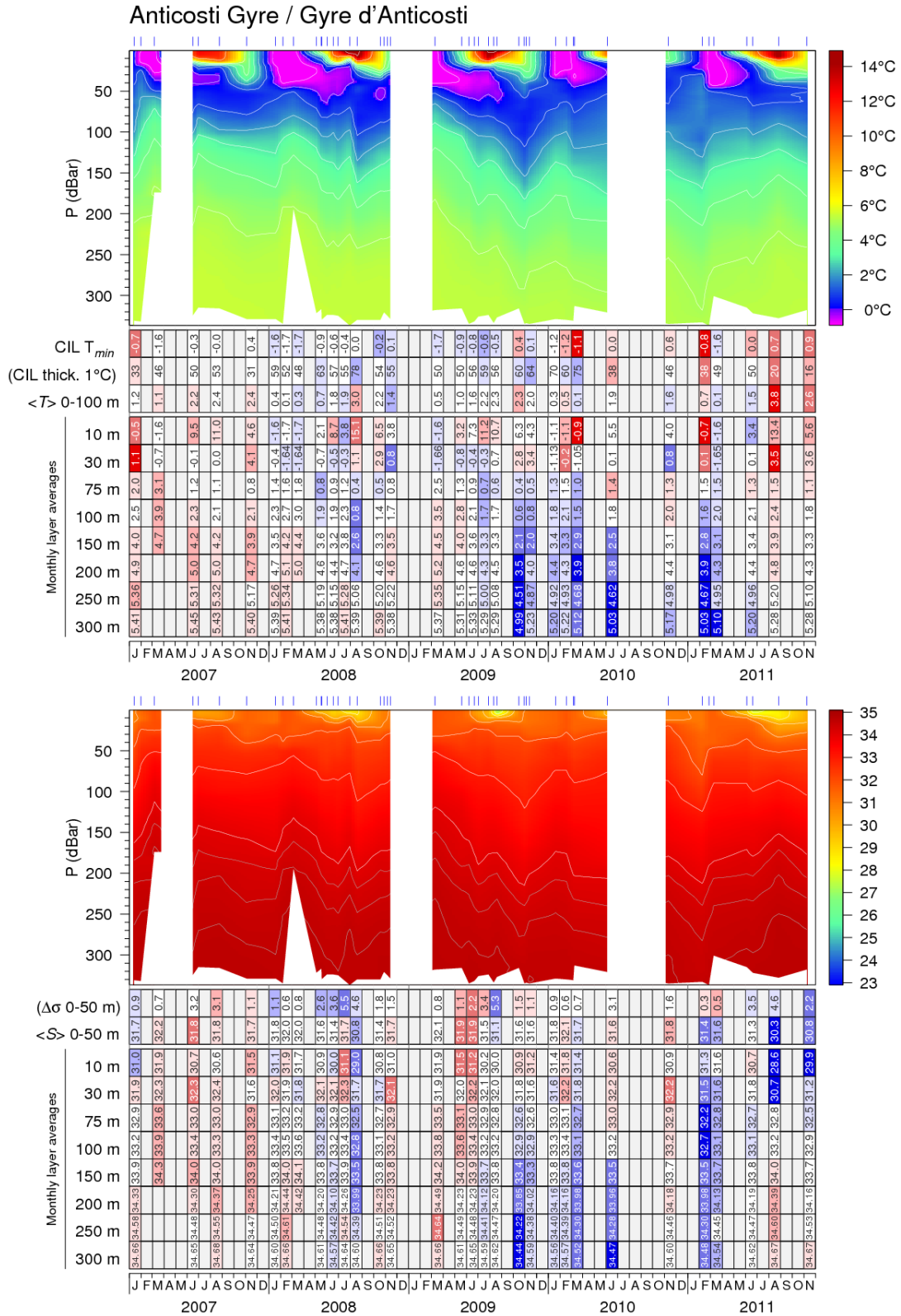
Fig. 49. Isotherm (top) and isohaline (bottom) time series at the Anticosti Gyre station; tick marks above indicate sample dates. Scorecard tables are monthly layer averages colour-coded according to the anomaly relative to the 1996–2010 monthly climatology for the station (yearly climatology for 250 m and deeper).
