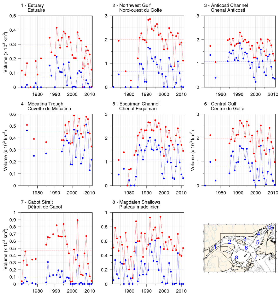
Fig. 28. Volume of the CIL colder than 0^\circ\text{C} (blue) and colder than 1^\circ\text{C} (red) in August and September (primarily region 8 in September). The volume of the CIL colder than 1^\circ\text{C} in November 2006 to 2009 and 2011 is also shown for the St. Lawrence Estuary (dashed line).
