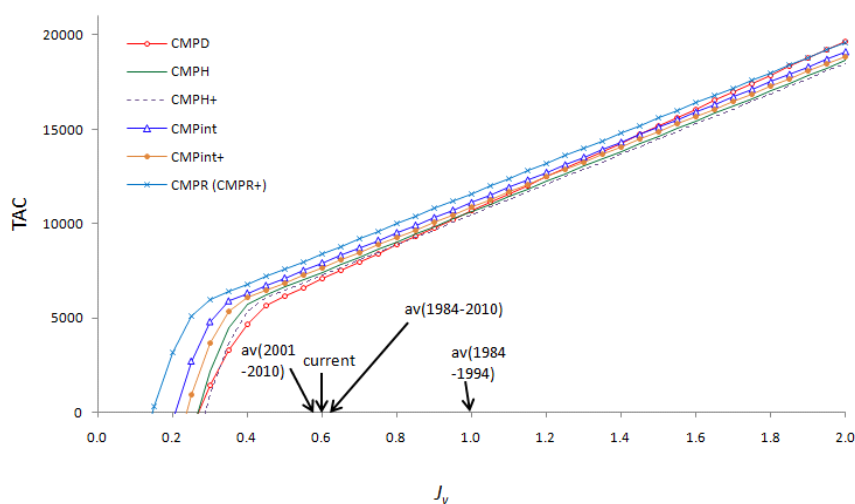
Figure 1: Relationship between the catch limit output by the seven CMPs and the RV Survey Index Ratio. The arrows indicate values of this ratio at other times or averaged over the periods indicated. Note CMPInt+ was selected as the Pollock MP.
