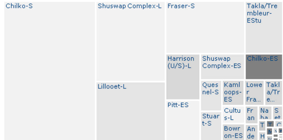
Figure 13: Treemap of status evaluations for 36 conservation units of Fraser sockeye
