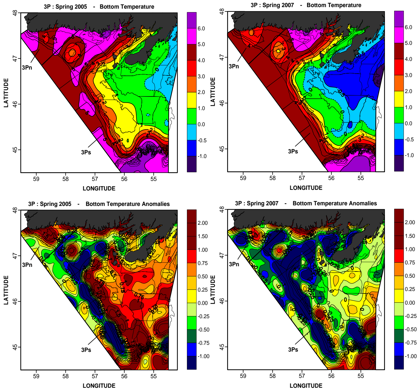
Figure 3. The April 2005 and 2007 bottom temperature and anomalies (in °C) in NAFO Subdivisions 3Pn and 3Ps. The anomalies are referenced to the 1971-2000 average.
