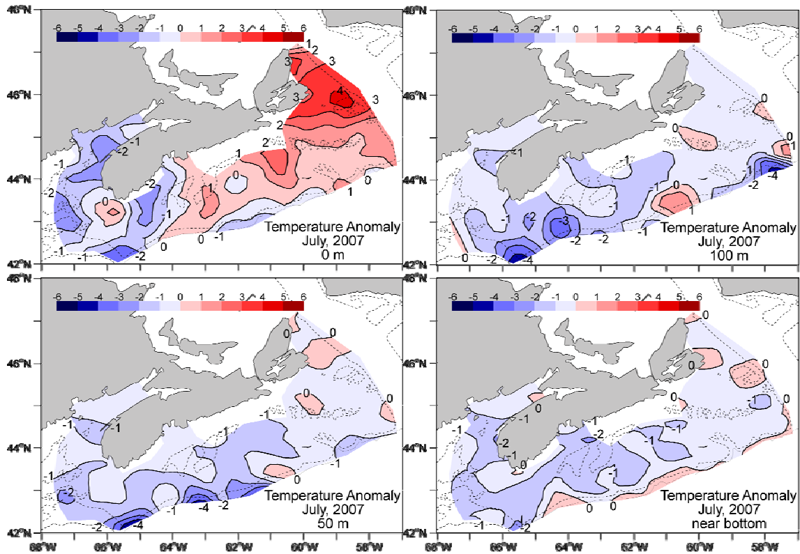
Figure 7. Plan views of the temperature anomalies at 0, 50, 100m and near the bottom for the Scotian Shelf in July 2007. The anomalies are based on observations collected during the annual groundfish survey.
