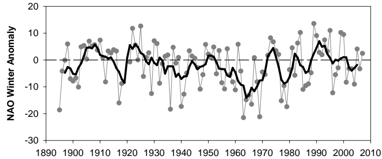
Figure 2. North Atlantic Oscillation winter anomaly relative to the 1971-2000 means. The annual anomaly (grey line with dots) and 5 year running means (black line) are shown.
