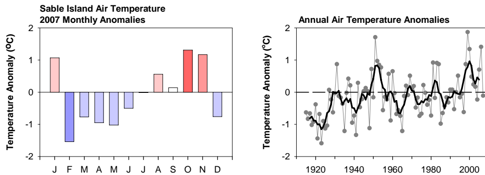
Figure 3. Sable Island monthly air temperature anomalies for 2007 relative to the 1971-2000 means (left panel). The colour of the bars represents the number of standard deviations the anomaly differs from the mean (see Figure 12). Time series of annual air temperature anomalies (grey line and dots) and 5 year running means (heavy, black line; right panel).
