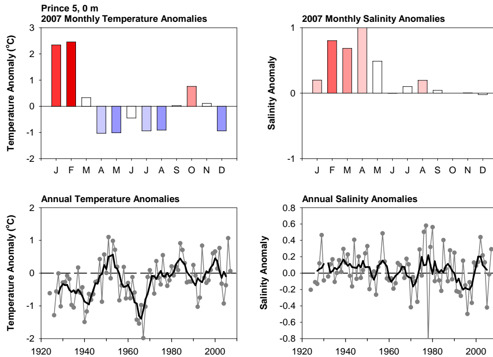
Figure 5. Monthly surface temperature anomalies for 2007 relative to the 1971-2000 means for the Prince 5 station at the mouth of the Bay of Fundy (top left panel). The colour of the bars represents the number of standard deviations the anomaly differs from the mean (see Figure 12). Time series of annual surface temperature anomalies (grey line and dots, lower left panel) and 5 year running means (heavy, black line; lower left panel). Monthly surface salinity anomalies for 2007 (top right panel) and the time series of annual surface salinity anomalies (grey line and dots, lower left panel) and 5 year running means (heavy, black line; lower right panel).
