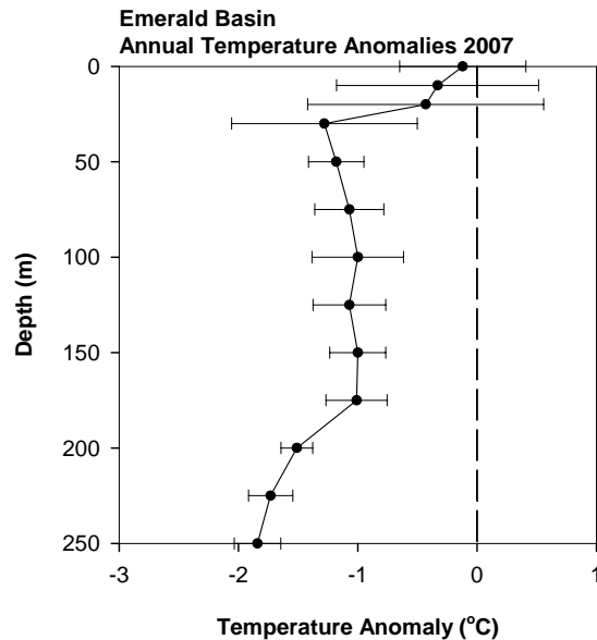
Figure 6. Depth profile of the annual temperature anomalies (dots) based on averages of the monthly anomalies for Emerald Basin in 2007. Horizontal bars are estimates of the standard error.
