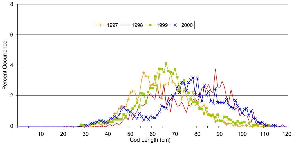
Figure 5a Length Composition of Cod (3Ps Stratified Random Surveys 1997-2000)
