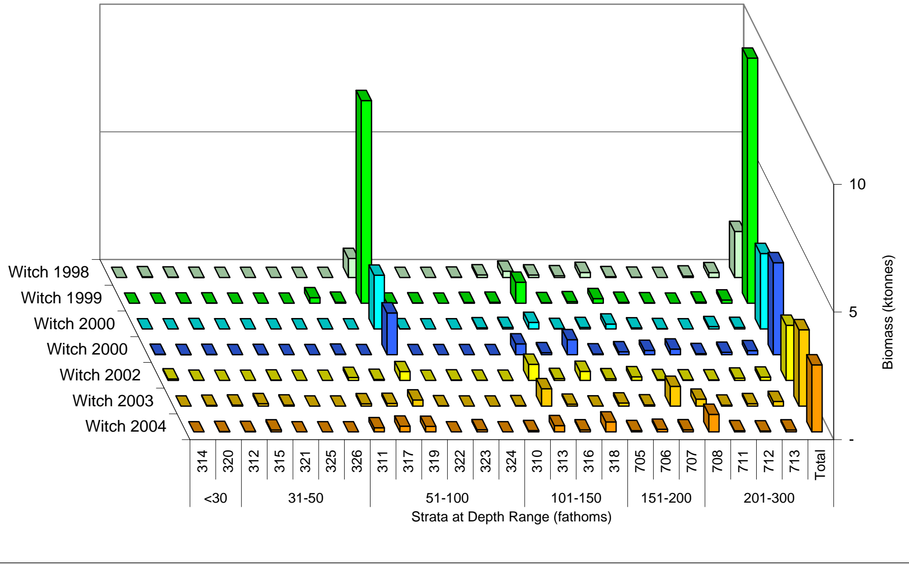
Figure 27 Witch, 3Ps, 1998-2004, Estimated Biomass
