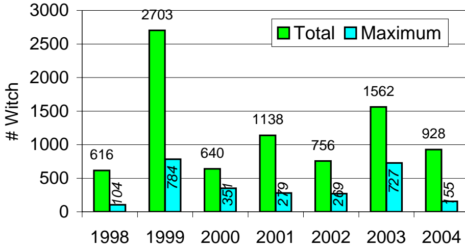
Figure 21a GEAC Fall 3Ps Surveys
