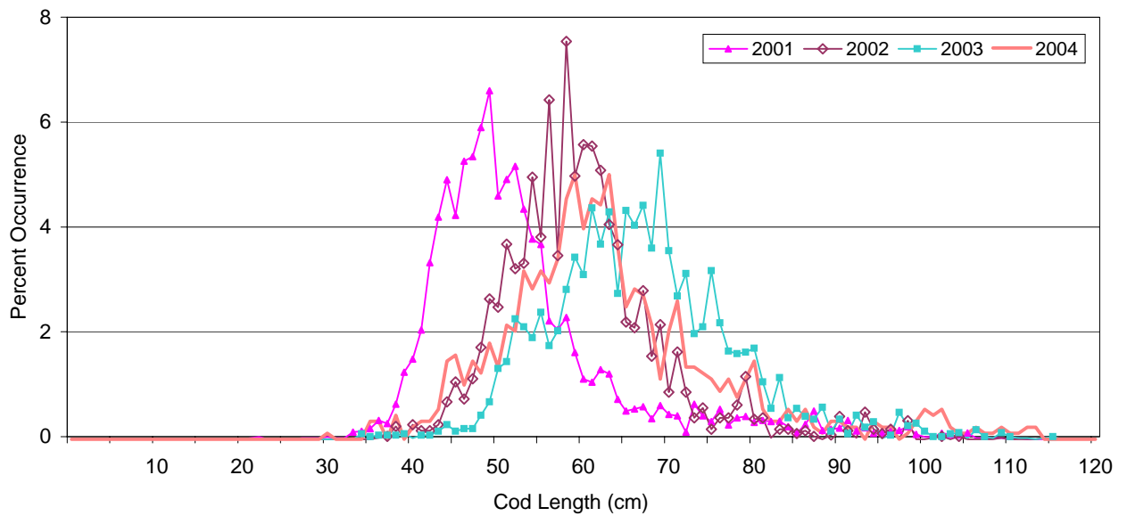
Figure 5b Length Composition of Cod (3Ps Stratified Random Surveys 2001-2004)
