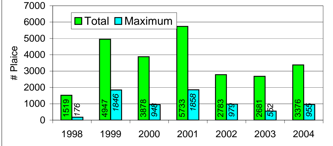
Figure 13a GEAC Fall 3Ps Surveys
