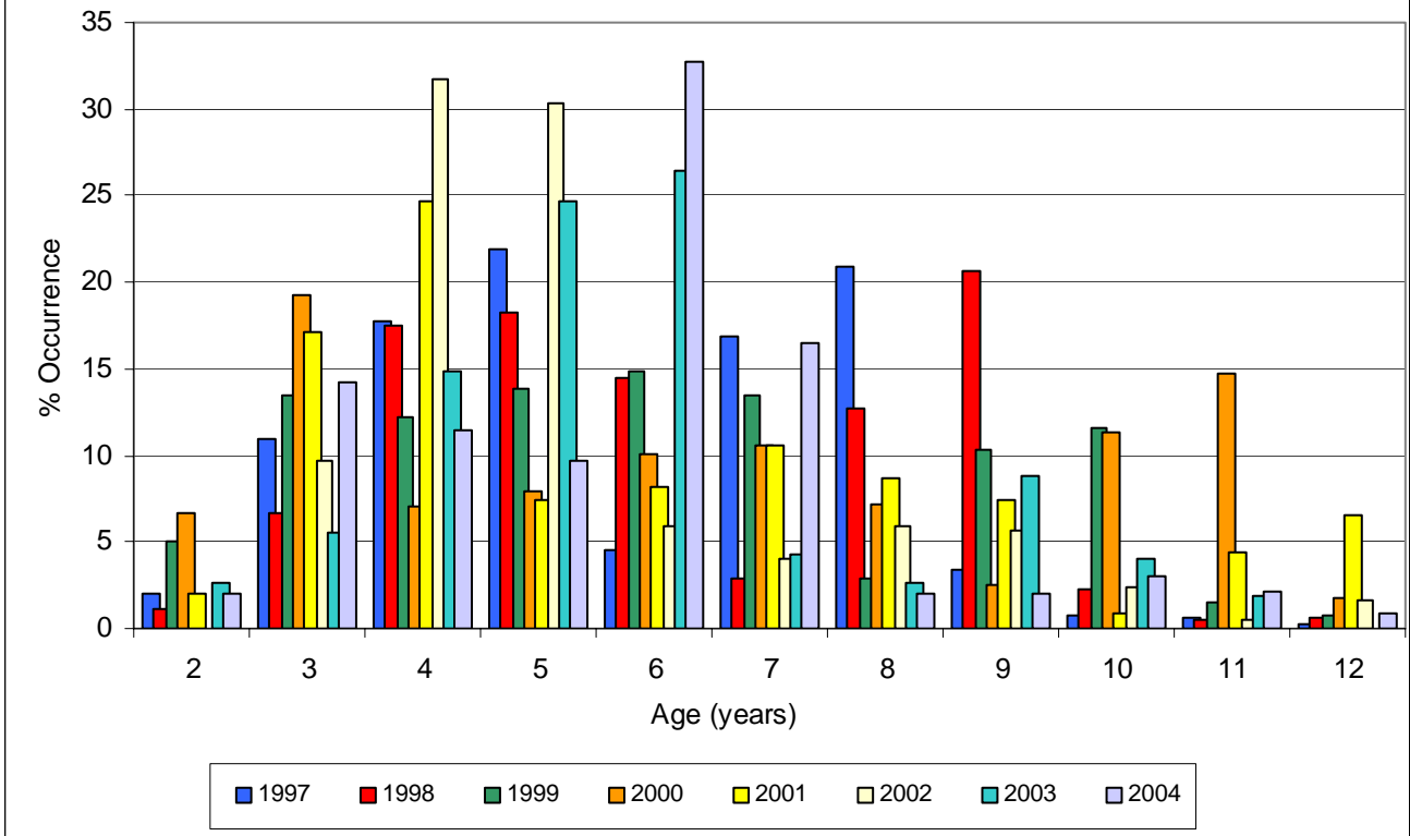
Figure 6d Age Composition of 3Ps Sampled Cod
