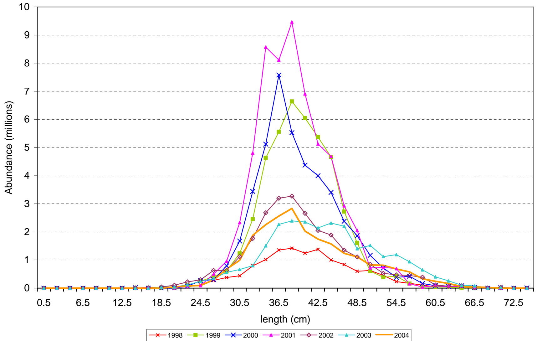
Figure 17 Plaice Survey Abundance index at length, 3Ps, 1998-2004
