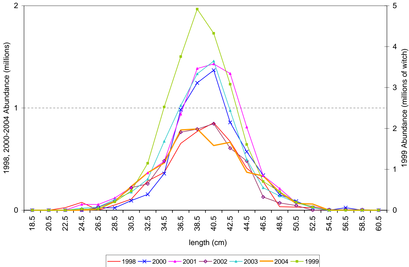
Figure 25 Witch Survey Abundance index at length, 3Ps, 1998-2004
