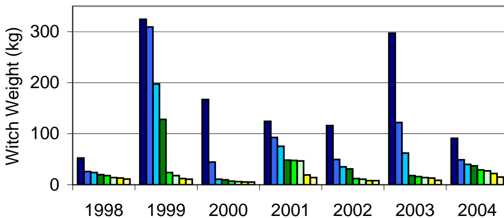
Figure 21c GEAC Fall 3Ps Surveys: Largest Sets
