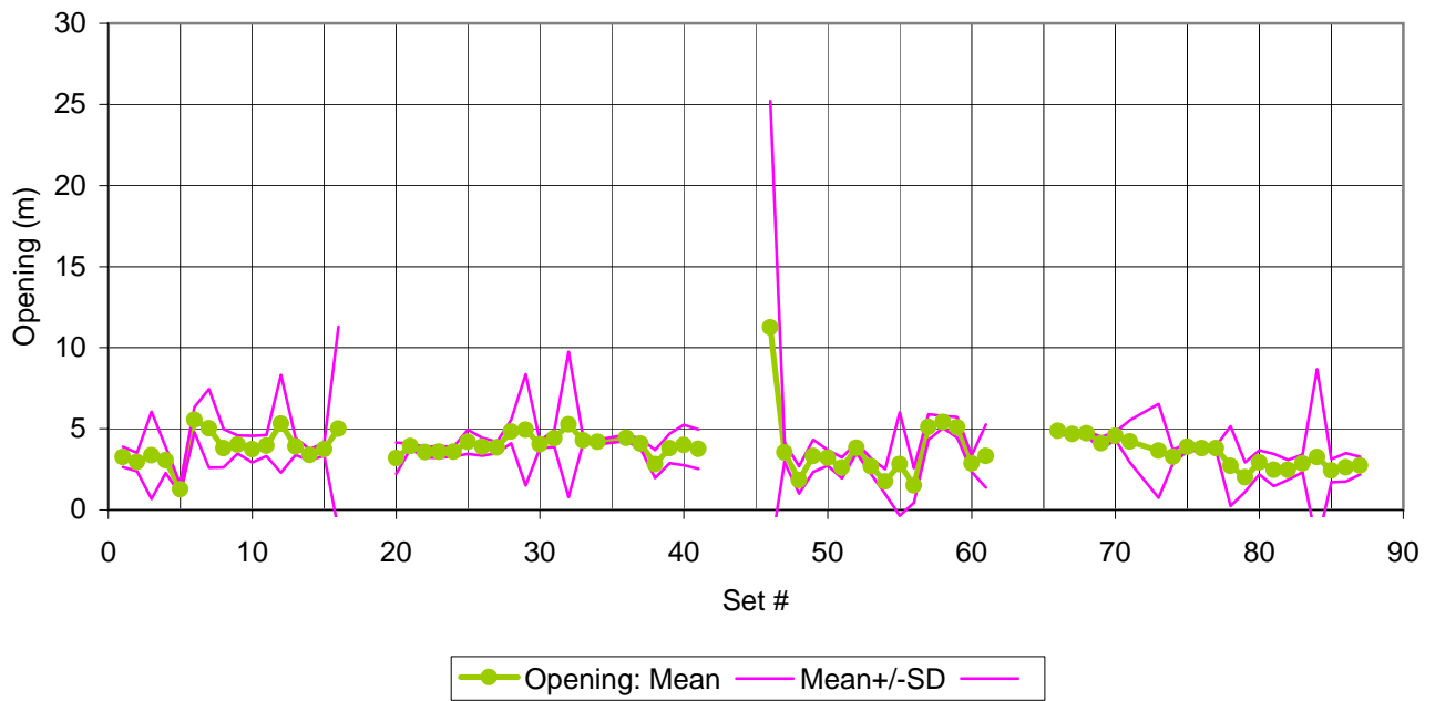
Figure 2b 2004 3Ps Survey Net Opening
