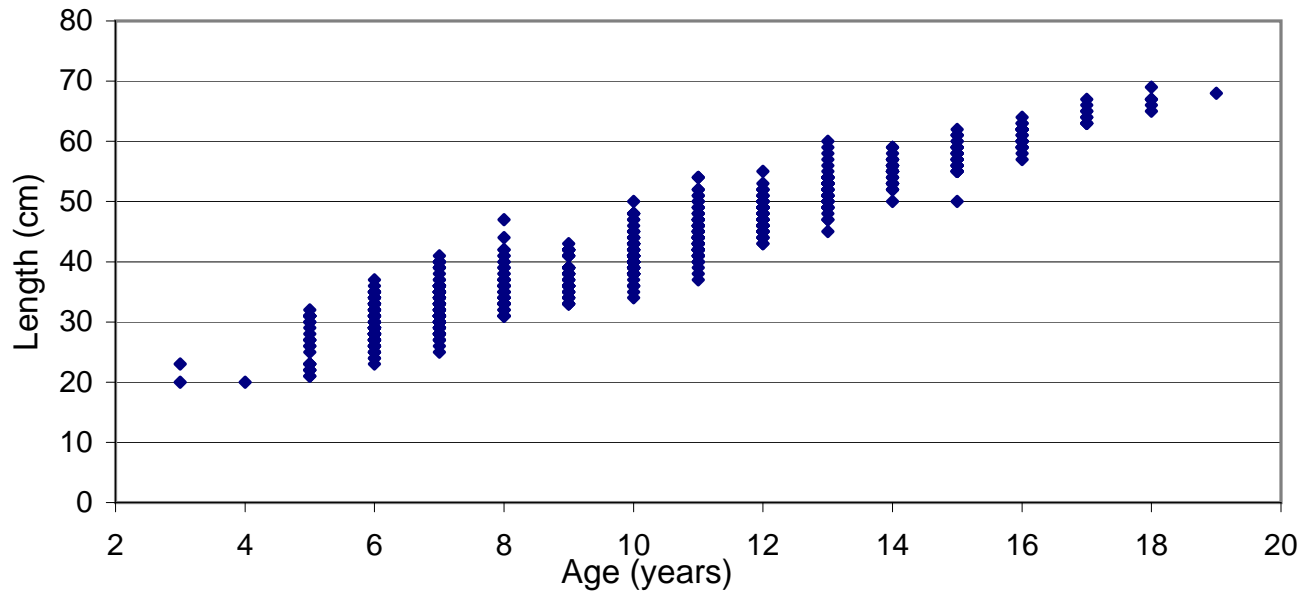
Figure 15a Plaice Age-Length Composition 3Ps 2004 (751 samples)
