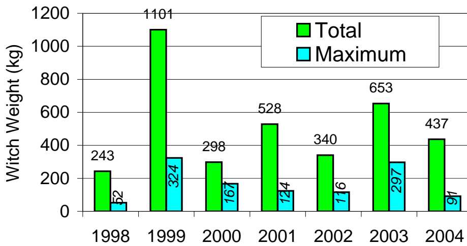
Figure 21b GEAC Fall 3Ps Surveys
