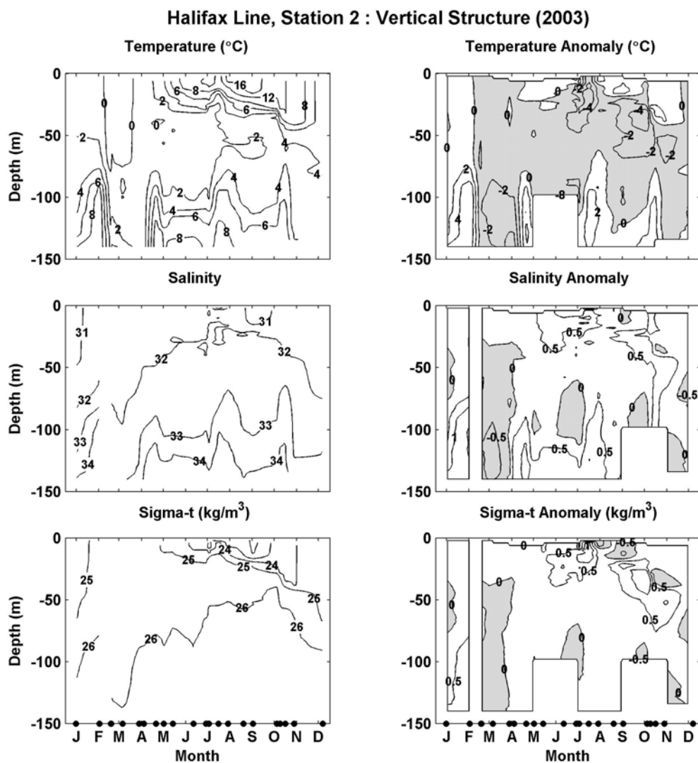
Fig. 6. Contours of the 2003 temperature, salinity and density (sigma-t) (left) and their anomalies (right) at the standard station H2. Negative anomalies are shaded.
