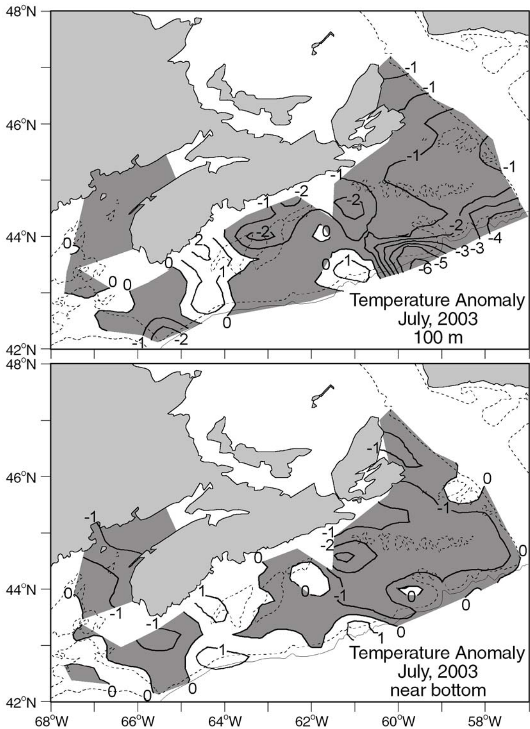
Fig.12b. Contours of temperature anomalies at 100 m (top panel) and near bottom (bottom panel) during the 2003 July groundfish and ITQ surveys.
