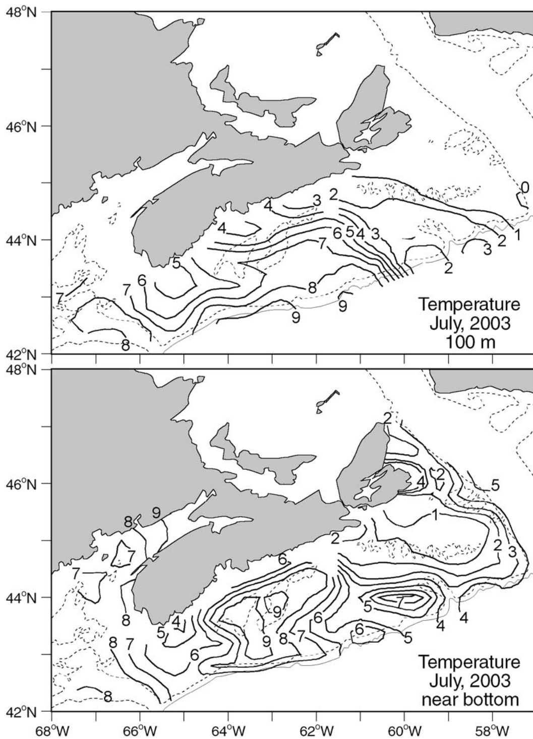
Fig. 11b. Contours of temperatures at 100 m (top panel) and near bottom (bottom panel) during the 2003 July groundfish and ITQ surveys.
