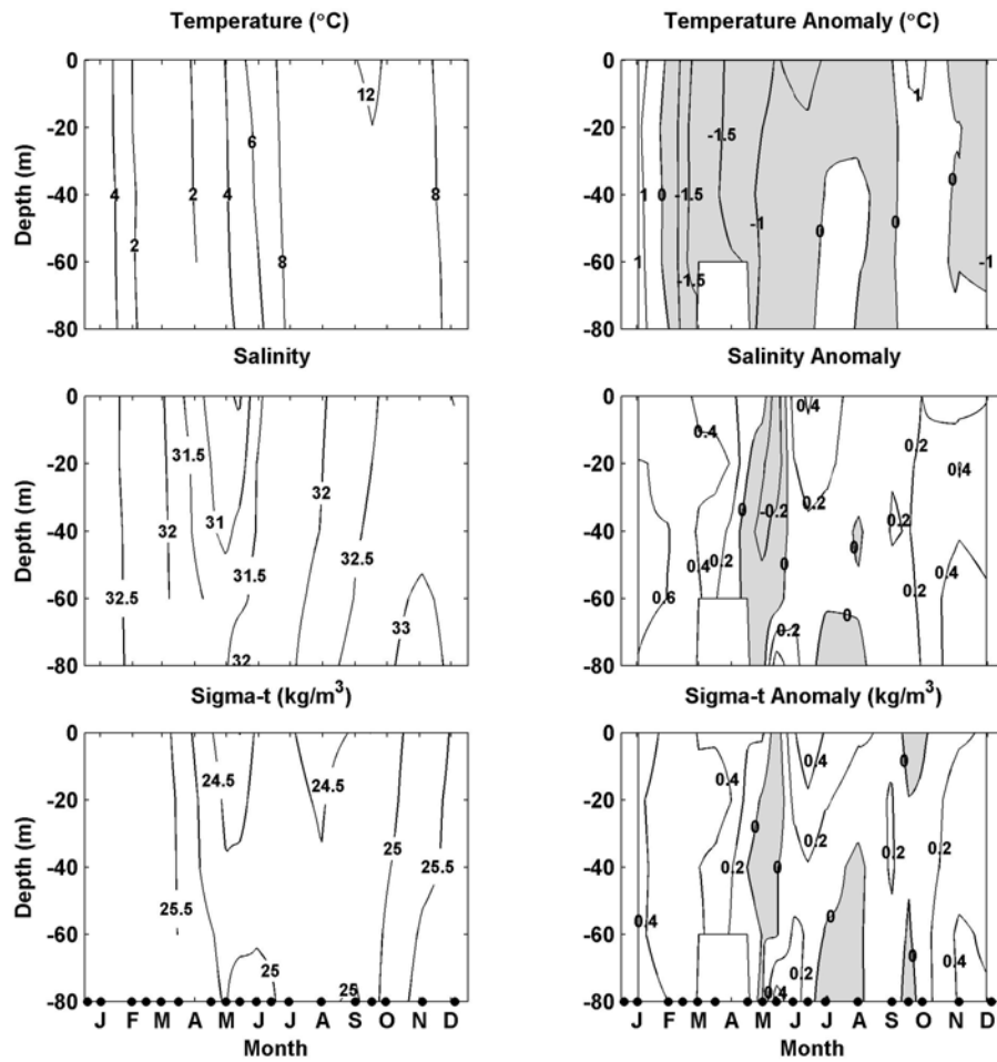
Fig. 3. Contours of temperature, salinity and sigma-t and their anomalies at Prince 5 as a function of depth during 2003 relative to the 1971-2000 means. Colder and fresher-than-normal conditions are shaded.
