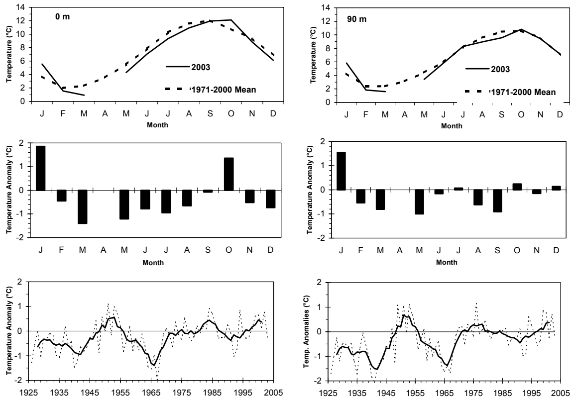
Fig. 4. The monthly mean temperatures for 2003 (solid line; top panels) and their long-term means (dashed line; top panels), the monthly anomalies relative to the long-term means for 1971-2000 (middle panels) and in the bottom panels are the time series of the annual means (dashed lines) and their 5-year running means (solid line) for Prince 5, 0 m (left) and 90 m (right).
