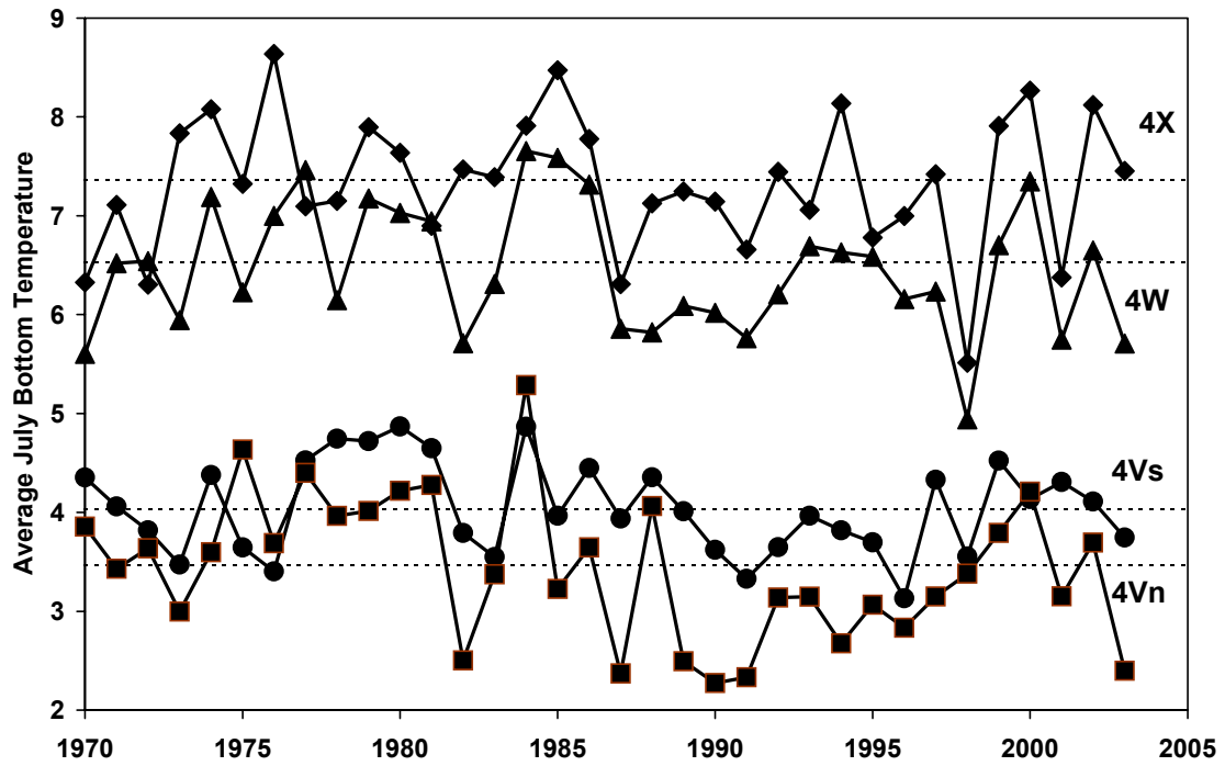
Fig. 14. Time series of annual mean bottom temperatures from areas 4Vn, 4Vs, 4W and 4X. The horizontal lines are the 1971-2000 means.
