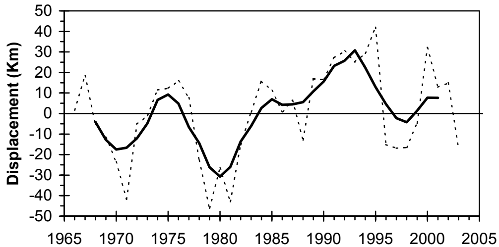
Gulf Stream Annual Anomalies 56°W-75°W
