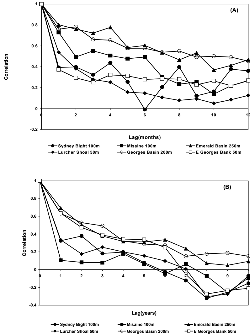
Fig. 10. Autocorrelations of the temperature series of Fig. 9 for the (A) monthly and (B) annual anomalies.
