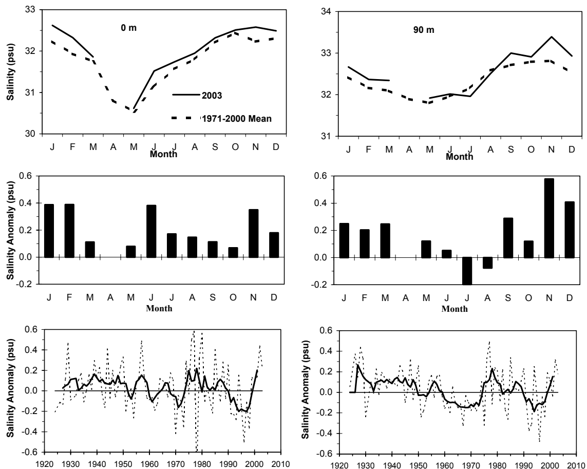
Fig. 5. The monthly mean salinities for 2003 (solid line; top panels) and their long-term means (dashed line; top panels), the monthly anomalies relative to the long-term means for 1971-2000 (middle panels) and in the bottom panels are the time series of the annual means (dashed lines) and their 5-year running averages (solid line) for Prince 5, 0 m (left) and 90 m (right).
