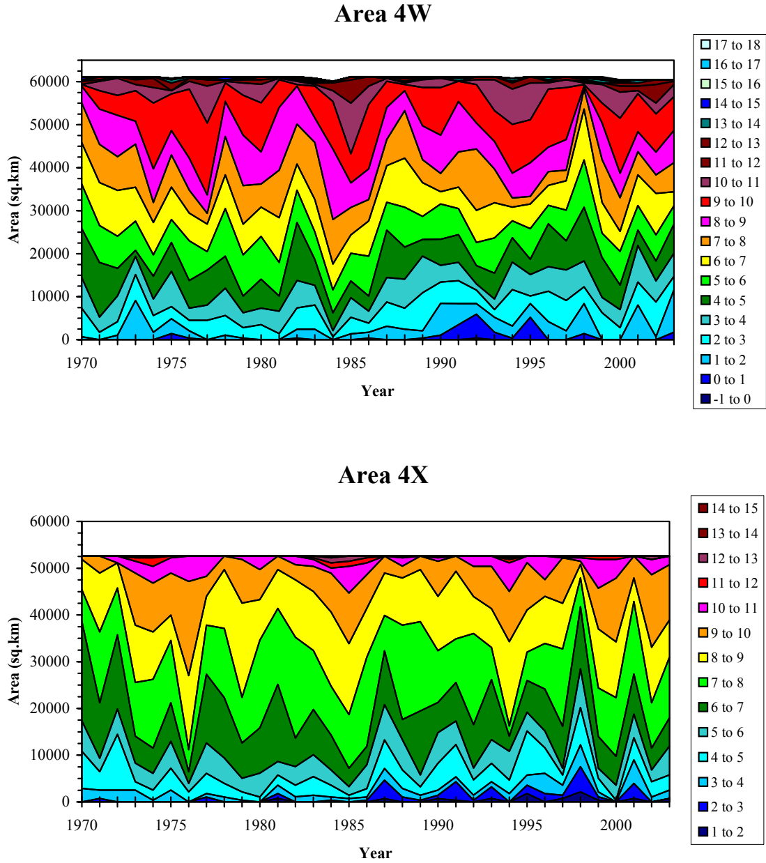
Fig. 13b. The time series of the area of the bottom for each 1°C temperature range for NAFO Subareas 4W (top panel) and 4X(bottom panel).
