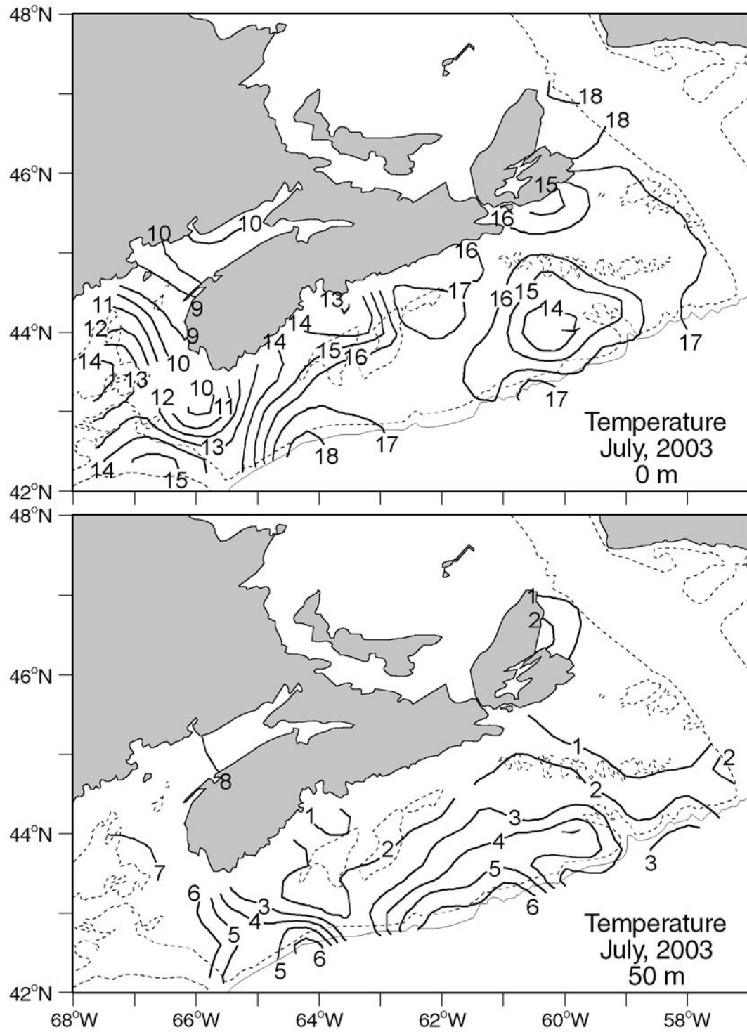
Fig.11a. Contours of temperatures at the surface (top panel) and 50 m (bottom panel) during the 2003 July groundfish and ITQ surveys.
