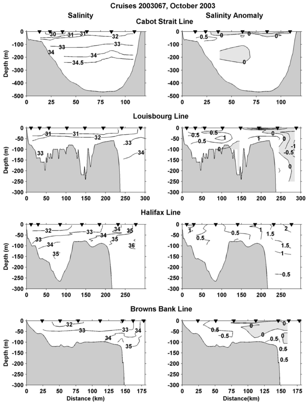
Fig.15e. Salinity and salinity anomalies for standard Scotian Shelf sections, October 2003.
