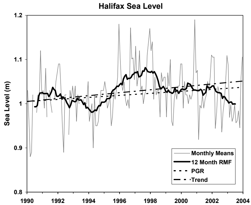
Fig. 20. The time series of the monthly means and a 12 month running mean of the sea level elevations at Halifax, along with the observed linear trend and that predicted by a model from post-glacial rebound.
