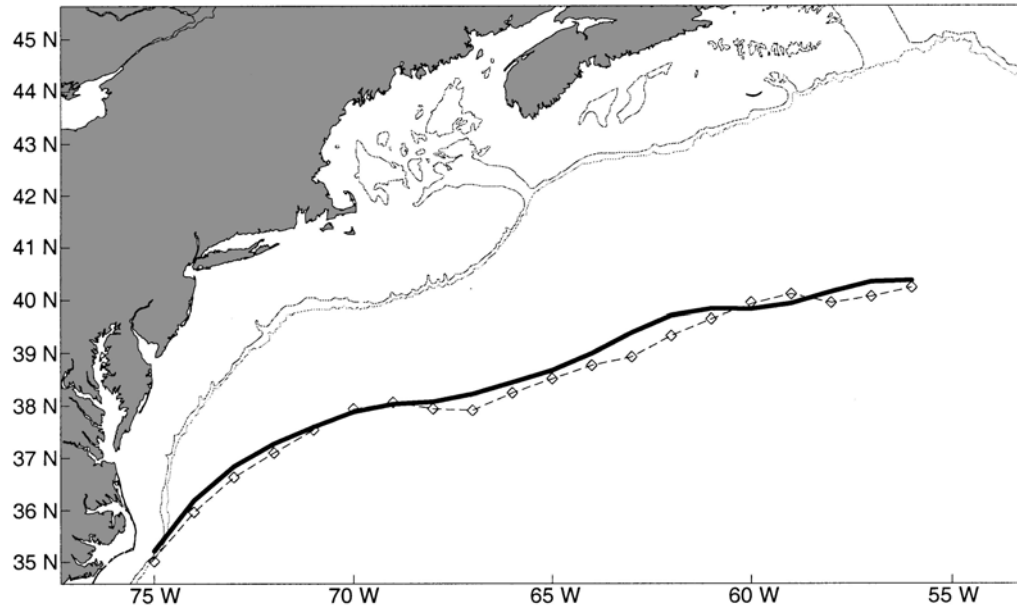
Gulf Stream Annual Anomalies 56°W-75°W
