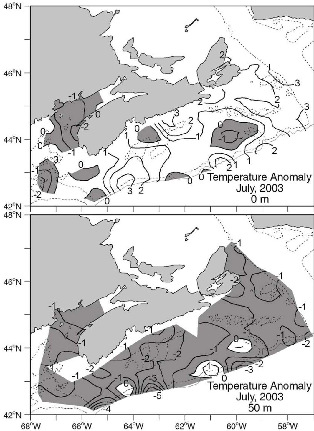
Fig.12a. Contours of temperature anomalies at the surface (top panel) and 50 m (bottom panel) during the 2003 July groundfish and ITQ surveys.
