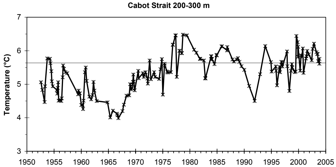
Fig. 16. Average temperature over the 200-300 m layer in Cabot Strait. The horizontal line indicates the 1971-2000 mean.
