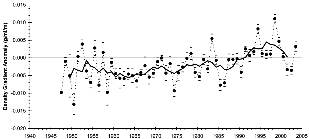
Fig. 19. The mean annual (dashed line) and 5-yr running mean (heavy solid line) of the stratification index (0-50 m density gradient) averaged over the Scotian Shelf (areas 4-23 inclusive). The short horizontal lines for each year represent the standard errors of the different areas.
