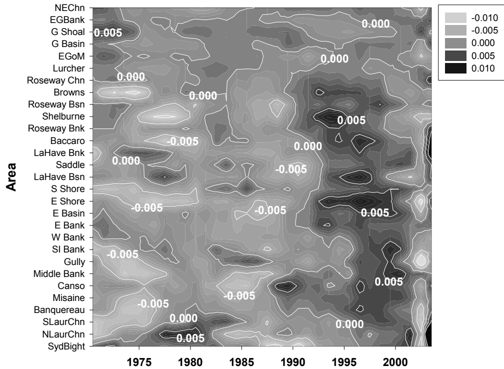
Fig. 18. The contoured density anomaly for 1970-2003. The anomalies for 1970-2001 are the 5 y running mean values; the annual values are shown for 2002-03.
