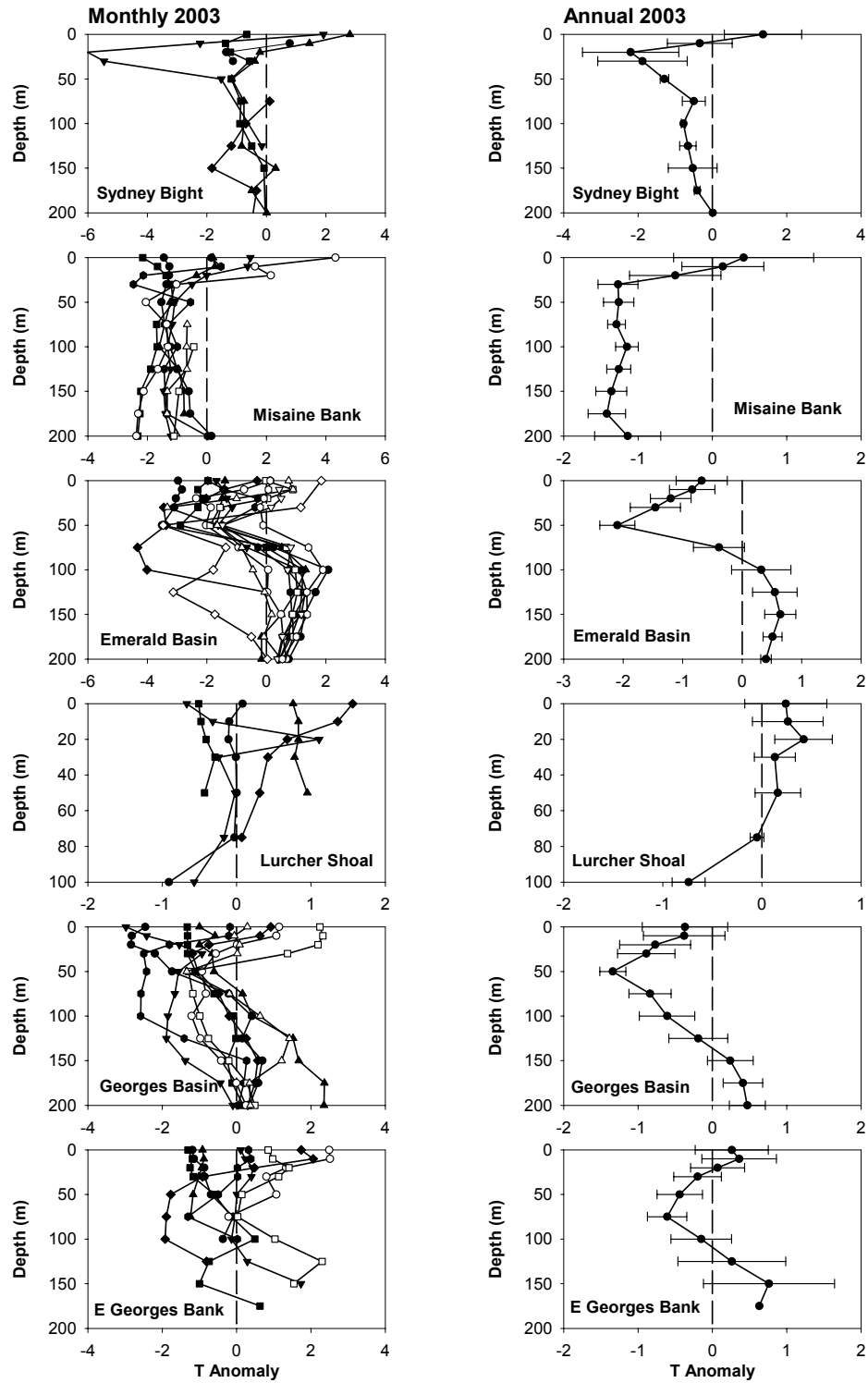
Fig. 8. Monthly (left) and annual ( \pm std. error, right) temperature anomaly profiles for selected locations. Symbol order is filled dot, square, up triangle, down triangle, diamond, hexagon, then open symbols in the same order.
