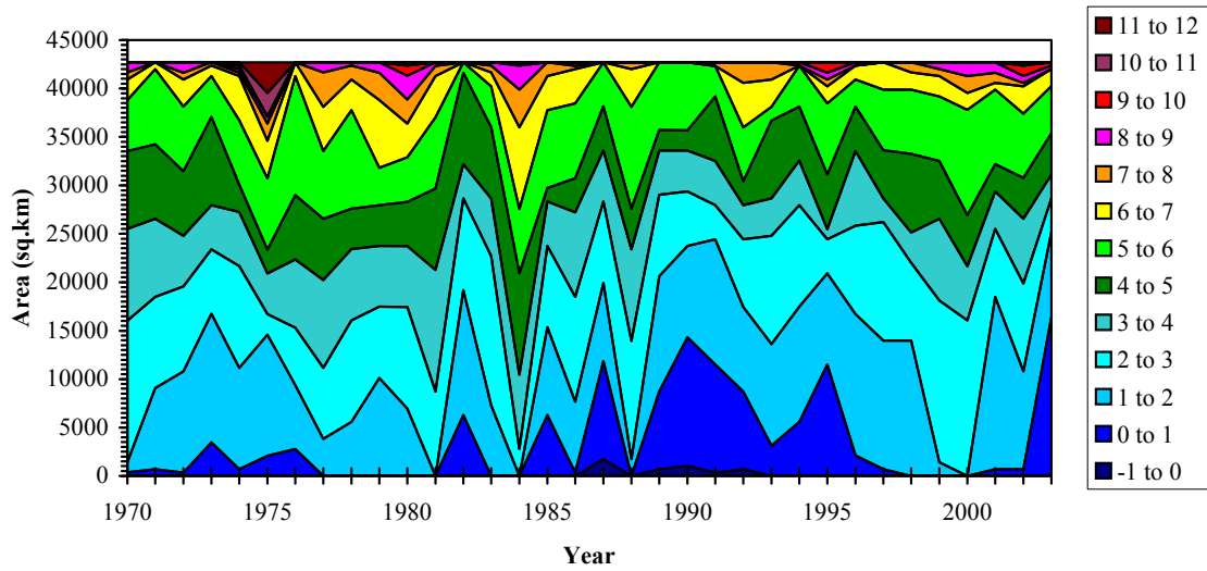
Fig.13a. The time series of the area of the bottom for each 1°C temperature range for NAFO Subareas 4Vn (top panel) and 4Vs(bottom panel).
