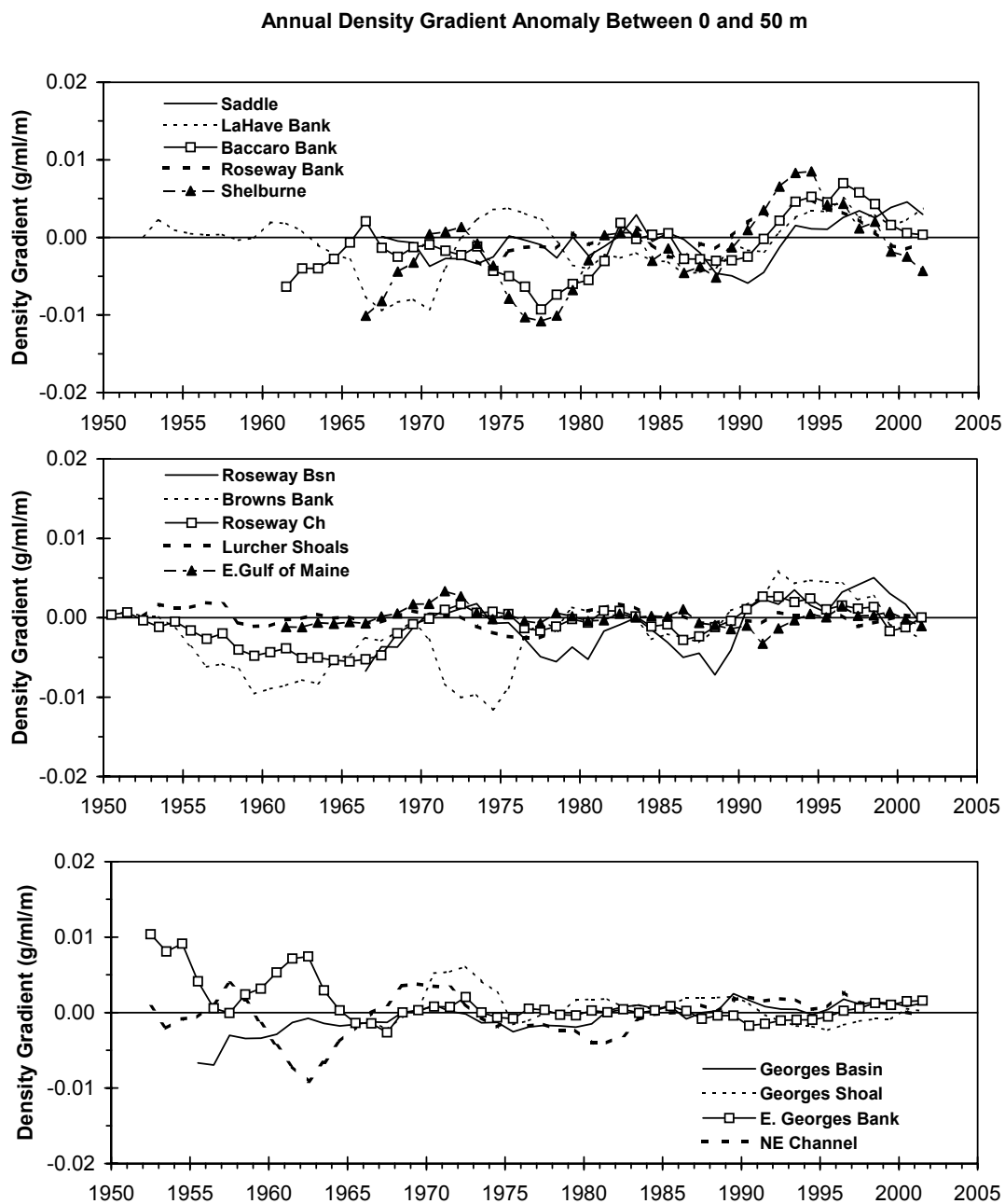
Fig.17b. Five-year running means annual density gradient anomalies between the surface and 50 m calculated for the areas 16-29 in Fig. 7.
