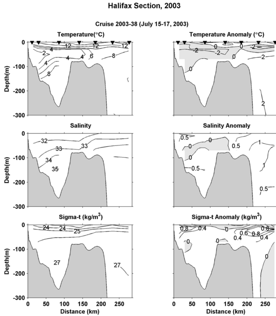
Fig.15c. Temperature, salinity, density and their anomalies for the Halifax section, July 2003.
