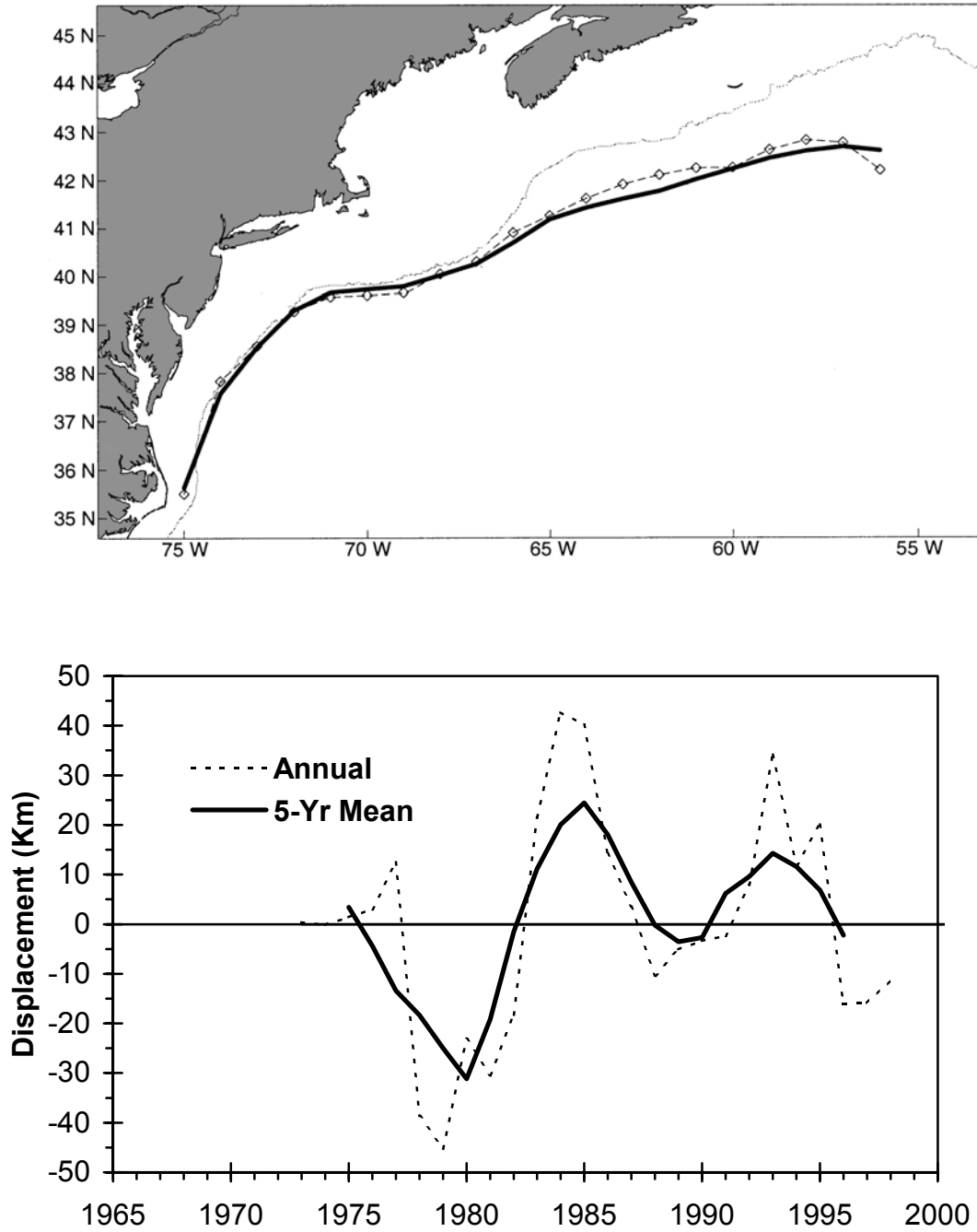
Fig. 21. The 2003 (dashed line) and long-term mean (1973-2000; solid line) positions of the shelf/slope front (top panel) and the time series of the annual anomaly of the mean (56°-75°W) position of the shelf/slope front (bottom panel).
