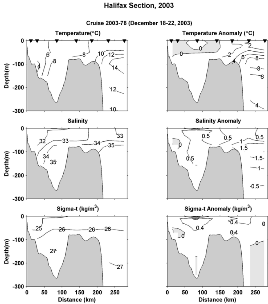
Fig.15g. Temperature, salinity, density and their anomalies for the Halifax section, December 2003.
