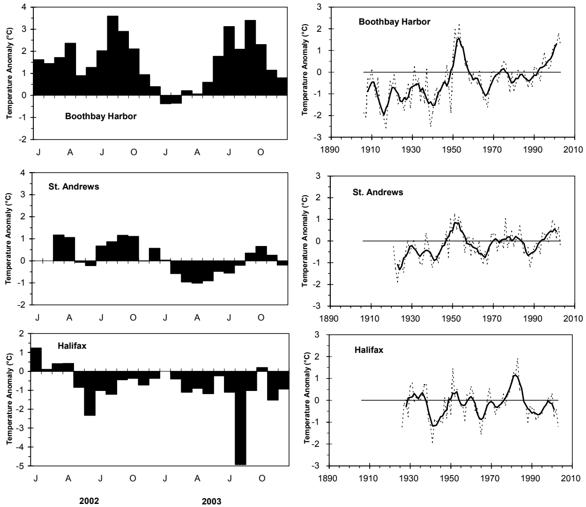
Fig. 2. The monthly sea surface temperature anomalies during 2002 and 2003 (left) and the annual temperature anomalies and their 5-year running means (right) for Boothbay Harbor, St. Andrews and Halifax Harbour. Anomalies are relative to the 1971-2000 means.
