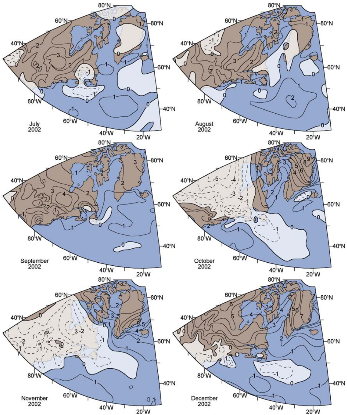
Fig. 2C. Monthly air temperature anomalies ( ^{\circ}\text{C} ) over the Northwest Atlantic from July to December of 2002 relative to their 1961-1990 means. The white shaded areas are colder-than-normal. (Redrawn from Grosswetterlagen Europas )
