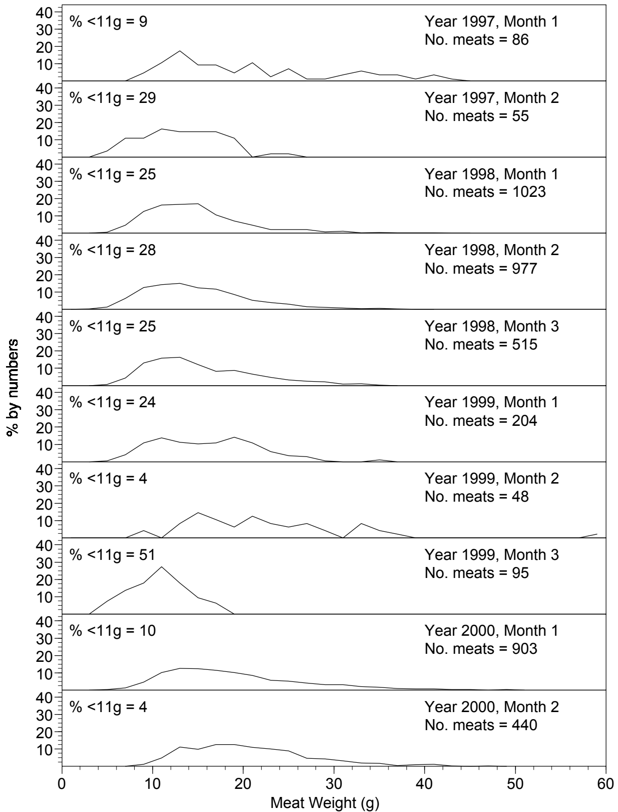
Figure 13a. Meat weight distribution for port samples from vessels fishing in SPA 6B by month. Vertical line at 11 grams is the meat weight equivalent to a meat count of 45/500g.
