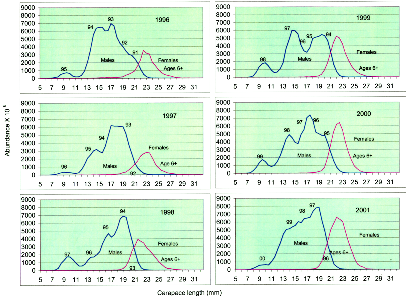
Fig. 9 Abundance at length for Hawke Channel + 3K (SFA 6) estimated from OGIVE MAPping (OGMAP) of research survey data, 1996 – 2001.
