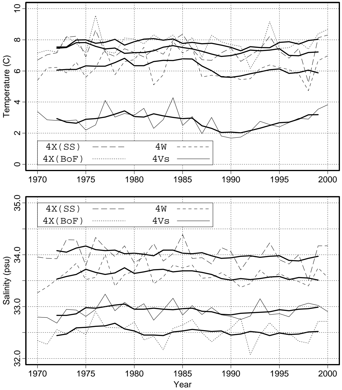
Figure 17: Time series of stratified mean near-bottom temperatures and salinities for summer 4VWX surveys. Bold line is a 5 year running mean.
