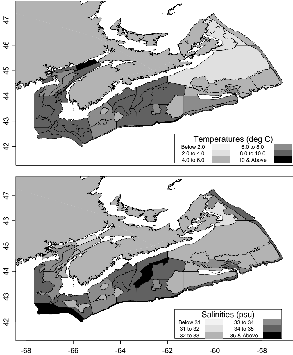
Figure 12: Map of near-bottom strata mean temperatures and salinities during the summer of 2000.
