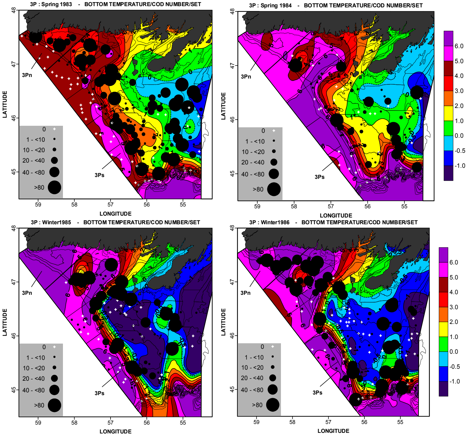
Fig. 2a. Bottom temperature contour maps (in °C) for 1983-1986 based on all data collected during the winter and spring time periods. The numbers of cod in each fishing set from the annual 3Pn and 3Ps surveys are shown as solid circles. The crosses represent zero catches.
