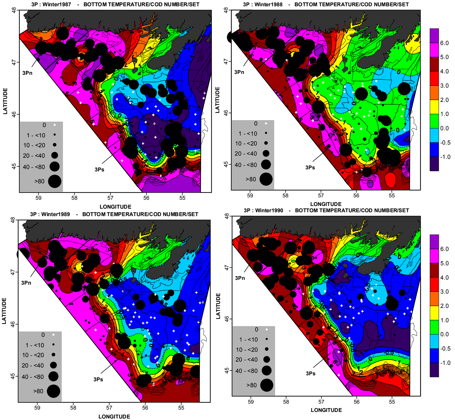
Fig. 2b. Bottom temperature contour maps (in °C) for 1987-1990 based on all data collected during the winter and spring time periods. The numbers of cod in each fishing set from the annual 3Pn and 3Ps surveys are shown as solid circles. The crosses represent zero catches.
