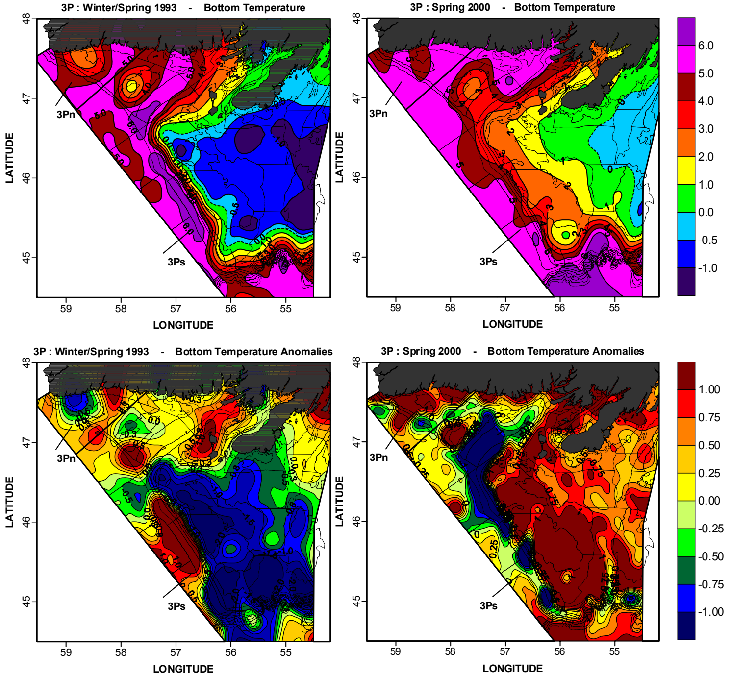
Fig. 1 Contour maps of bottom temperature and anomalies (in °C) for 1993 and 2000 in NAFO Subdivisions 3Pn and 3Ps. The anomalies are referenced to all available data collected in the area from 1971-2000.
