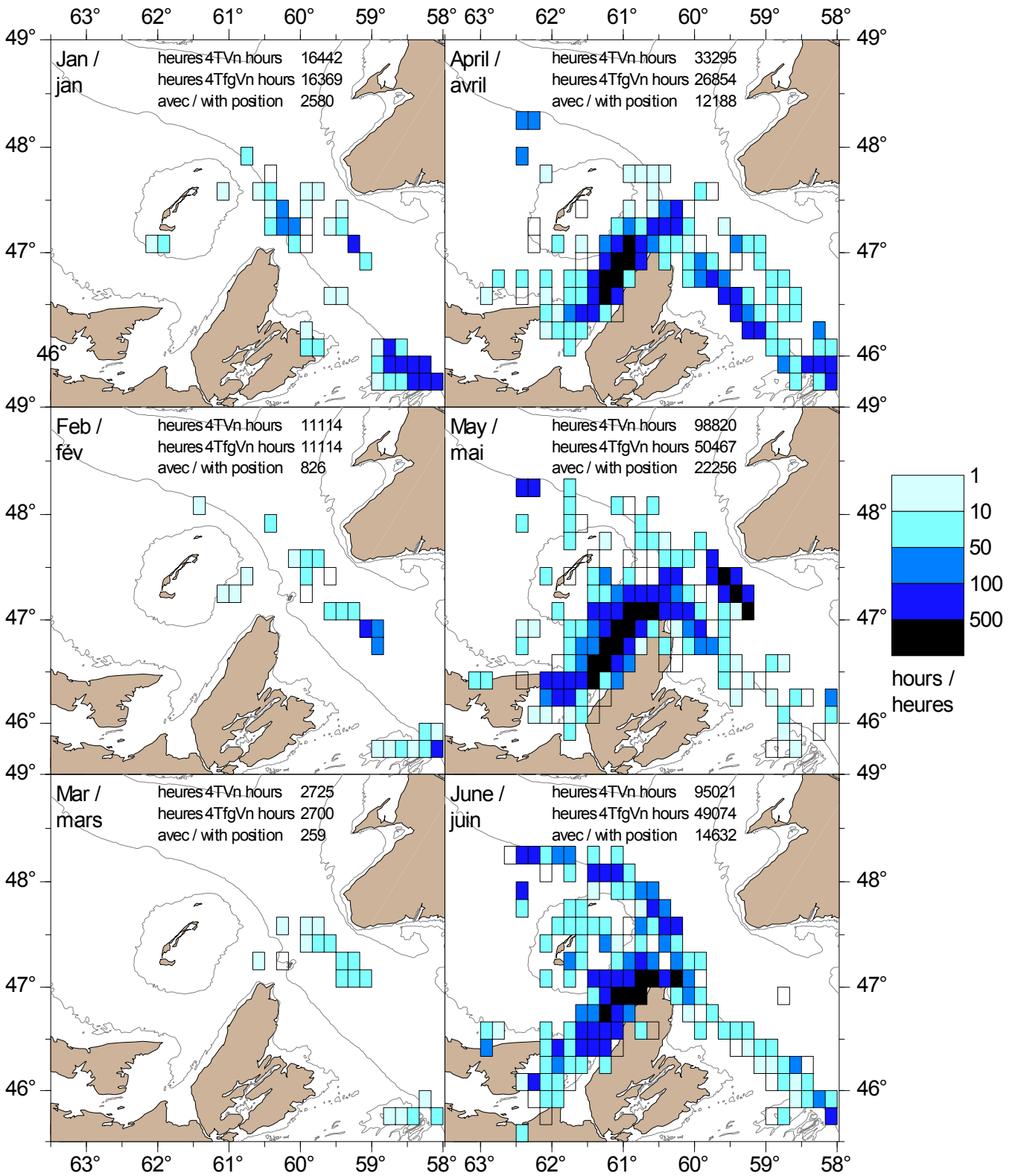
Figure 2. Groundfish mobile gear effort in the southern Gulf of St. Lawrence (1986 to 1990)
