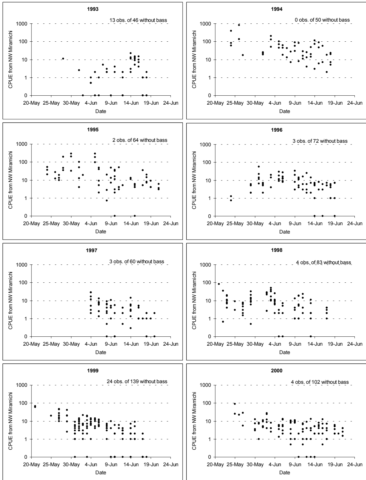
Figure 7. Catch per unit of effort of adult striped bass (bass per trapnet per 24-hr. period) in the commercial gaspereau fishery of the NW Miramichi River for years 1993 to 2000. Individual points may represent several observations.
