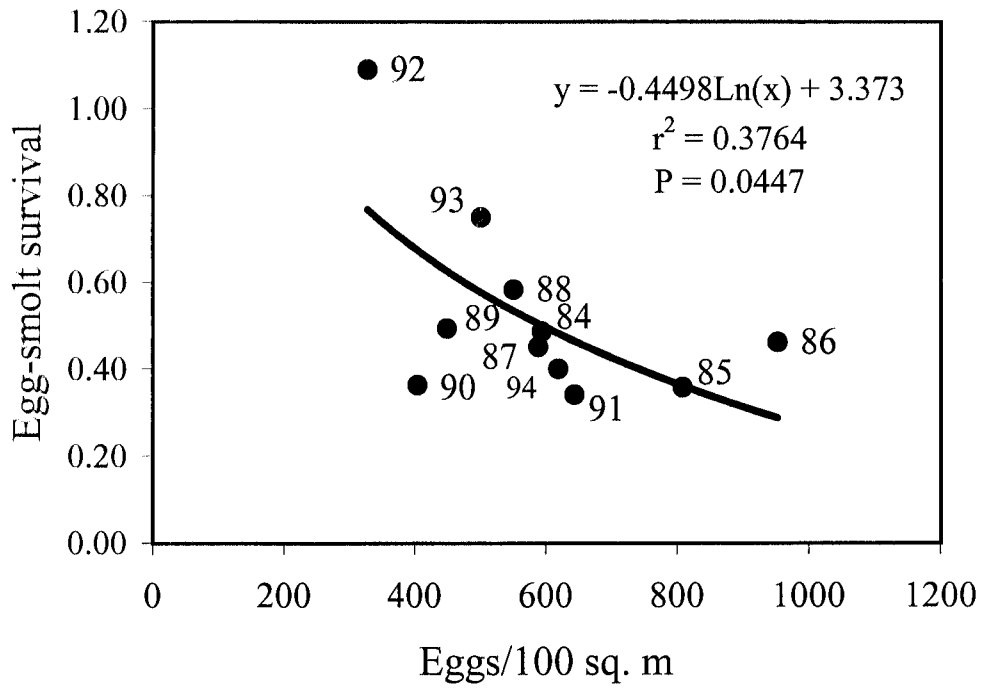
Fig. 32. Relationship between egg-to-smolt survival and egg deposition for Northeast Brook, Trepassey.
