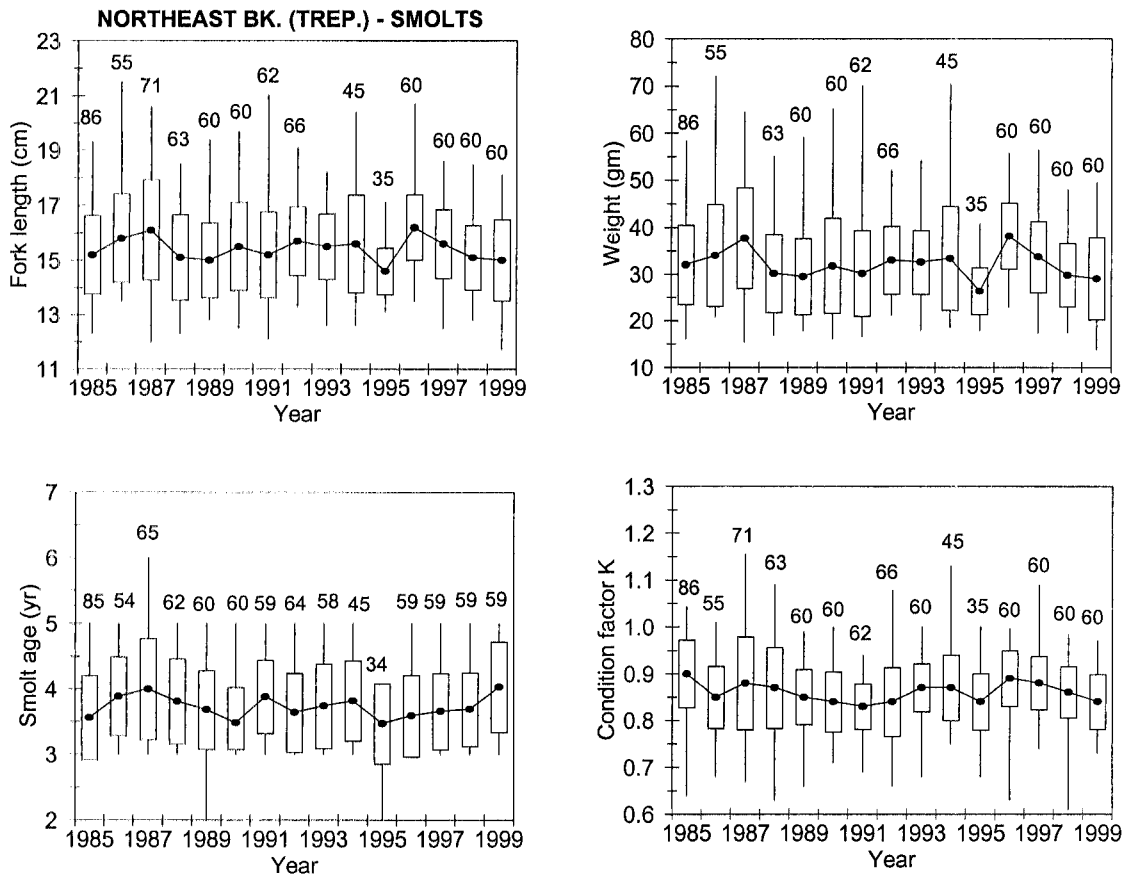
Fig. 28. Mean fork length, mean weight, mean smolt age, and mean condition factor for smolts from Northeast Brook, Trepassey, 1985-99. The rectangle around each point denotes the standard deviation; the vertical line is the range; the number above the vertical line is the sample size.
