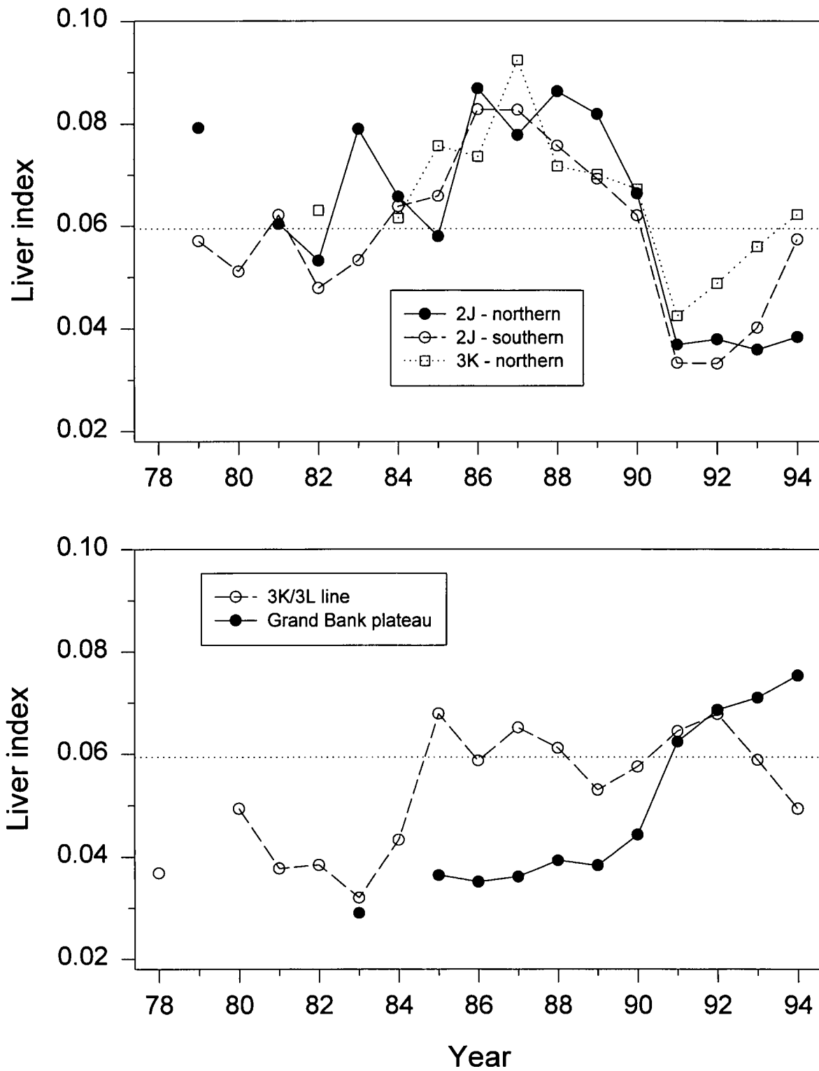
Fig. 4. Annual variability in mean liver index for cod 45-62 cm caught in five regions of Divisions 2J3KL during assessment surveys in the autumns of 1978-1994.
