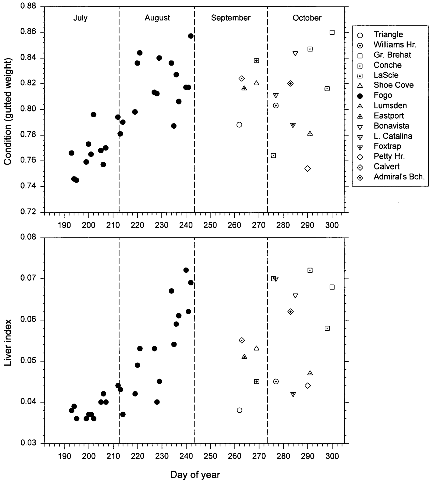
Fig. 5. Condition of cod sampled during the sentinel survey in Division 2J3KL in 1995. The data are aggregated by community and day of year. Any influence of fish size has been ignored. All samples collected from communities on Fogo Island on a specific day are aggregated. In the legend, communities are ordered from north (top) to south.
