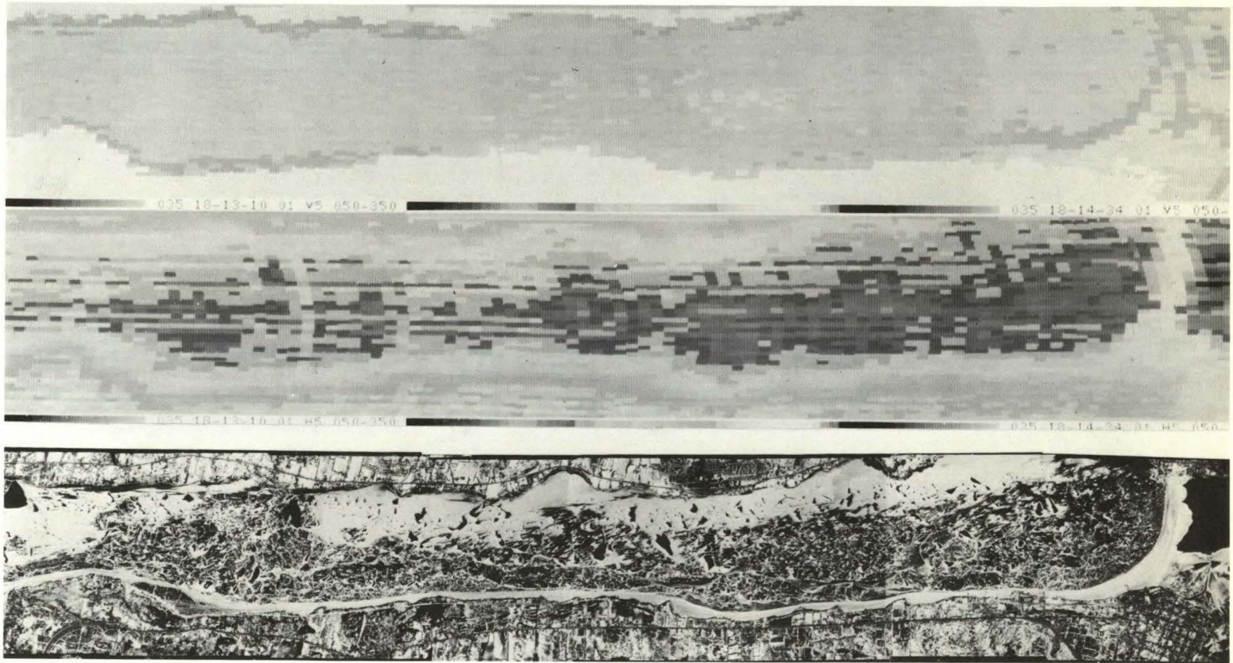
30. Photomosaic and PMIS imagery of part of the St. Lawrence River - Morristown to Ogdensburg. This data was obtained along flight line 1 at an altitude of 2225 m on February 4, 1974.
