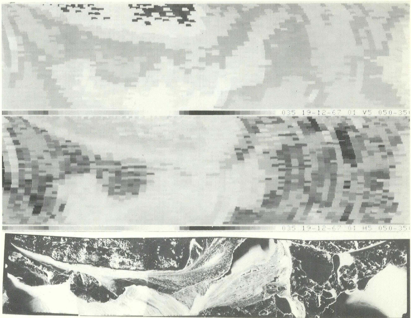
33. Photomosaic and PMIS imagery along line 4 north of Carleton Island, taken at an altitude of 700 m.
