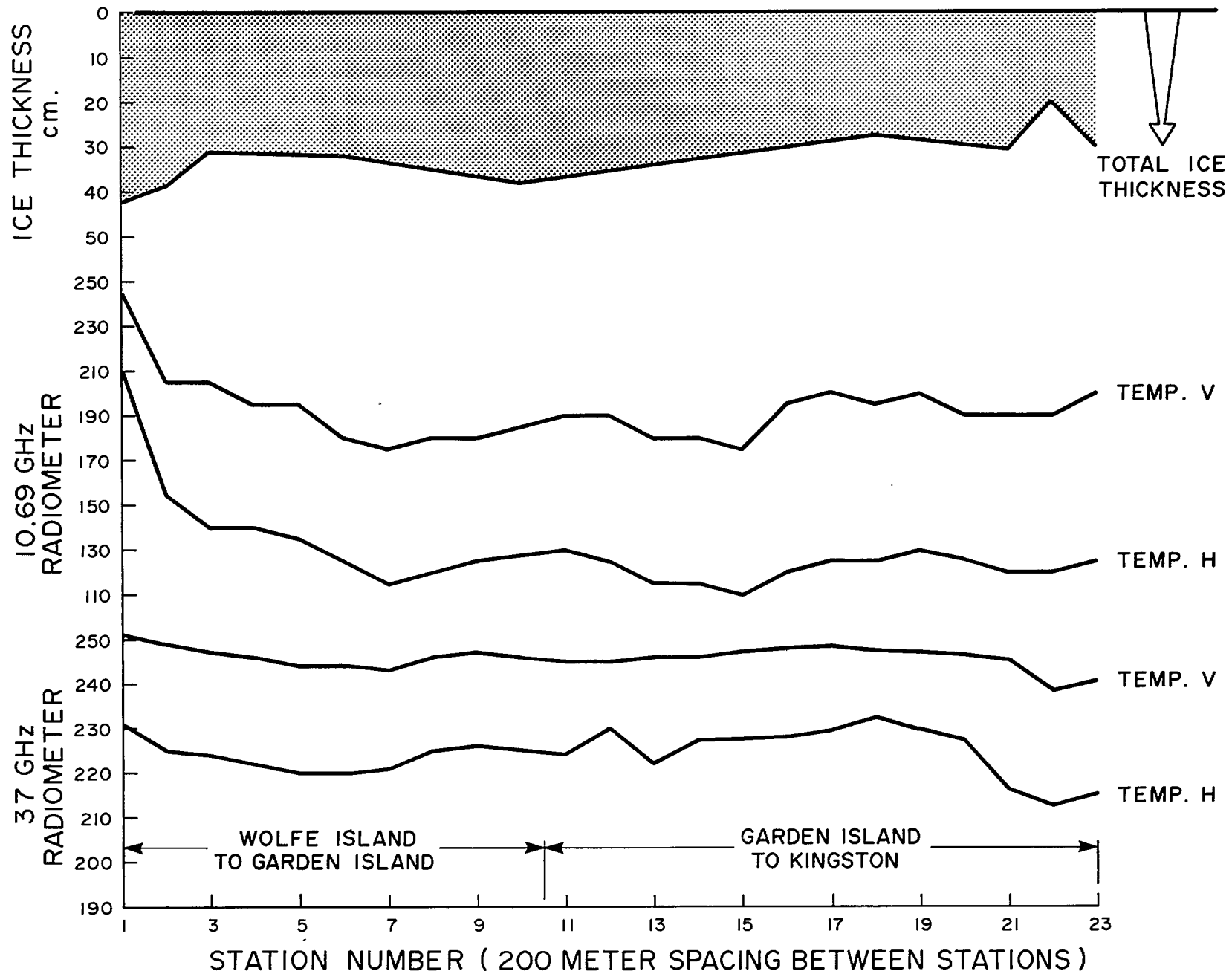
36. Ice thickness and brightness temperature profiles for 10.69 GHz and 37 GHz PMIS and Aerojet passive microwave radiometer respectively. These profile correspond to flight line 6.
