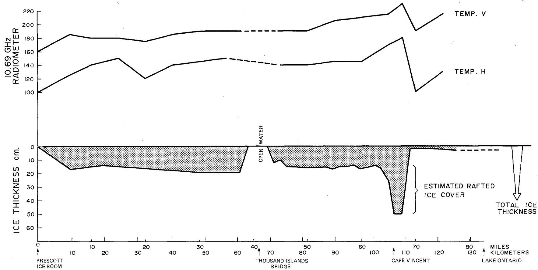
31. Ice thickness and PMIS brightness temperature profile along flight line 1.
