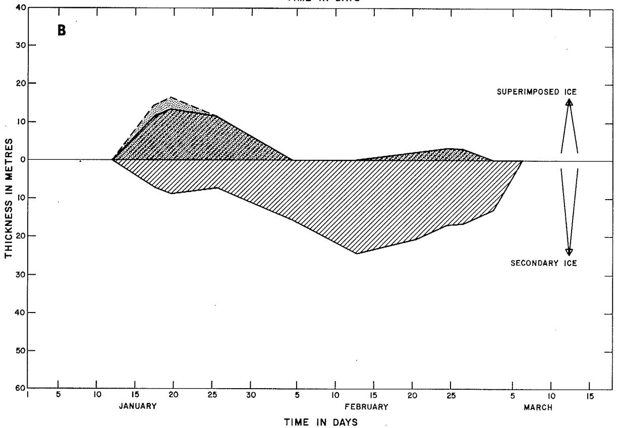
28. Ice thickness station profiles showing the thickness due to secondary and superimposed ice. A) Station H-3 9.65 km; B) Station 6 78.8 km; C) Station 12 99.7 km and D) Station 17 102.2 km from Prescott-Ogdensburg.
