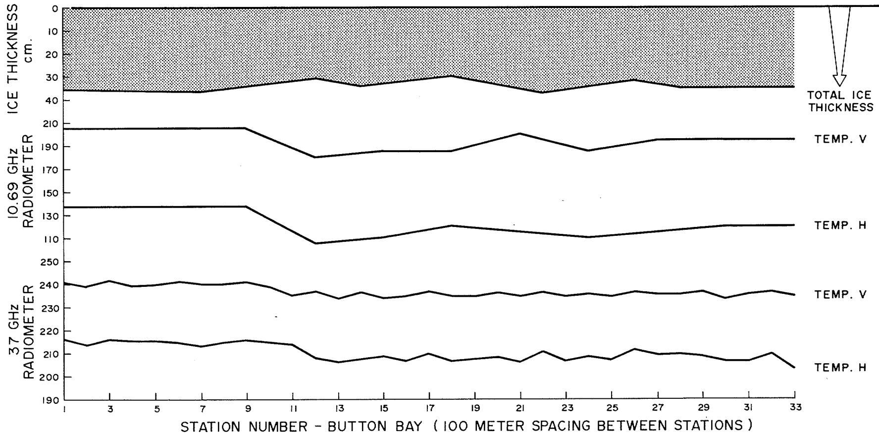
35. Ice thickness and brightness temperature profiles for 10.69 GHz and 37 GHz. PMIS and Aerojet passive microwave radiometers respectively. This area corresponds to the shorefast and black ice area in Figure 34.
